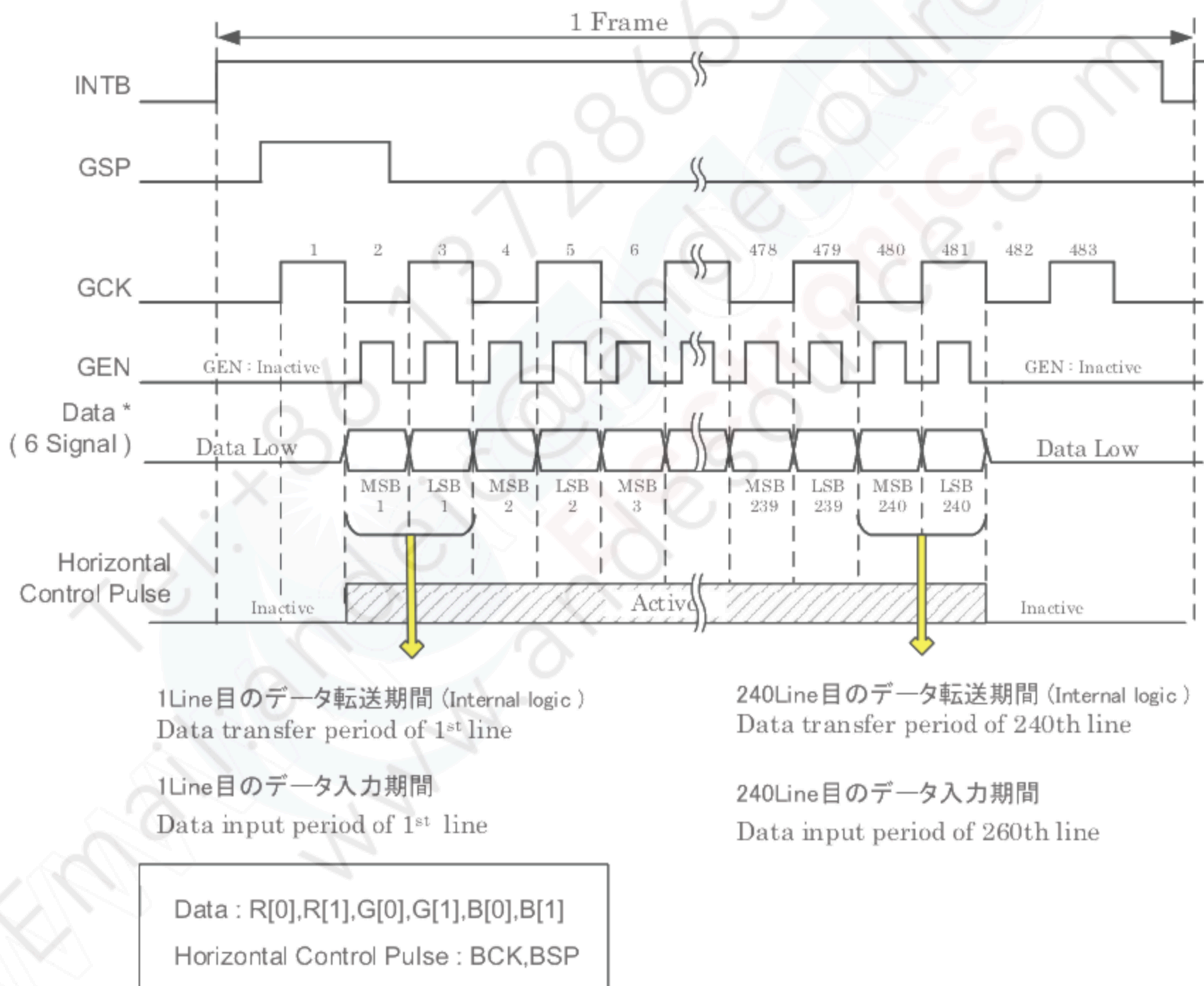
Figure 6-5-1 Vertical Diagram
