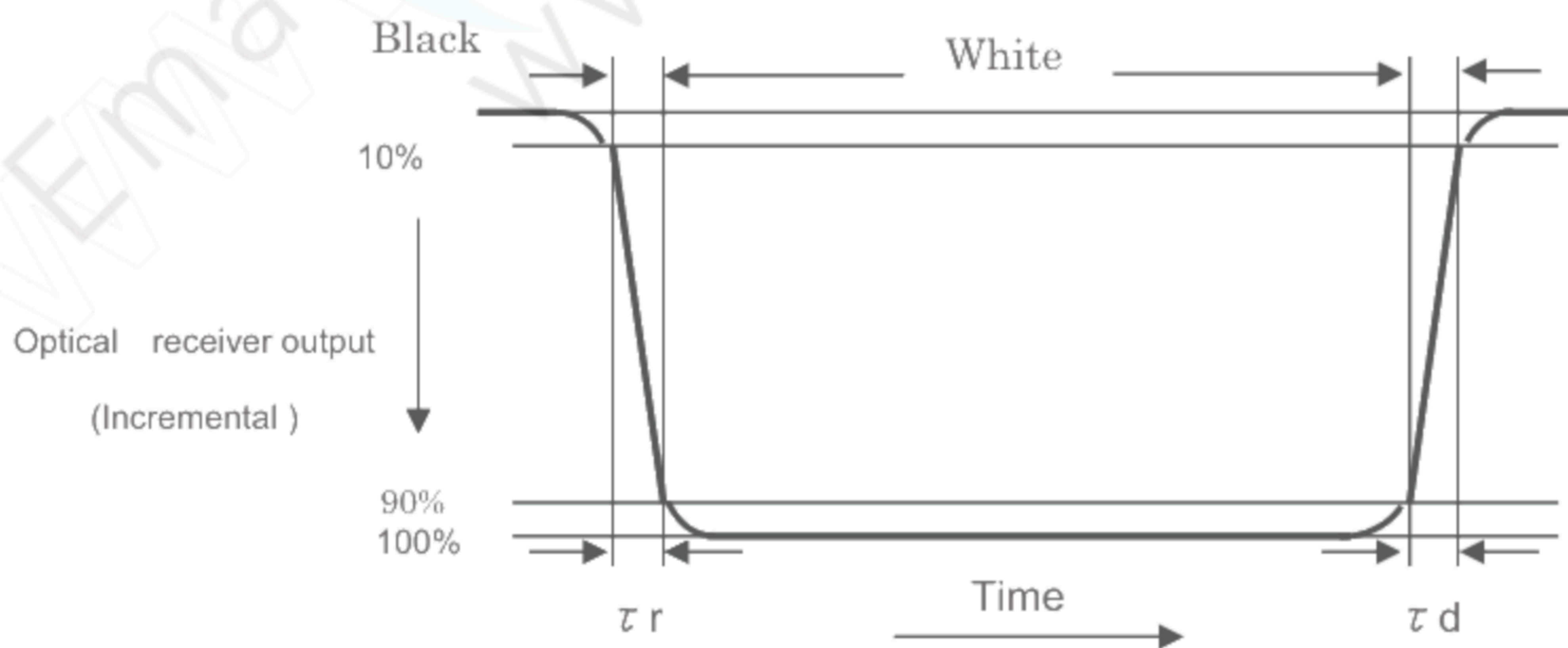
Figure 7-4 Respons time
