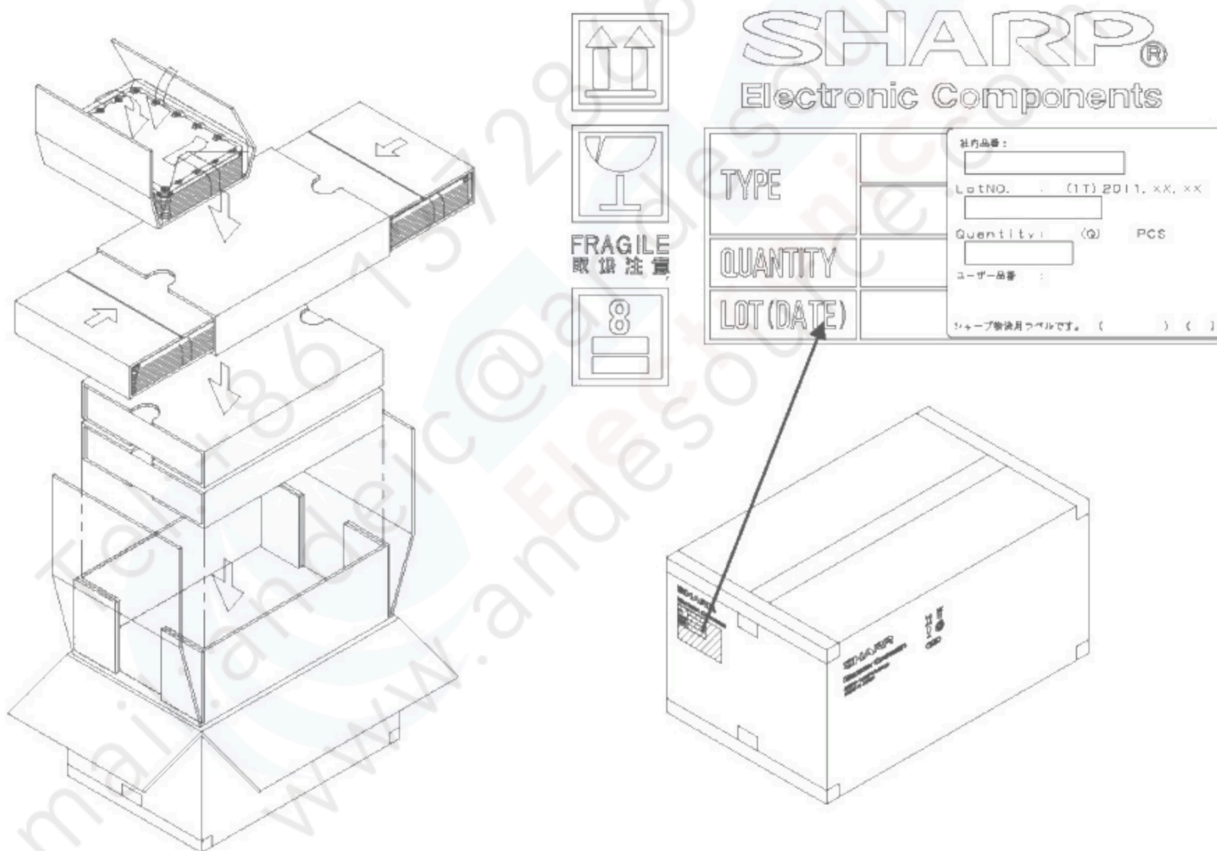
Figure. 12-1 Packaging Form
