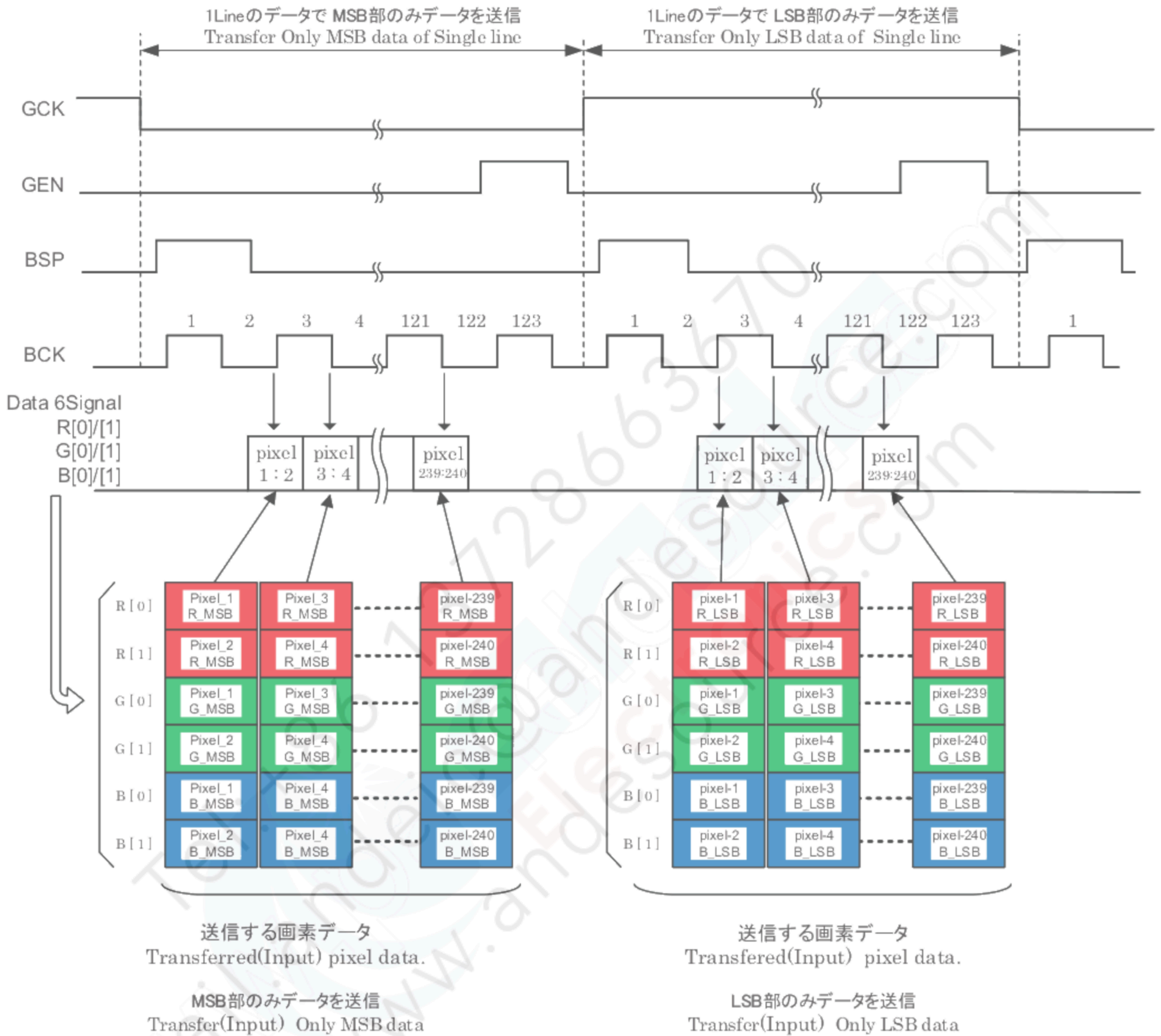
Figure 6-5-2 Horizontal Diagram
