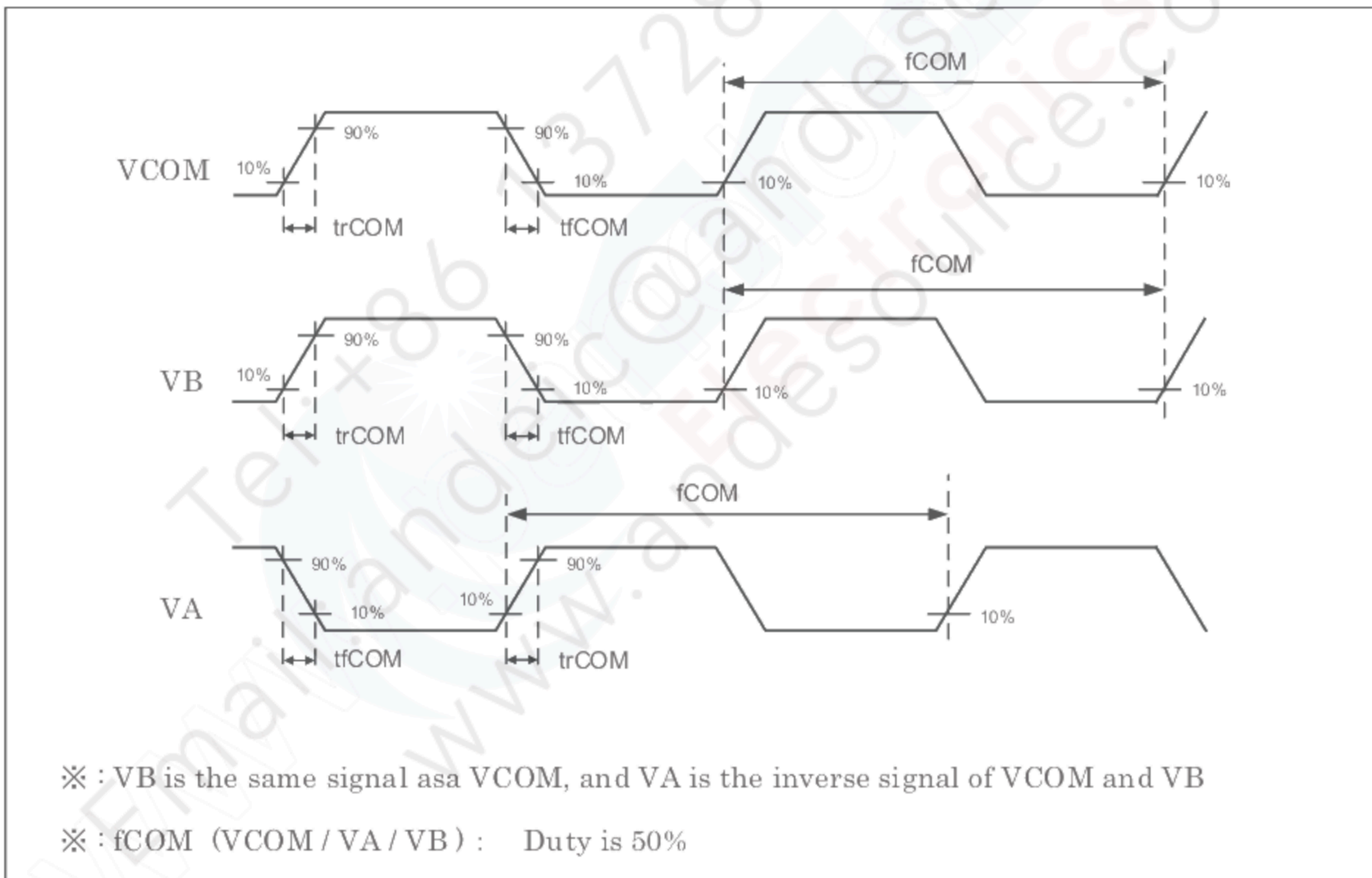
Figure 6-3-2 AC timing 2
