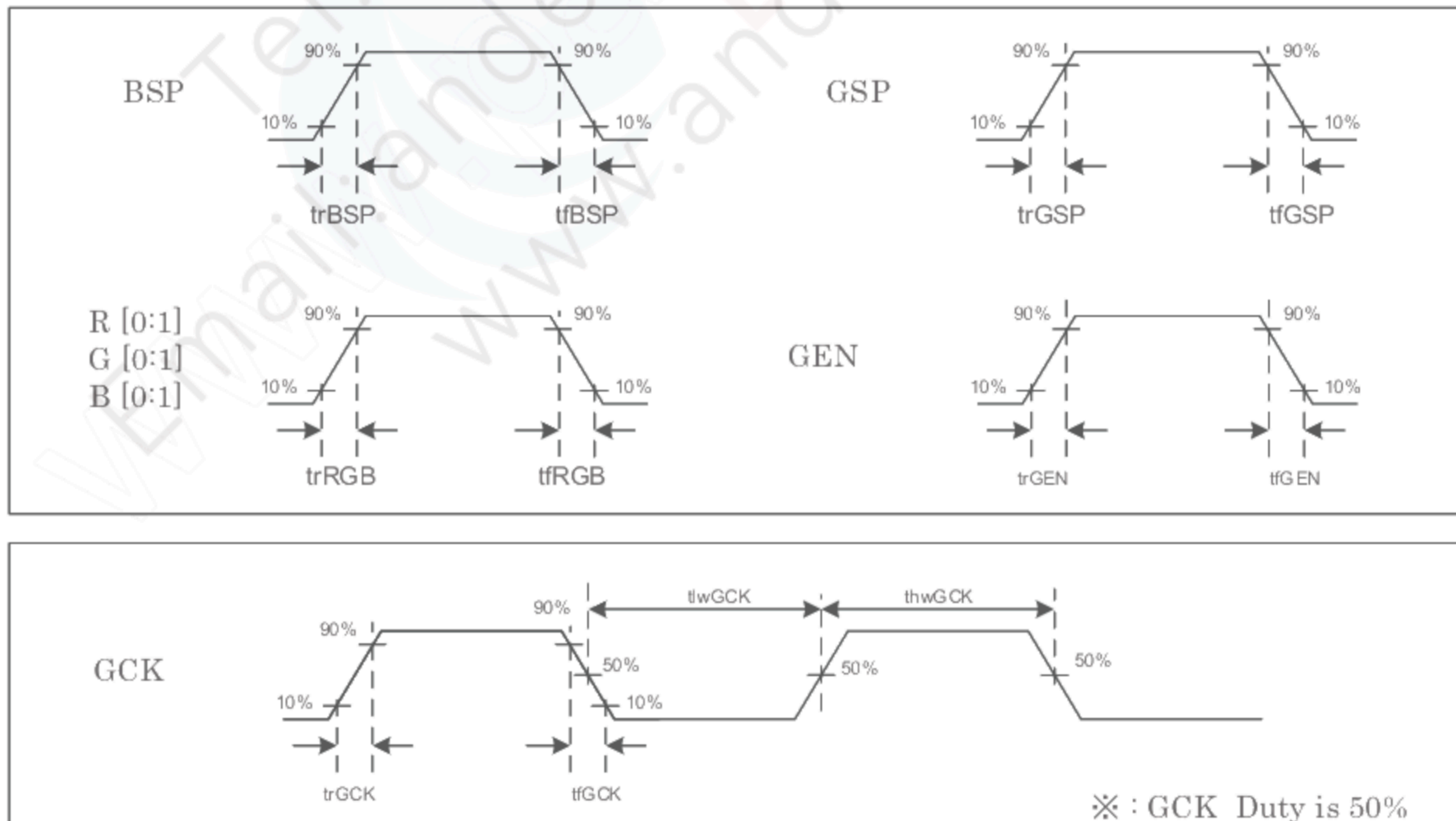
Figure 6-3-1 AC timing 1
