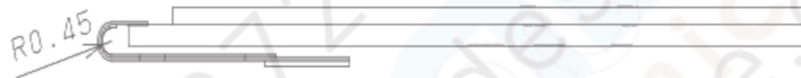
Figure 8-2 FPC Bend Specification
