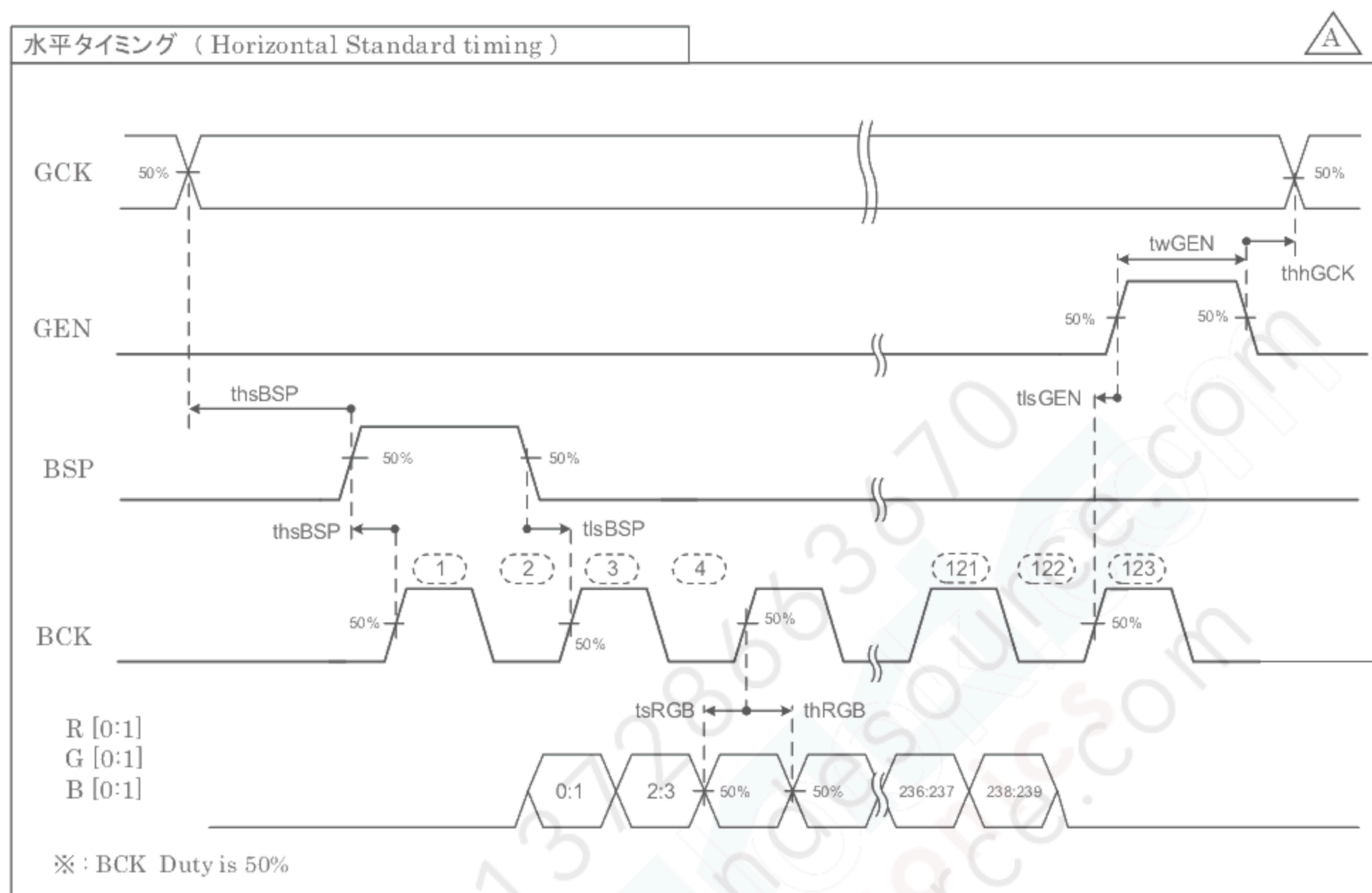
Figure 6-3-2 AC timing 2
