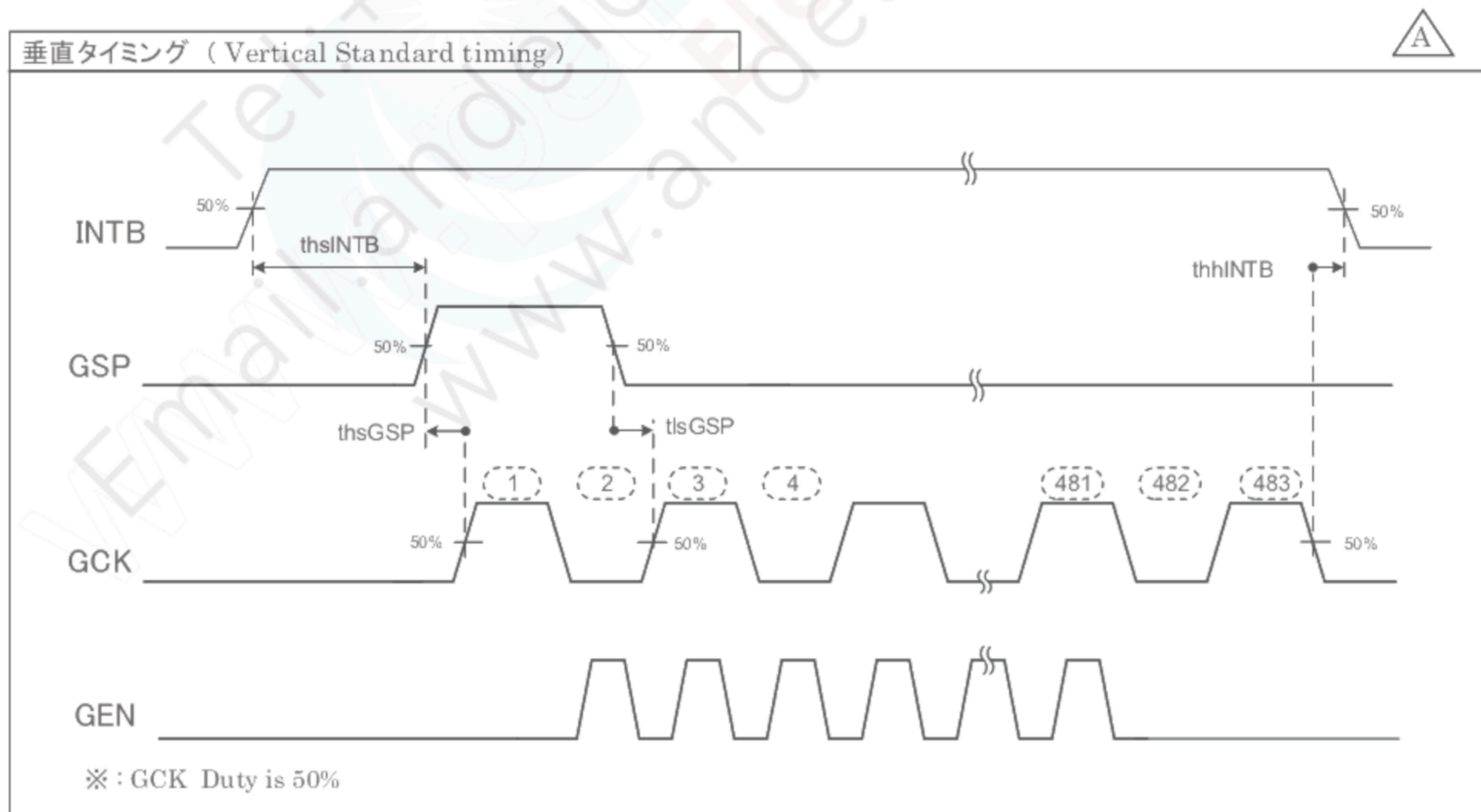
Figure 6-3-3 AC timing (type-5)
