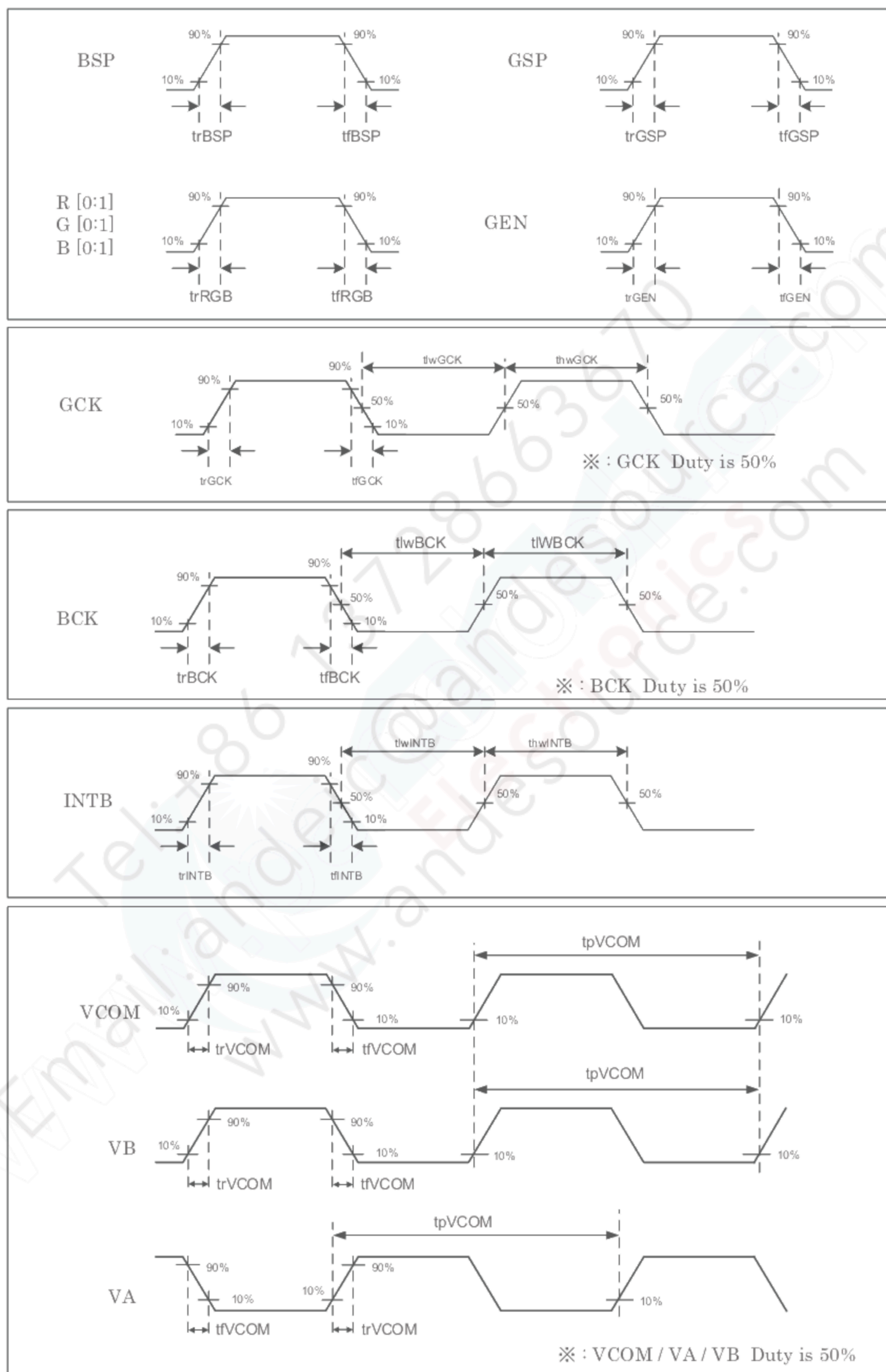
Figure 6-3-1 AC timing 1
