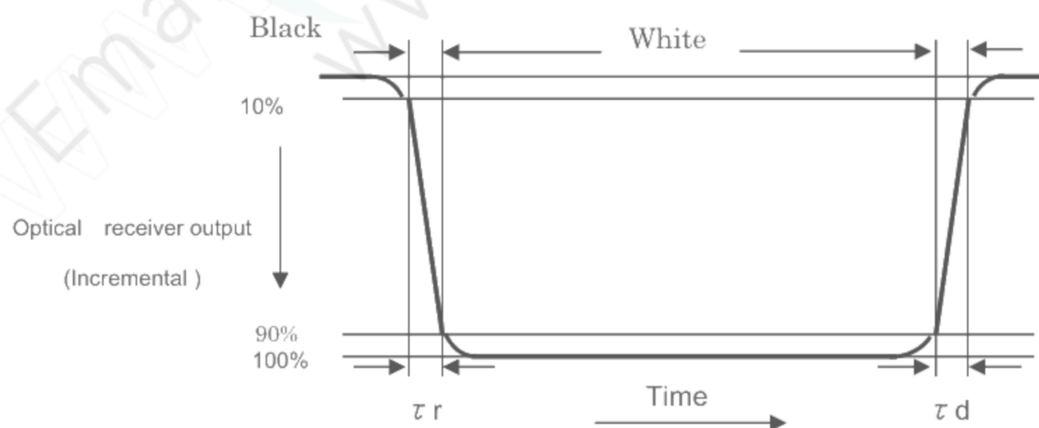
Figure 7-4 Respons time
