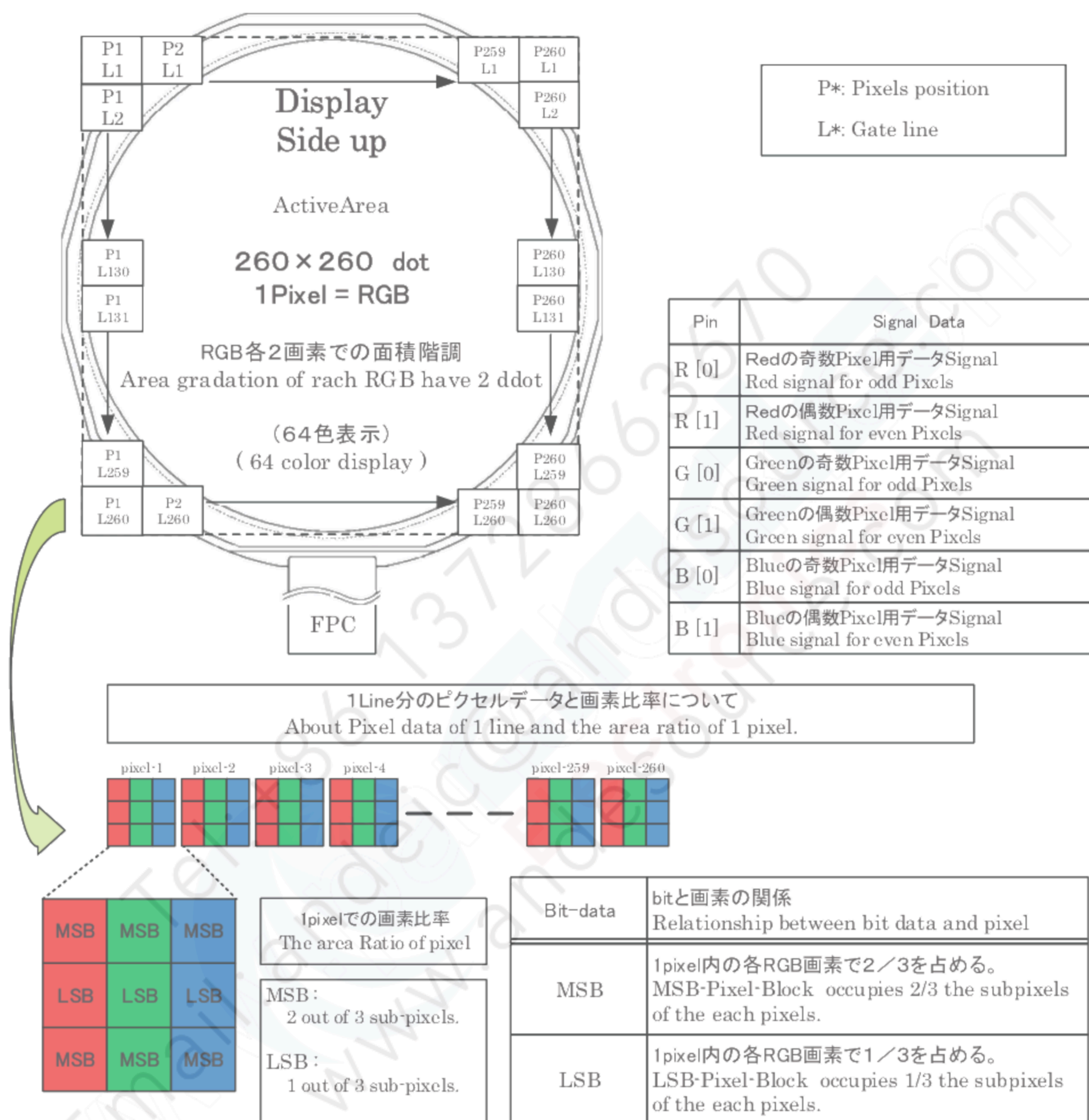
Figure 6-6-1 Data position 1
