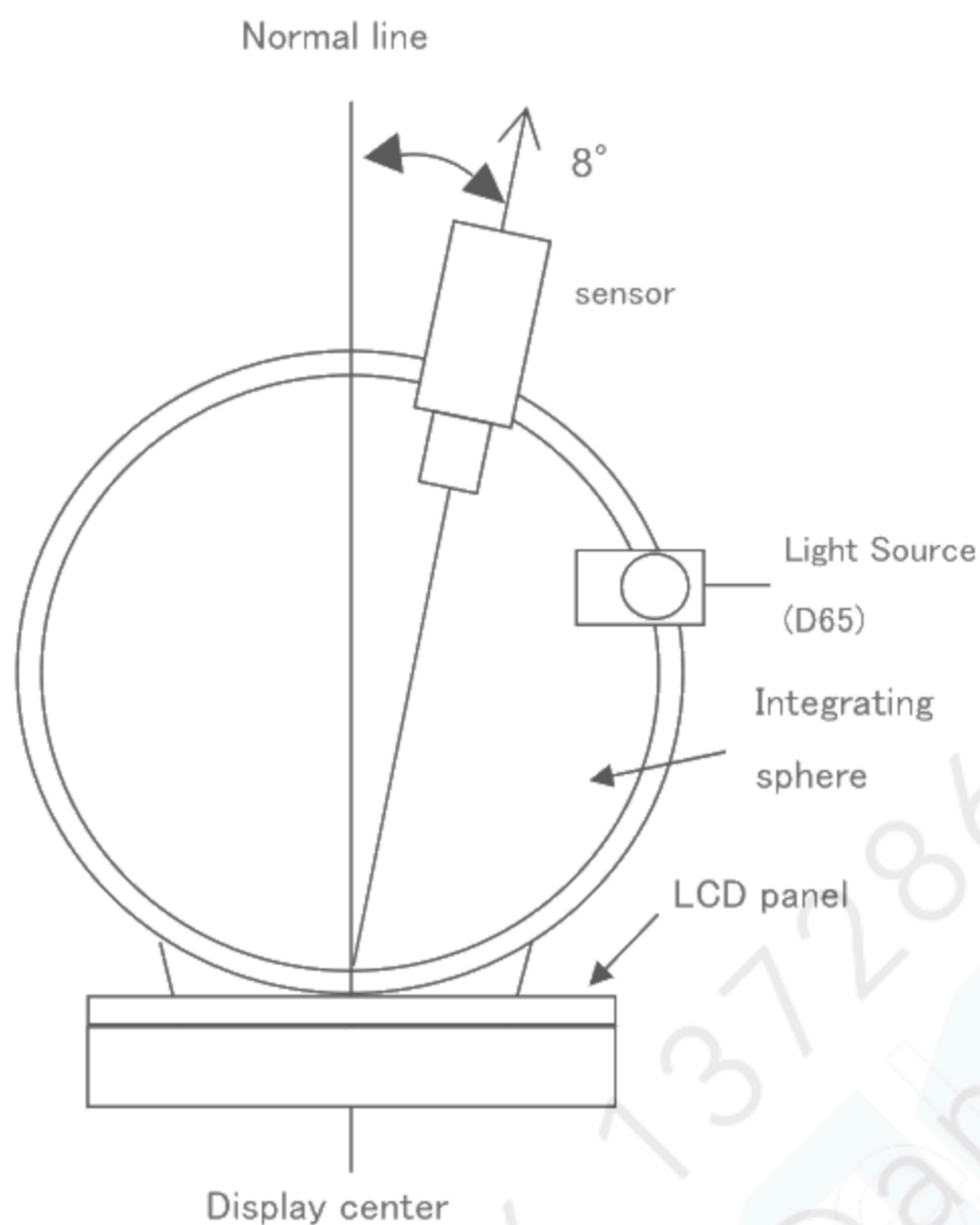
Figure 7-2 Contrast ratio, Reflection ratio, Panel chromaticity
