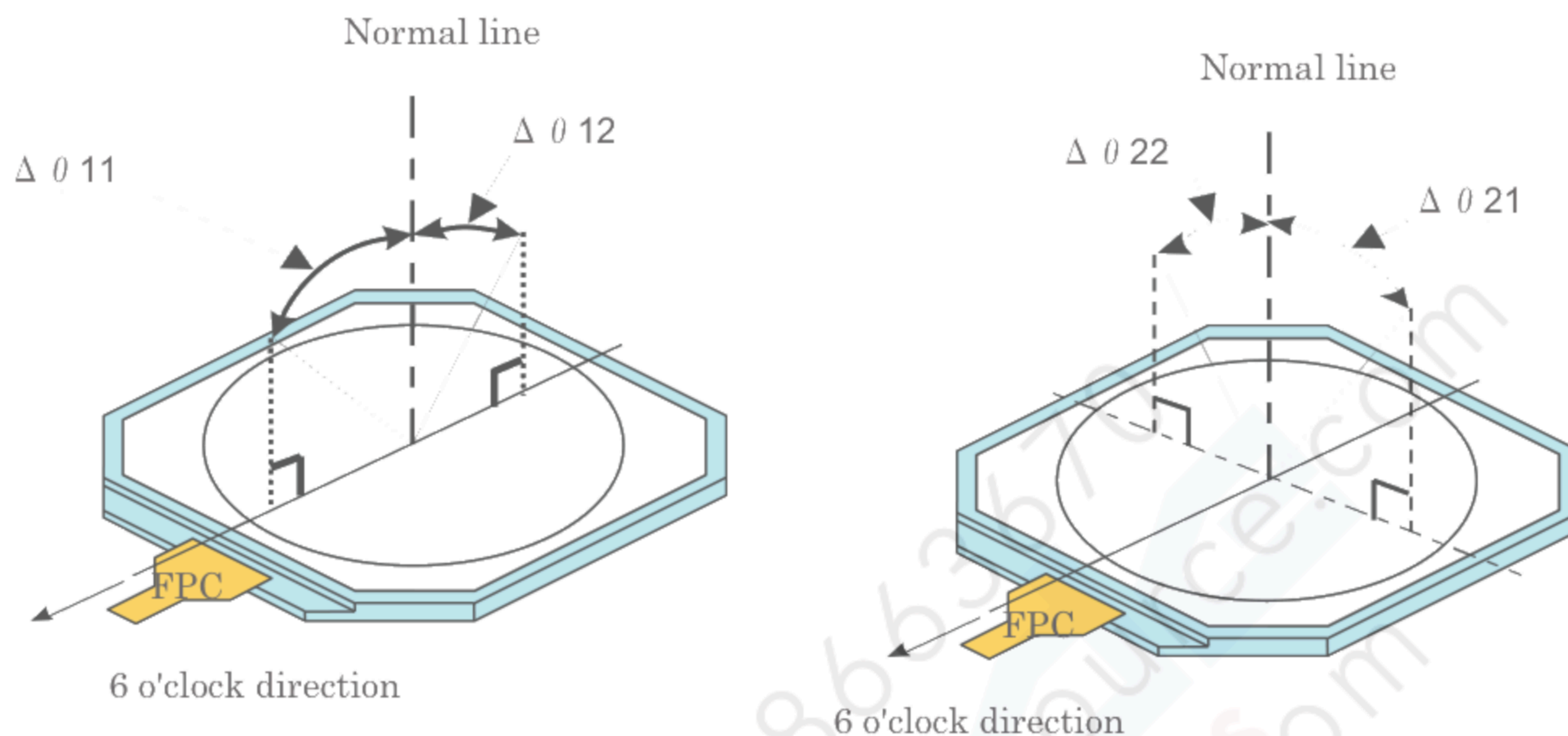
Figure 7-1 Defintion of Viewing Angle
