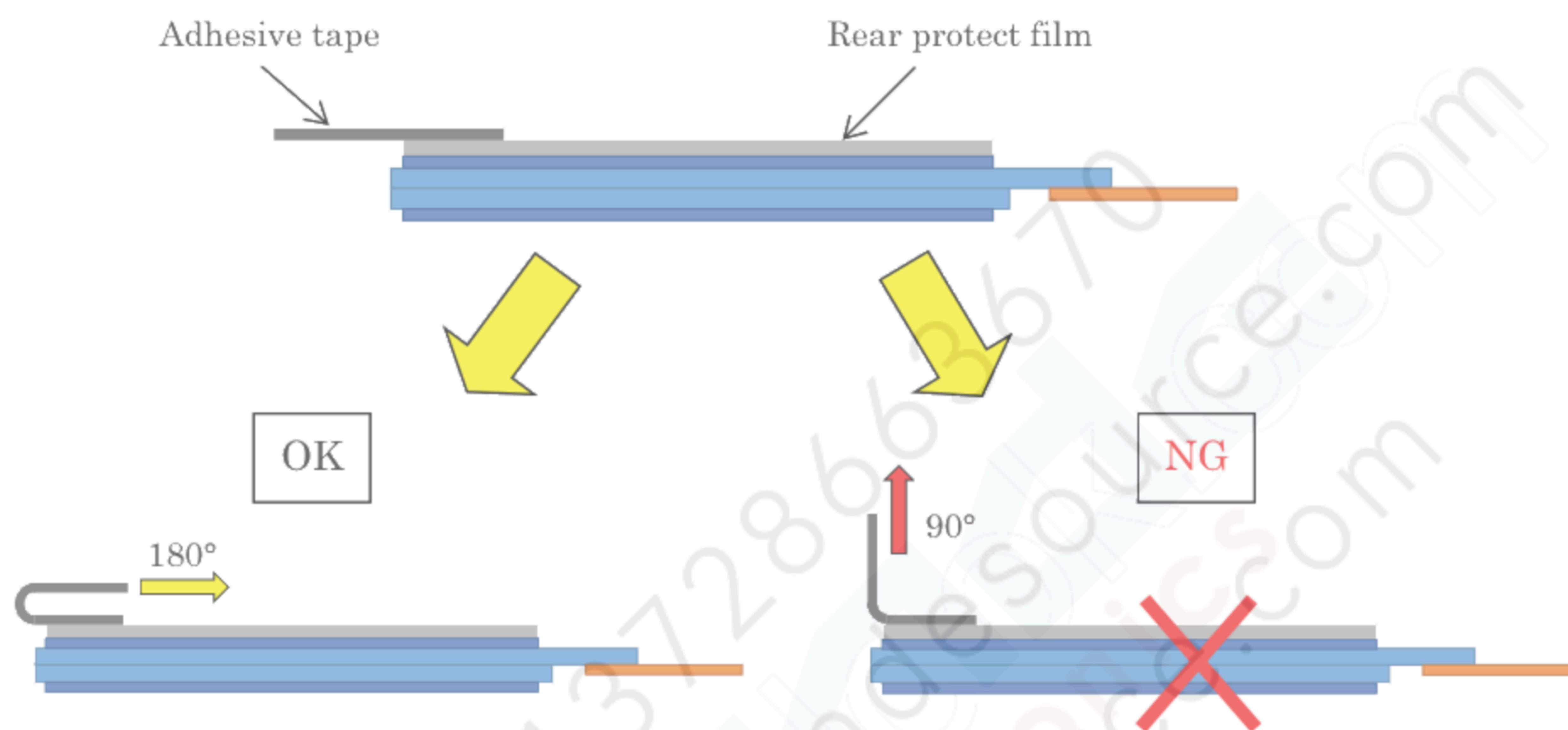
Figure POL-2 Peel angle
