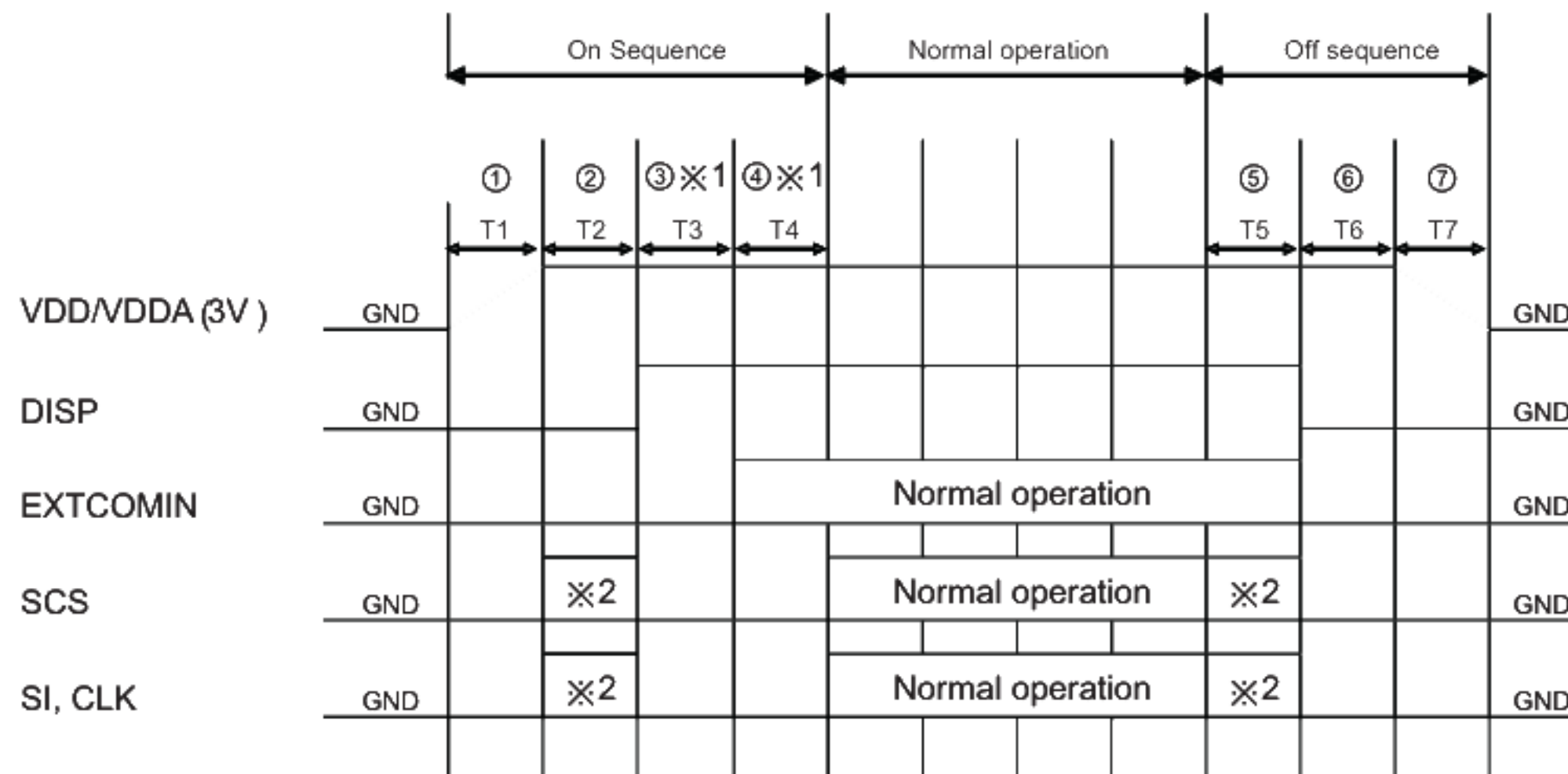
Figure 6-1 Power source sequence
