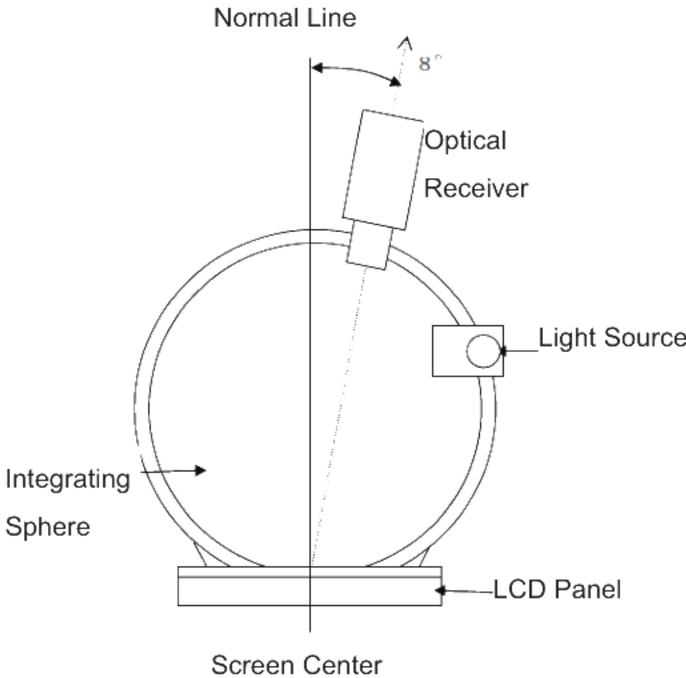
Measurement Equipment (CM-2002)
