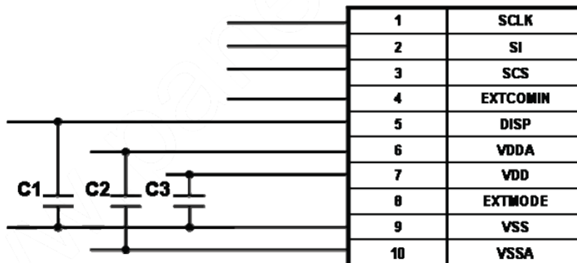
Figure 9-1 External circuit diagram (recommended)
