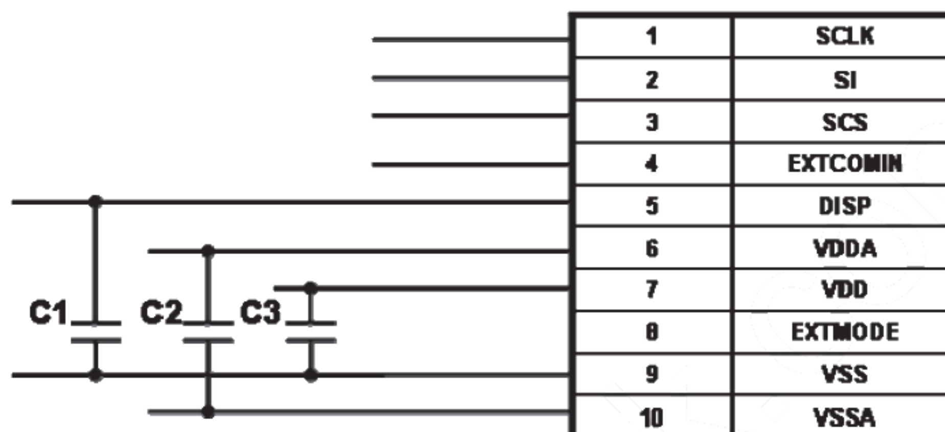
Fig. 9-1 External capacitor recommendation capacity value
