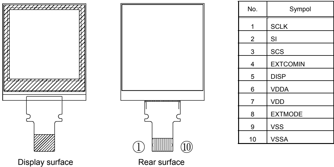
Figure 8-2 Module outline
