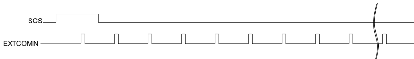
Figure 6-3 EXTCOMIN Signal 2
