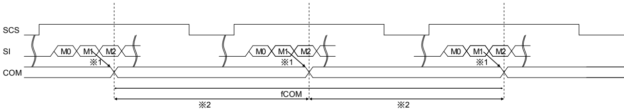
Figure 6-10 COM Inversion (EXTMODE=Lo)
