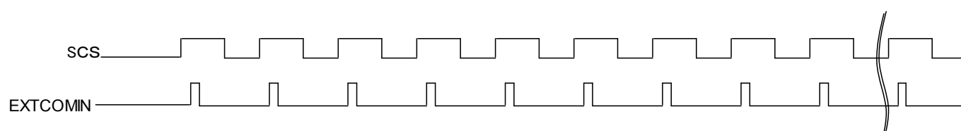
Figure 6-2 EXTCOMIN Signal 1
