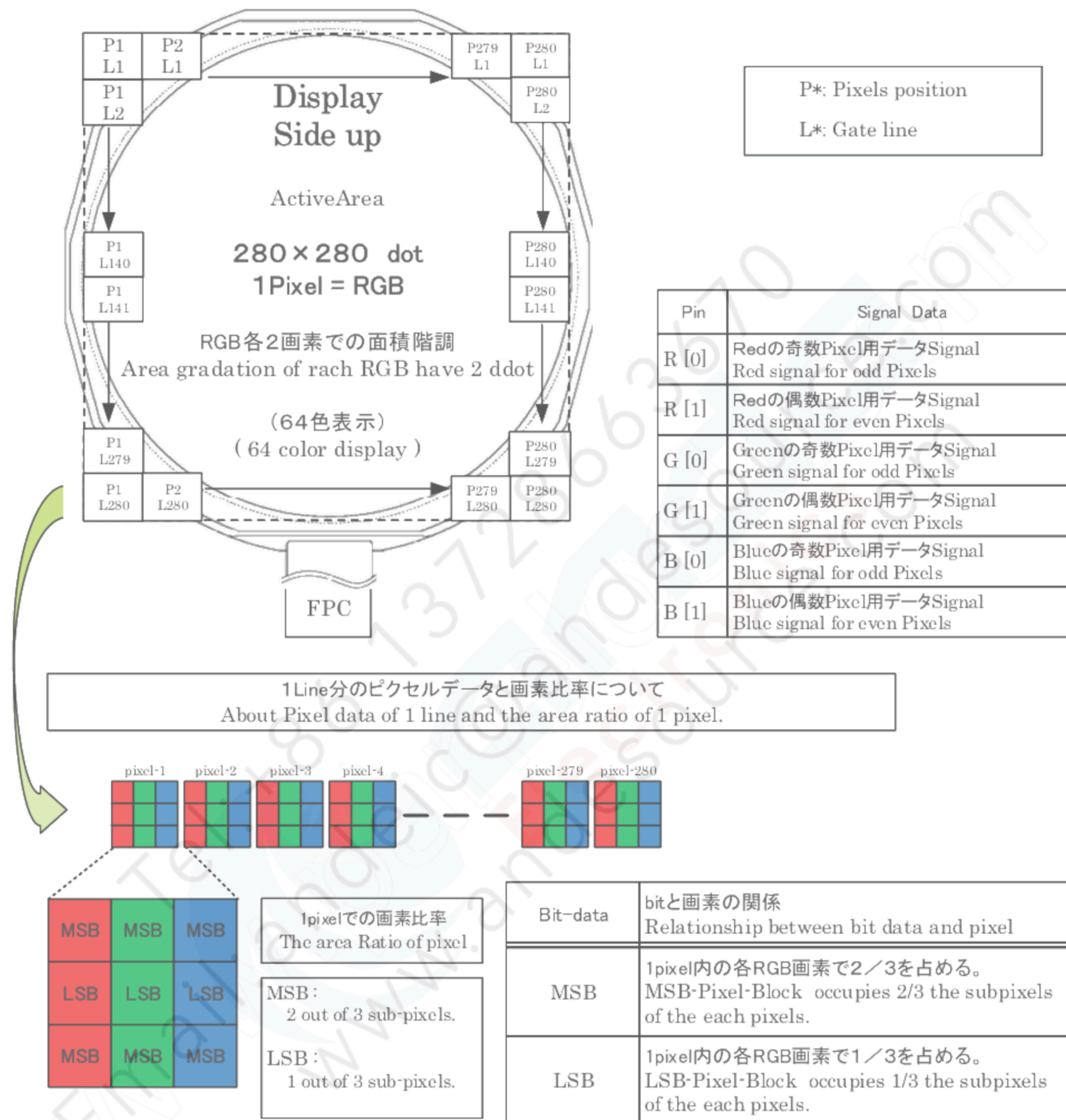
Figure 6-6-1 Data position 1
