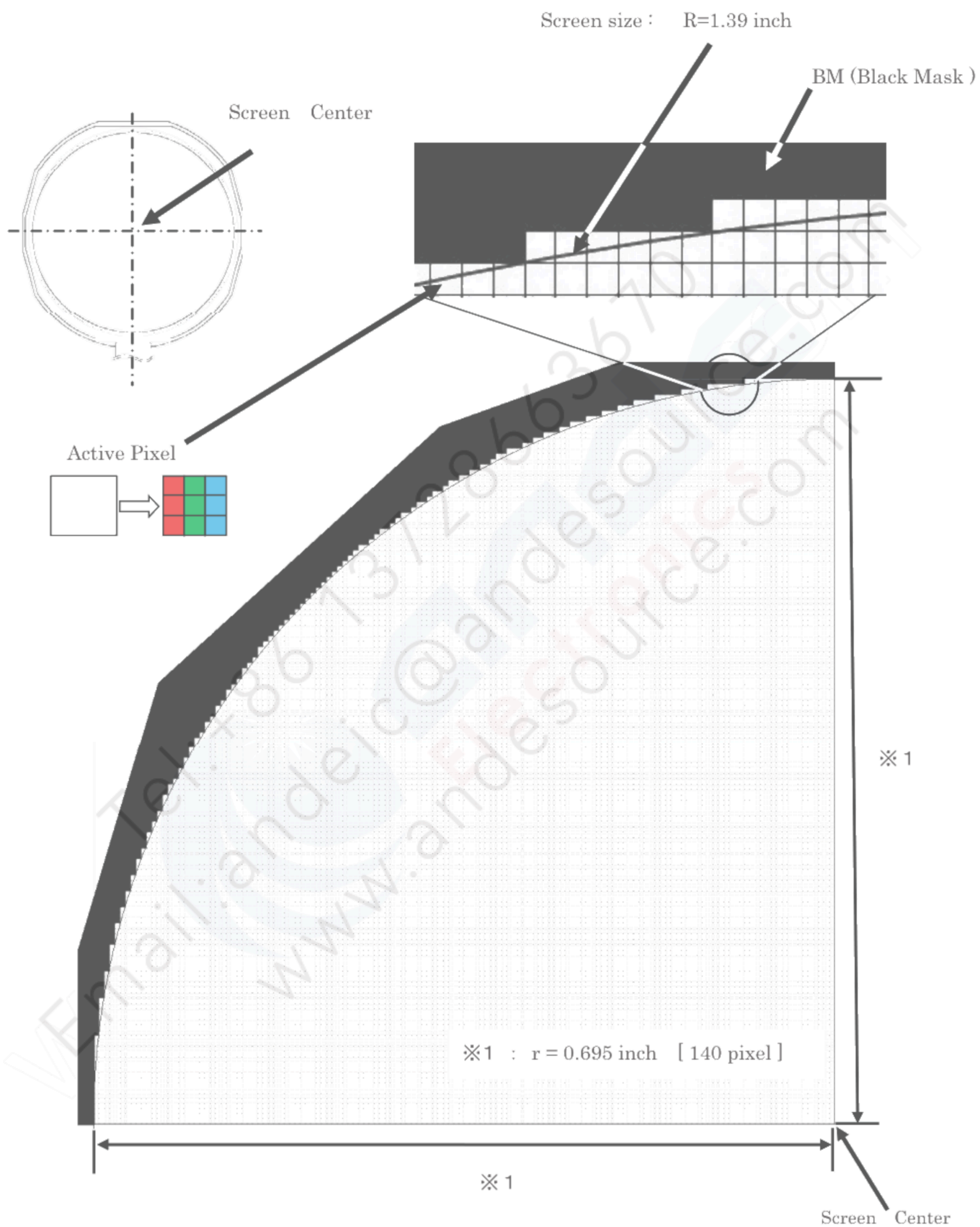
Figure 6-6-2 Data position 2
