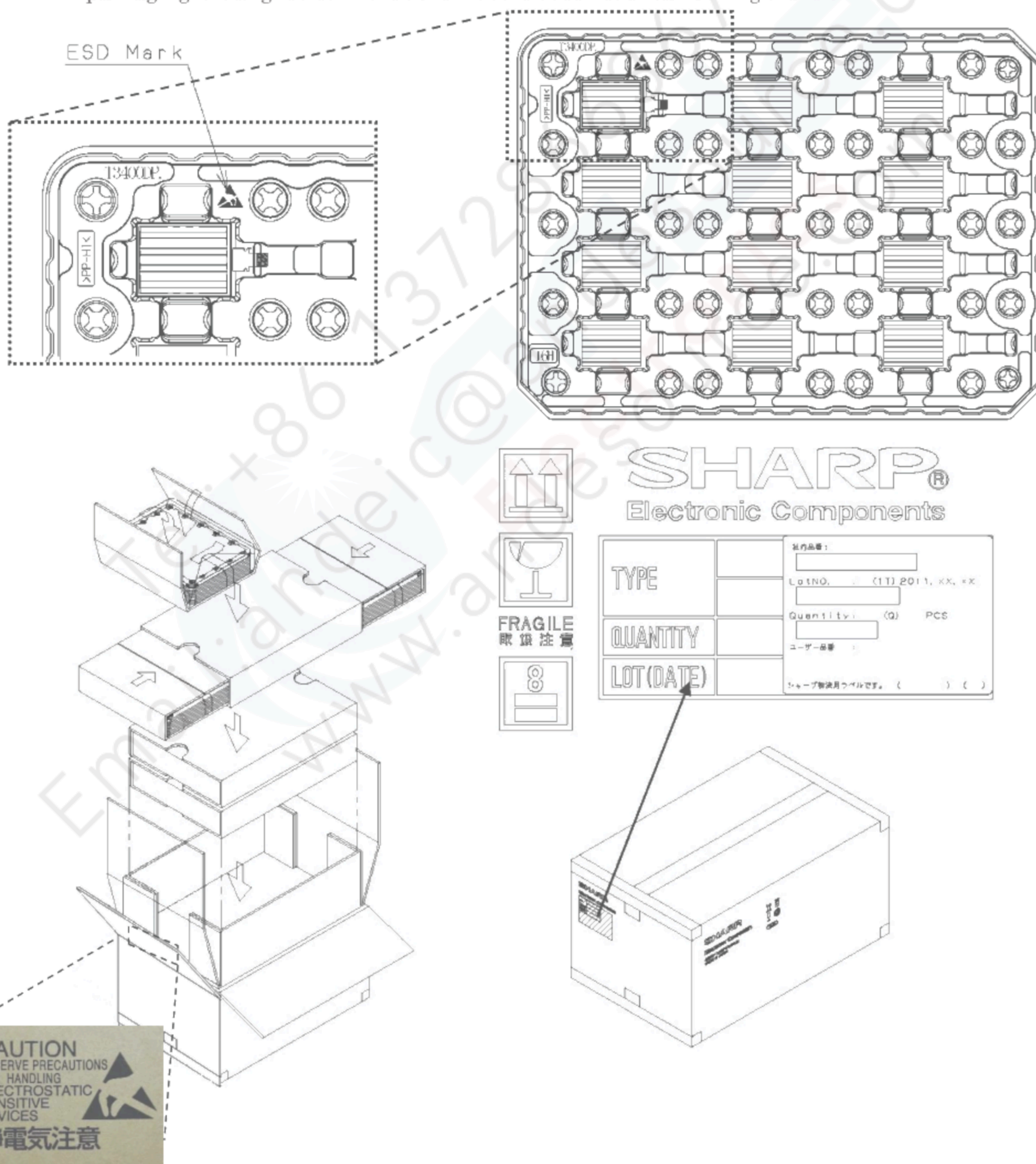
Figure. 12-1 Packaging Form
