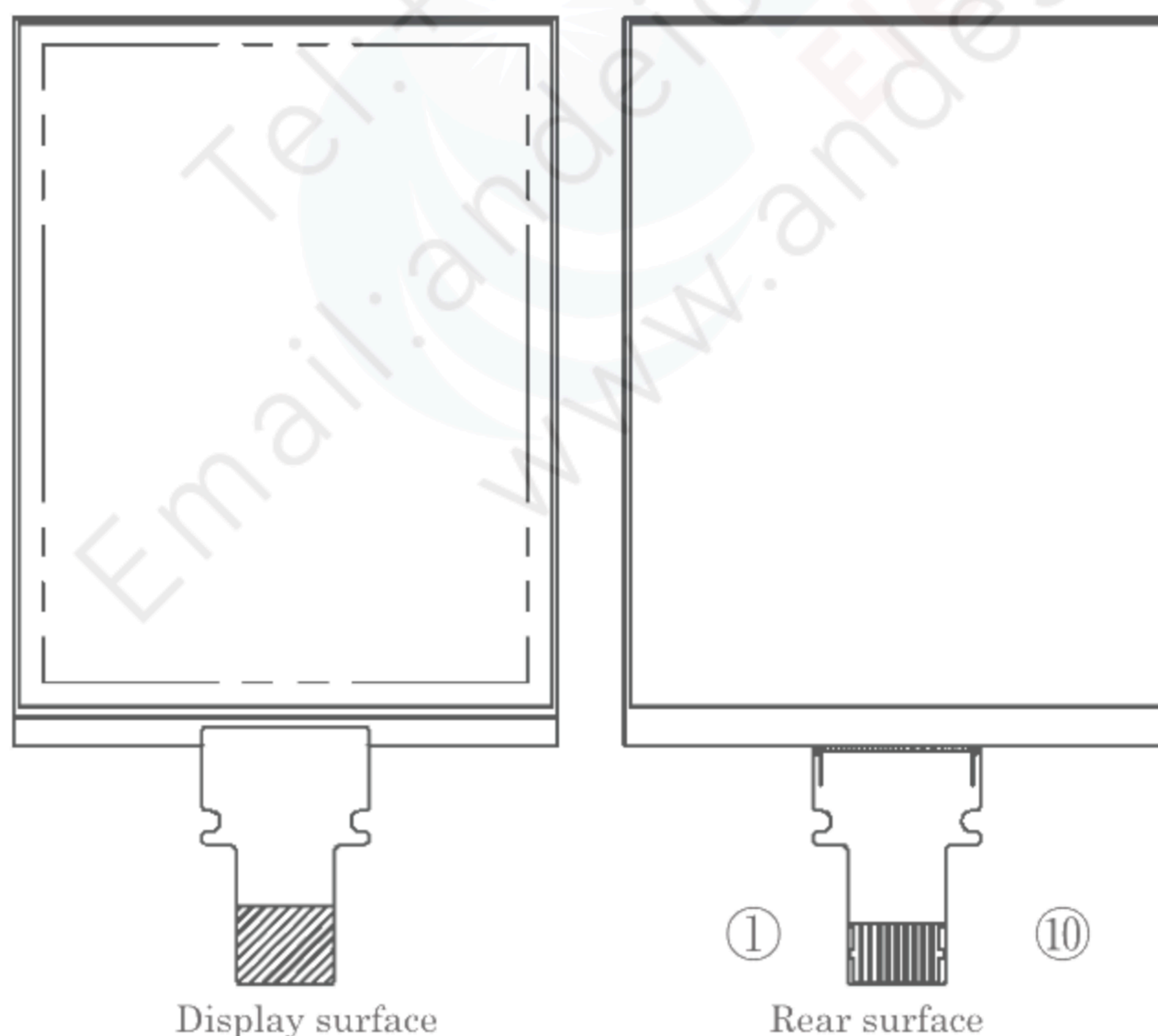
Figure 8-1 Module outline
