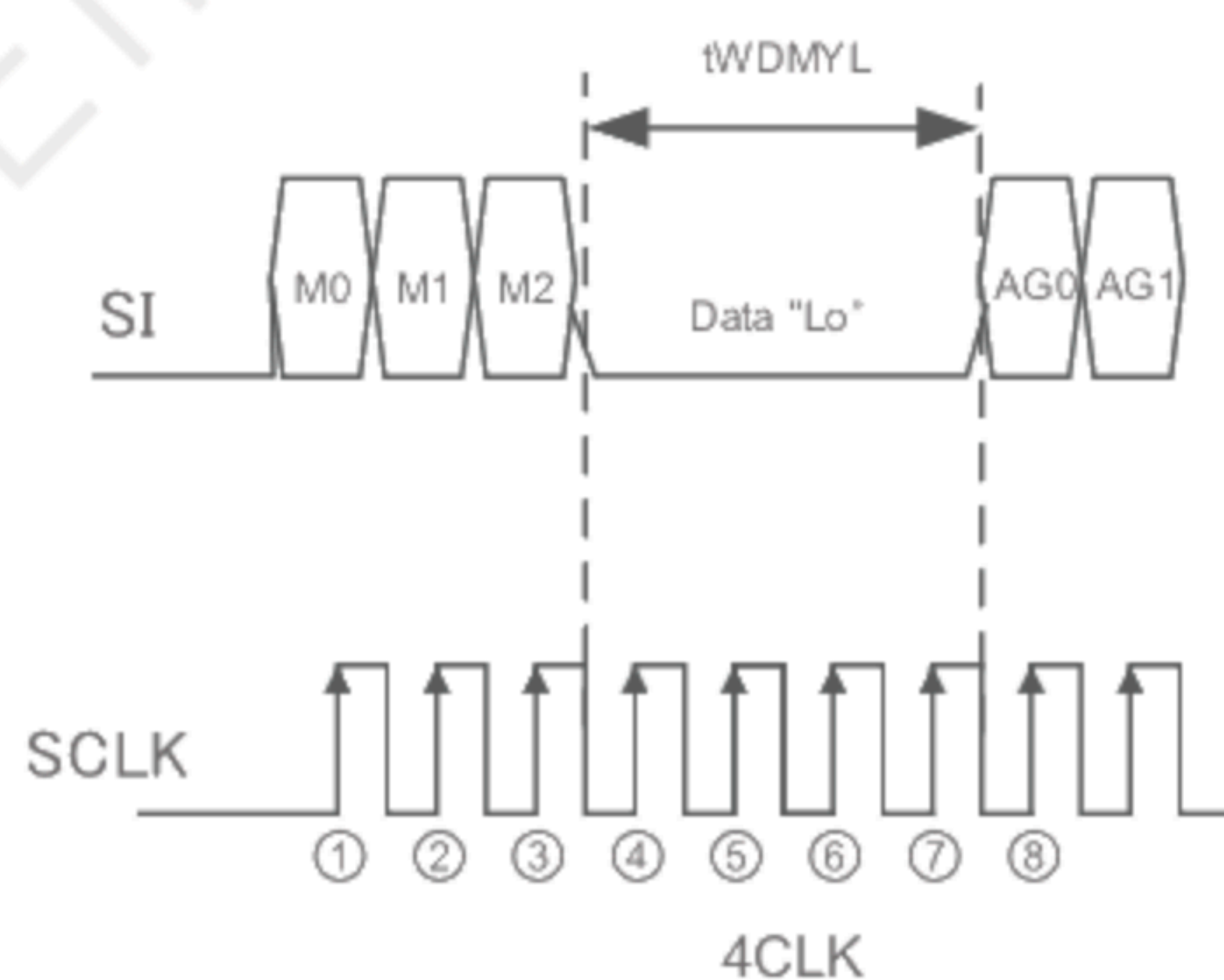
Figure 6-3-2 Signal Timing-2
