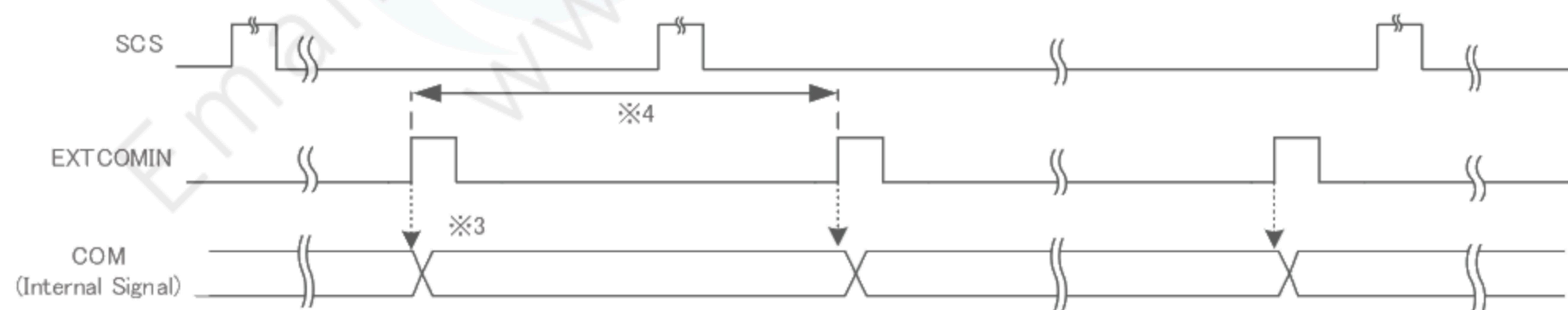
Figure 6-11 COM Inversion (EXTMODE=Hi)2
