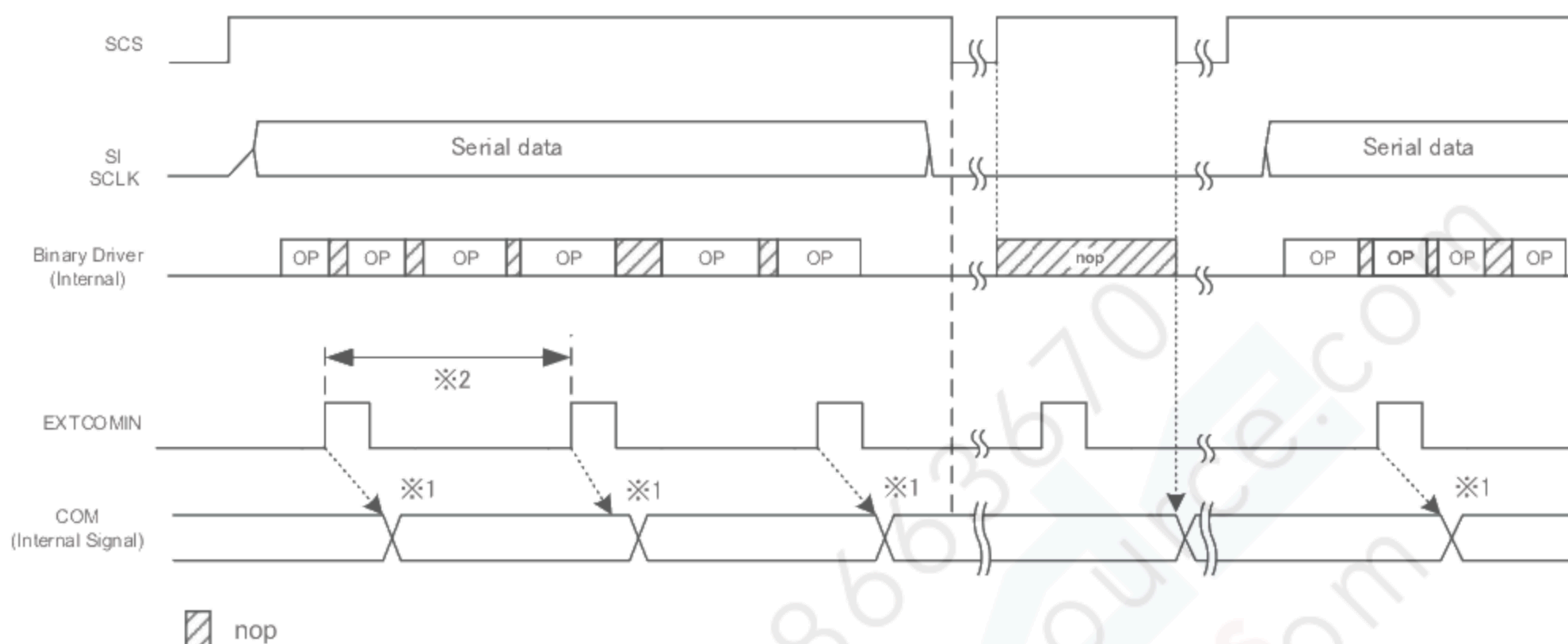
Figure 6-10 COM Inversion (EXTMODE=Hi) 1
