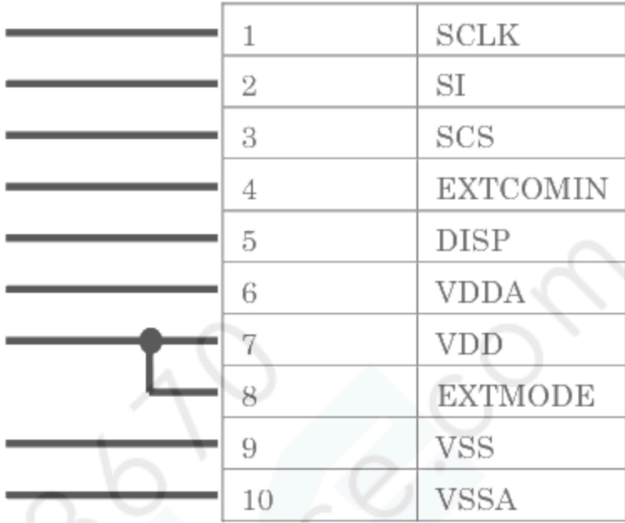
Figure 4-1 Recommended circuit
