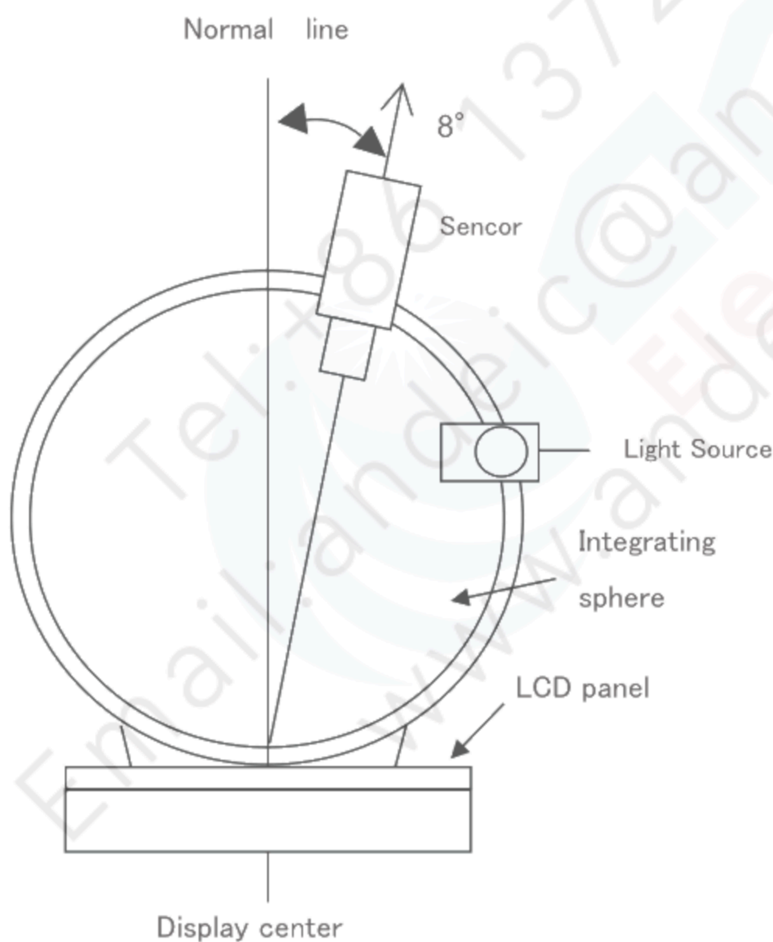
Figure 7-2 Contrast ratio, Reflection ratio, Panel chromaticity
