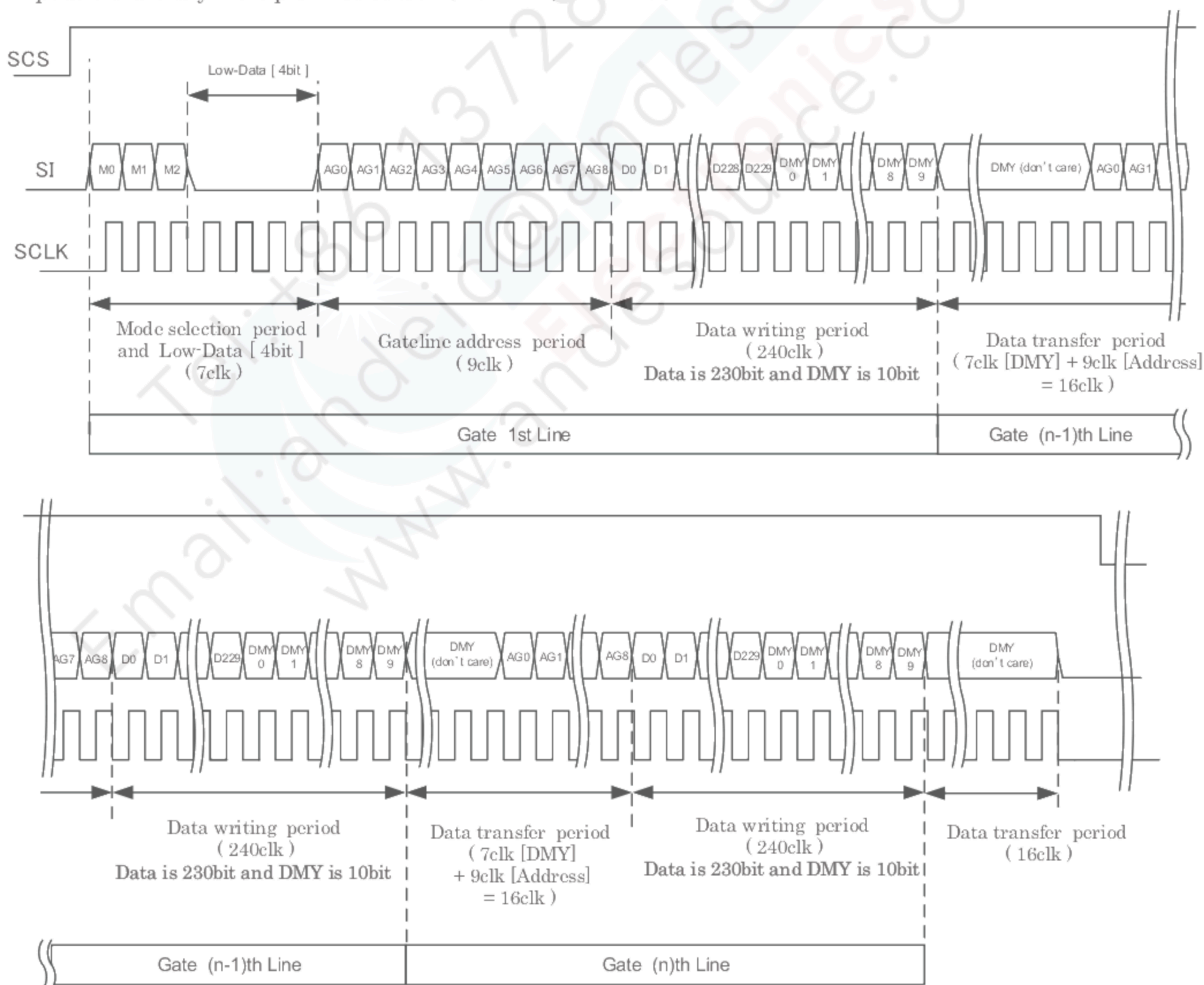
Figure 6-7 Data update mode by Multiple Lines
