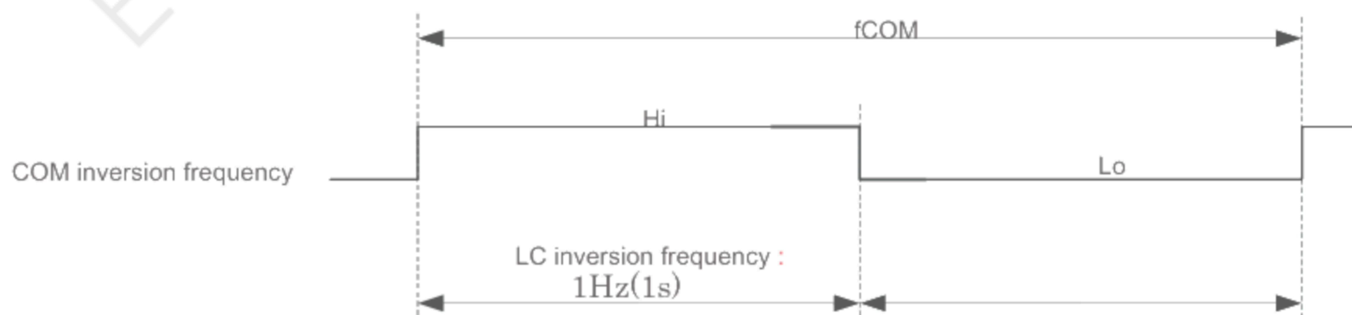
Figure 6-4 COM inversion frequency
