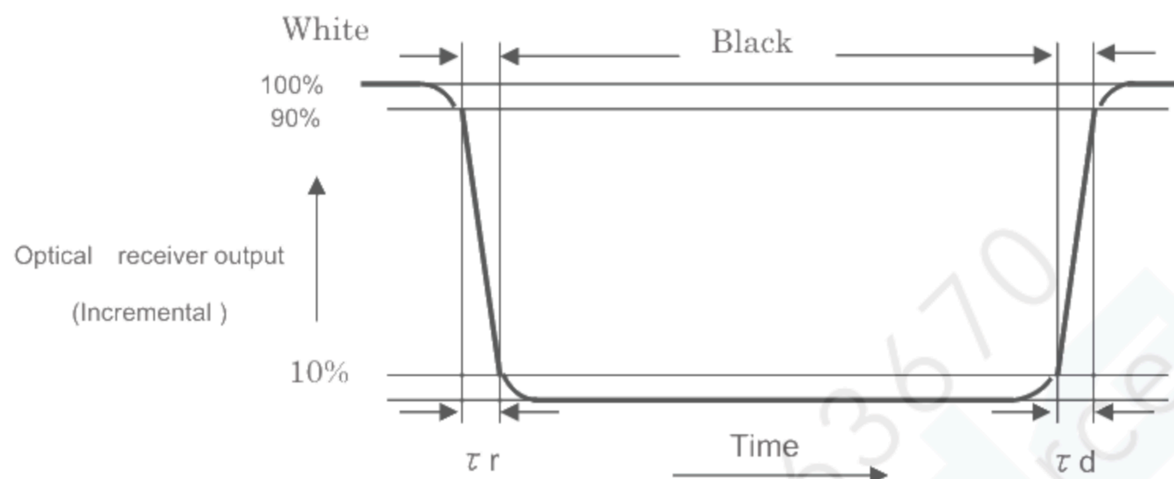
Figure 7-4 Respons time
