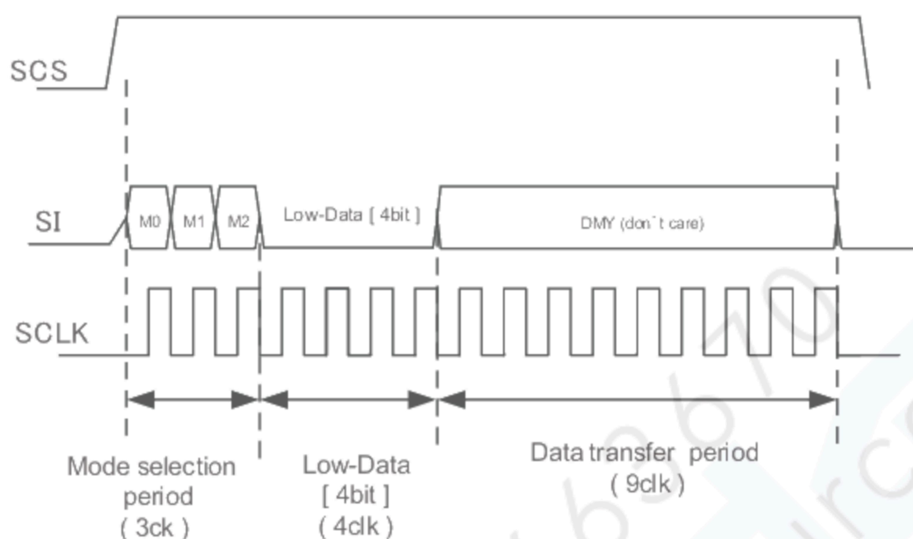
Figure 6-8 All Clear mode
