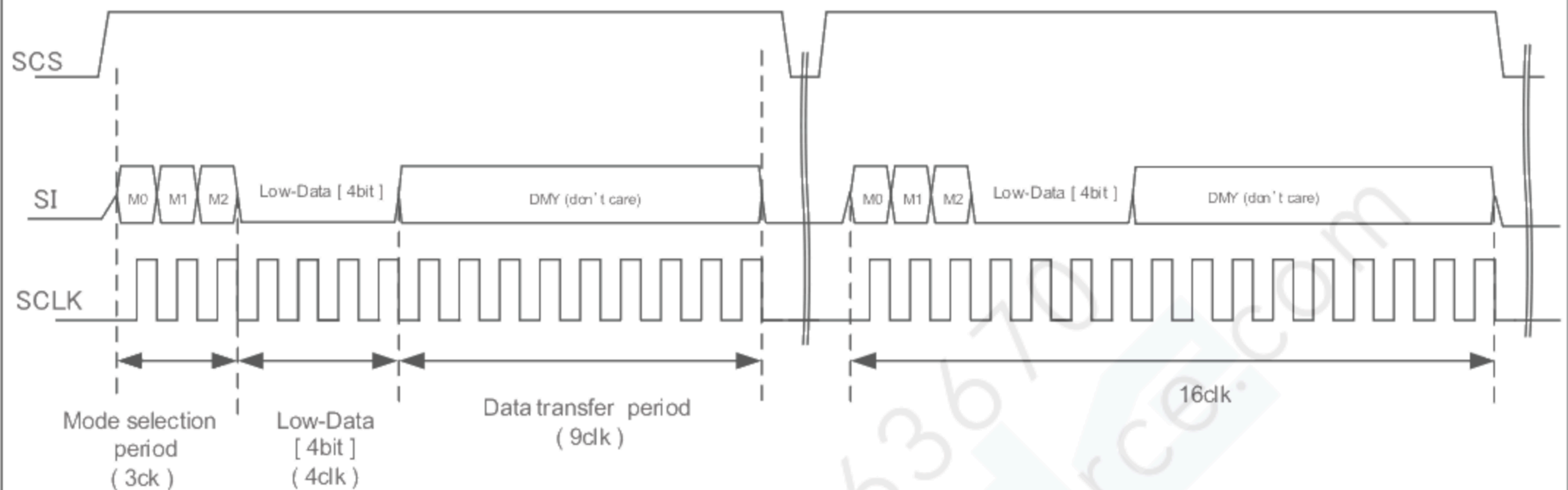
Figure 6-7 Hold mode
