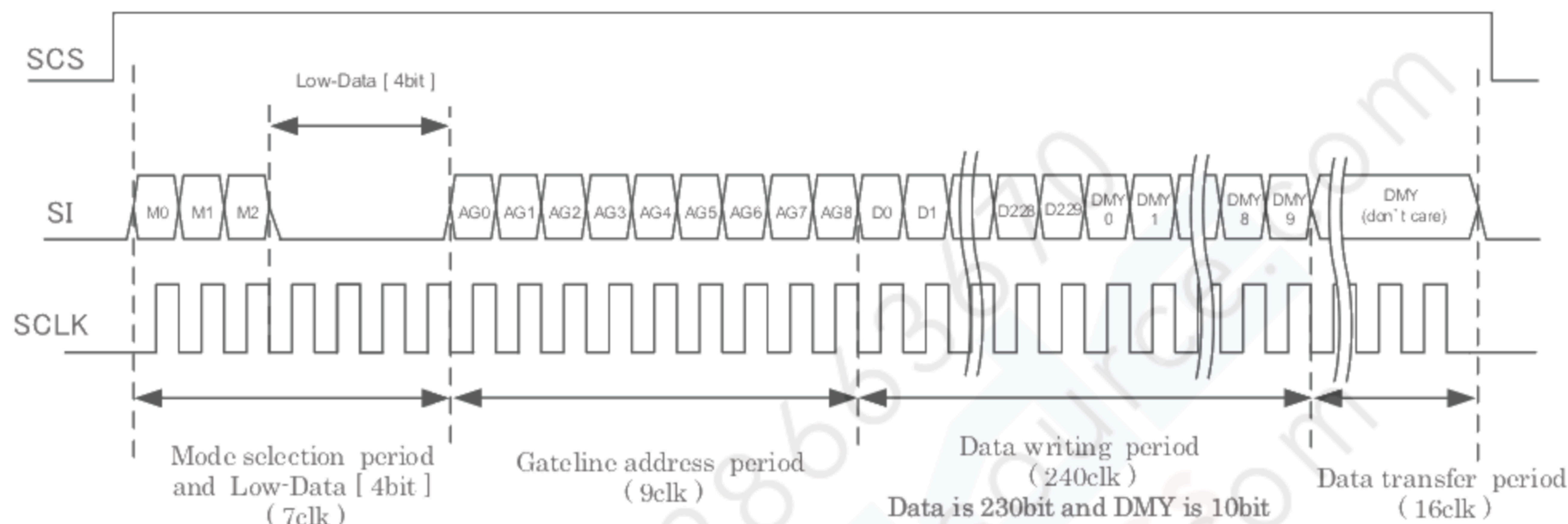
Figure 6-5 Data update mode by 1line
