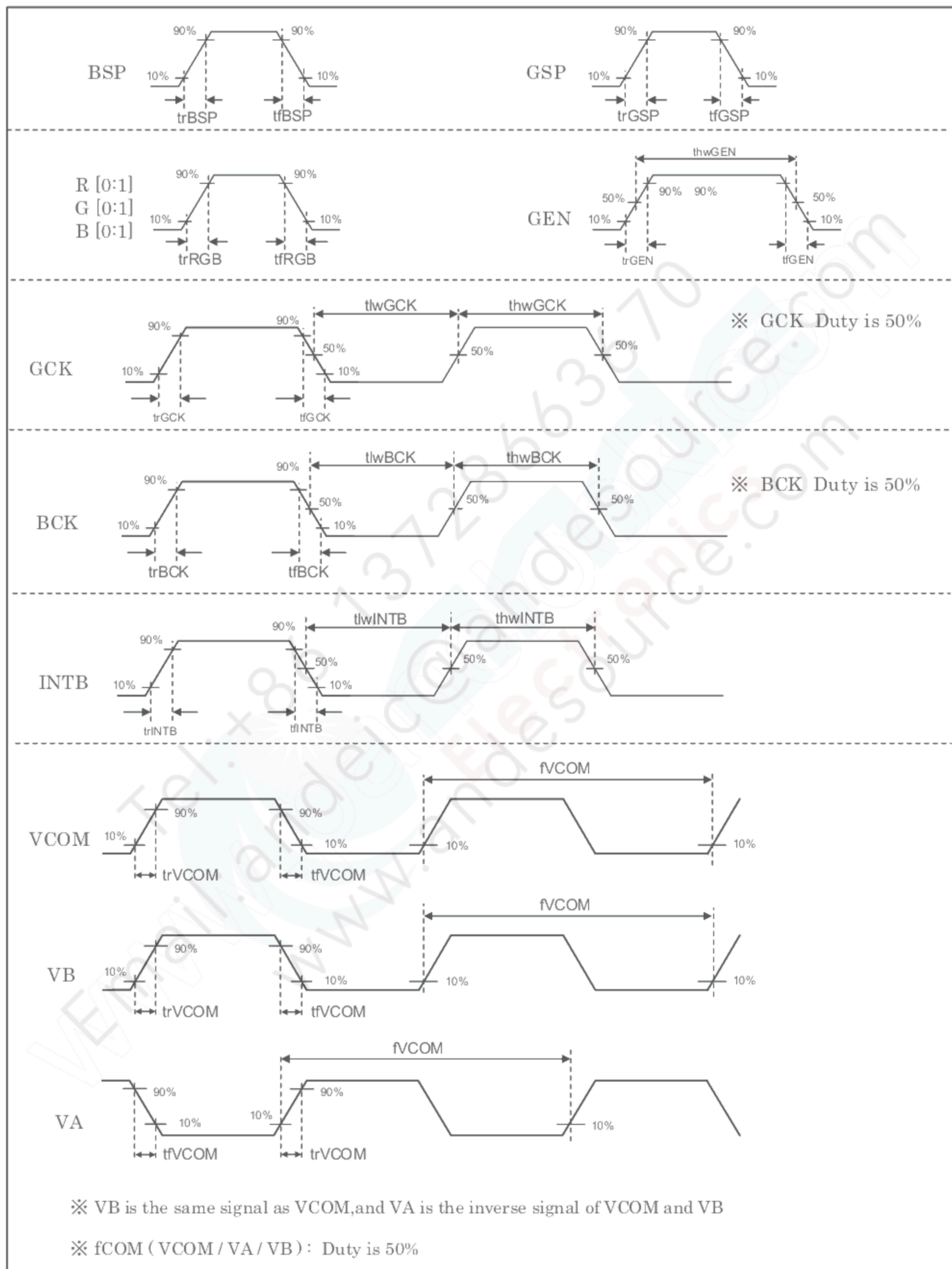
Figure 6-3-2 AC timing 1
