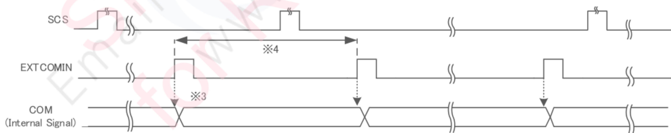
Figure 6-11 COM Inversion (EXTMODE=Hi)2
