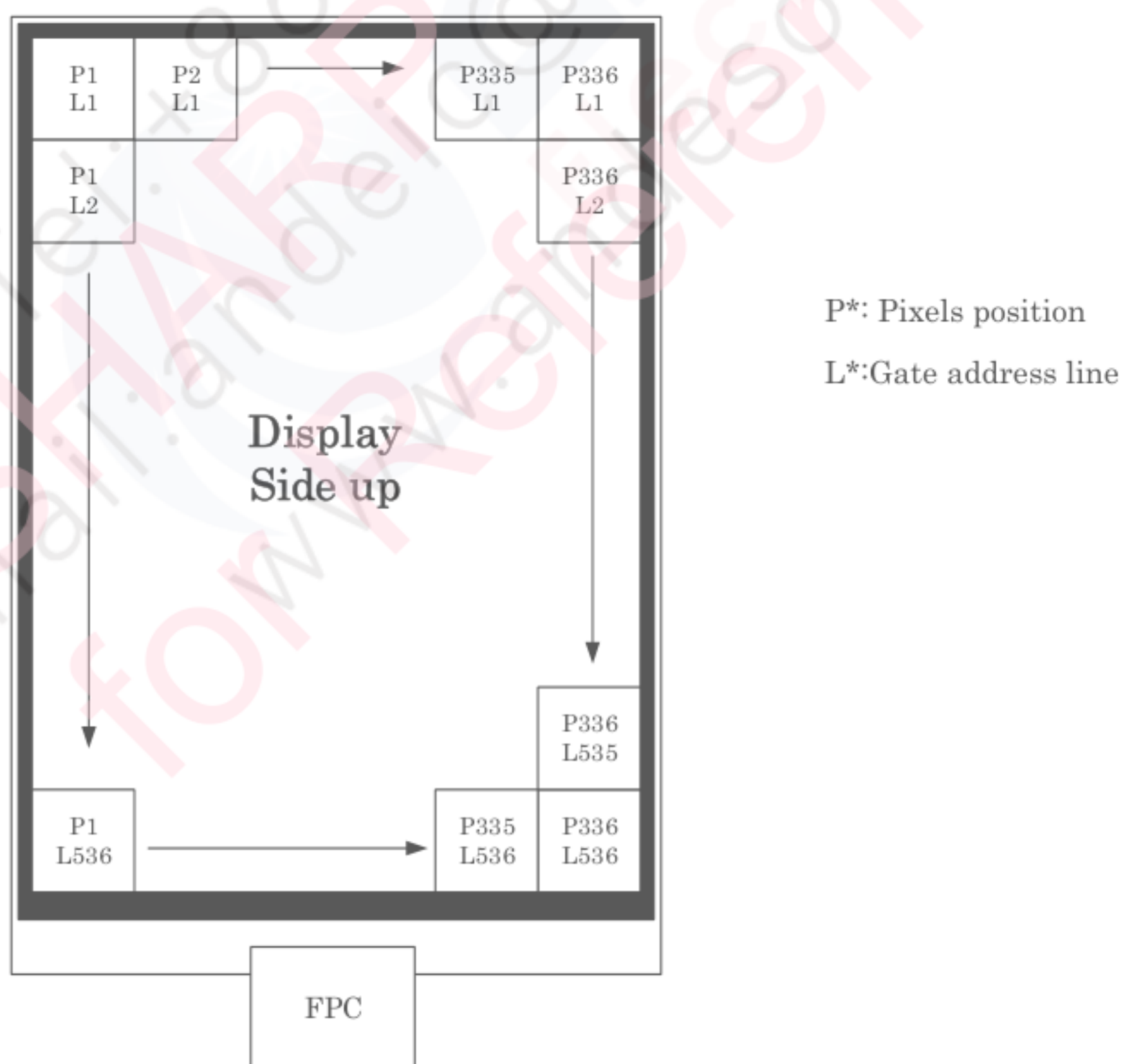
Figure 6-12 Data position
