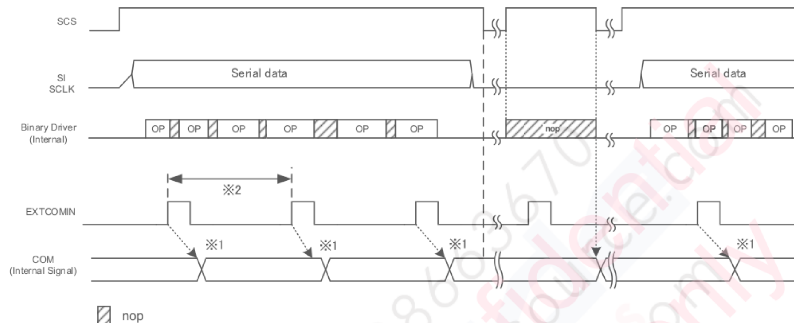
Figure 6-10 COM Inversion (EXTMODE=Hi) 1
