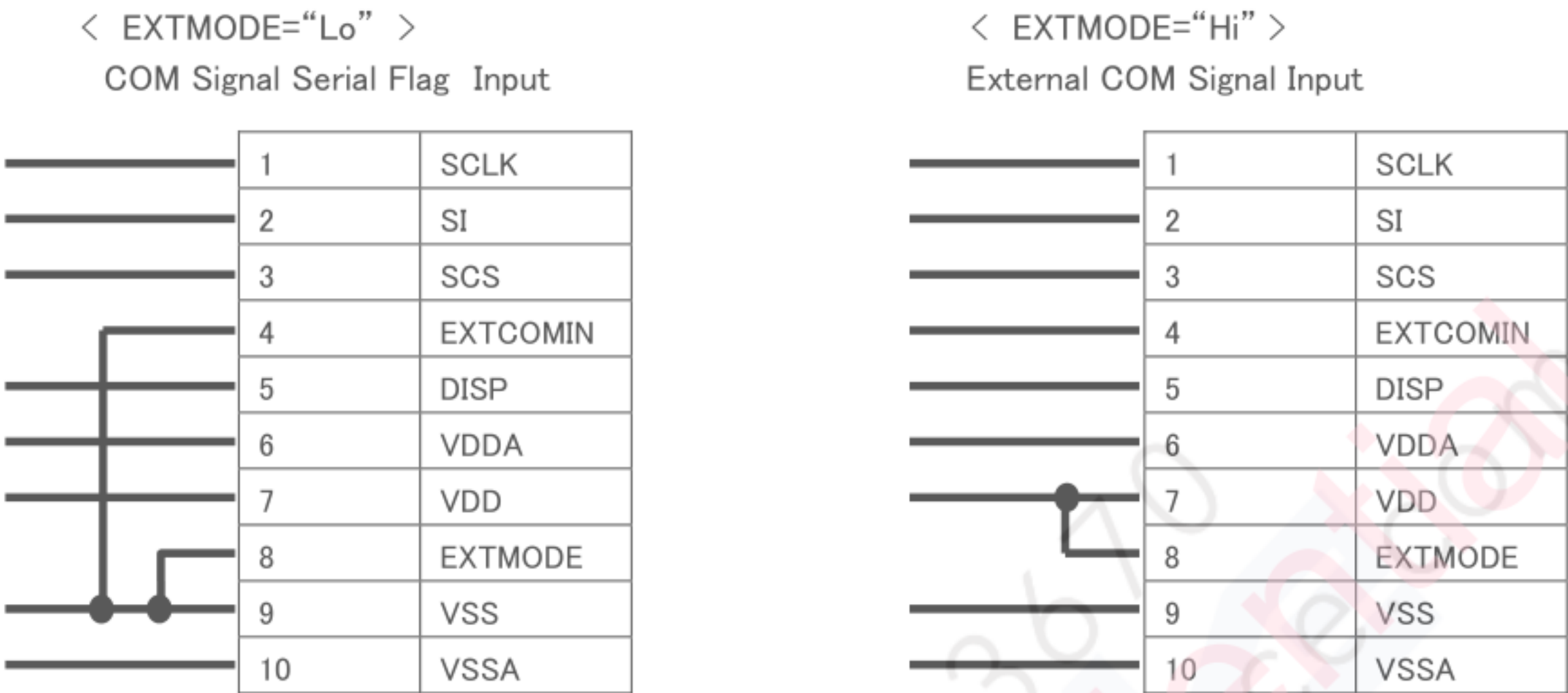
Figure 4-1 Recommended circuit
