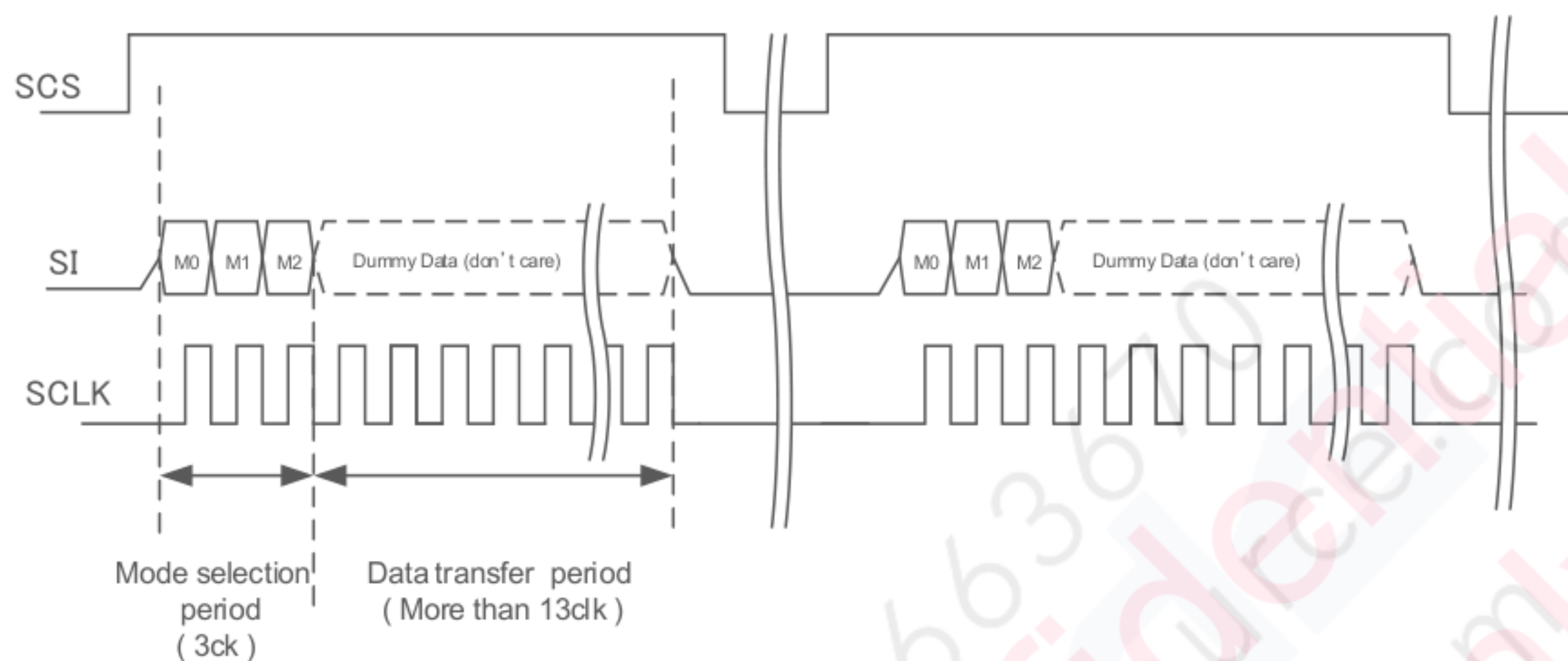
Figure 6-7 Display mode
