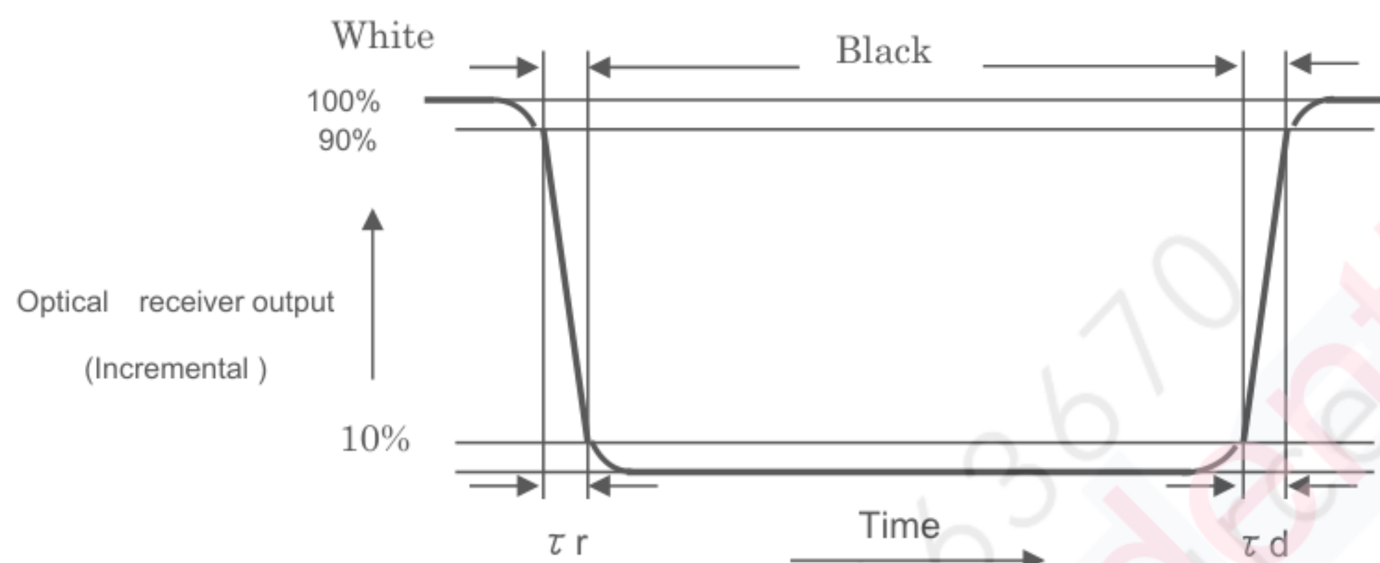
Figure 7-4 Respons time
