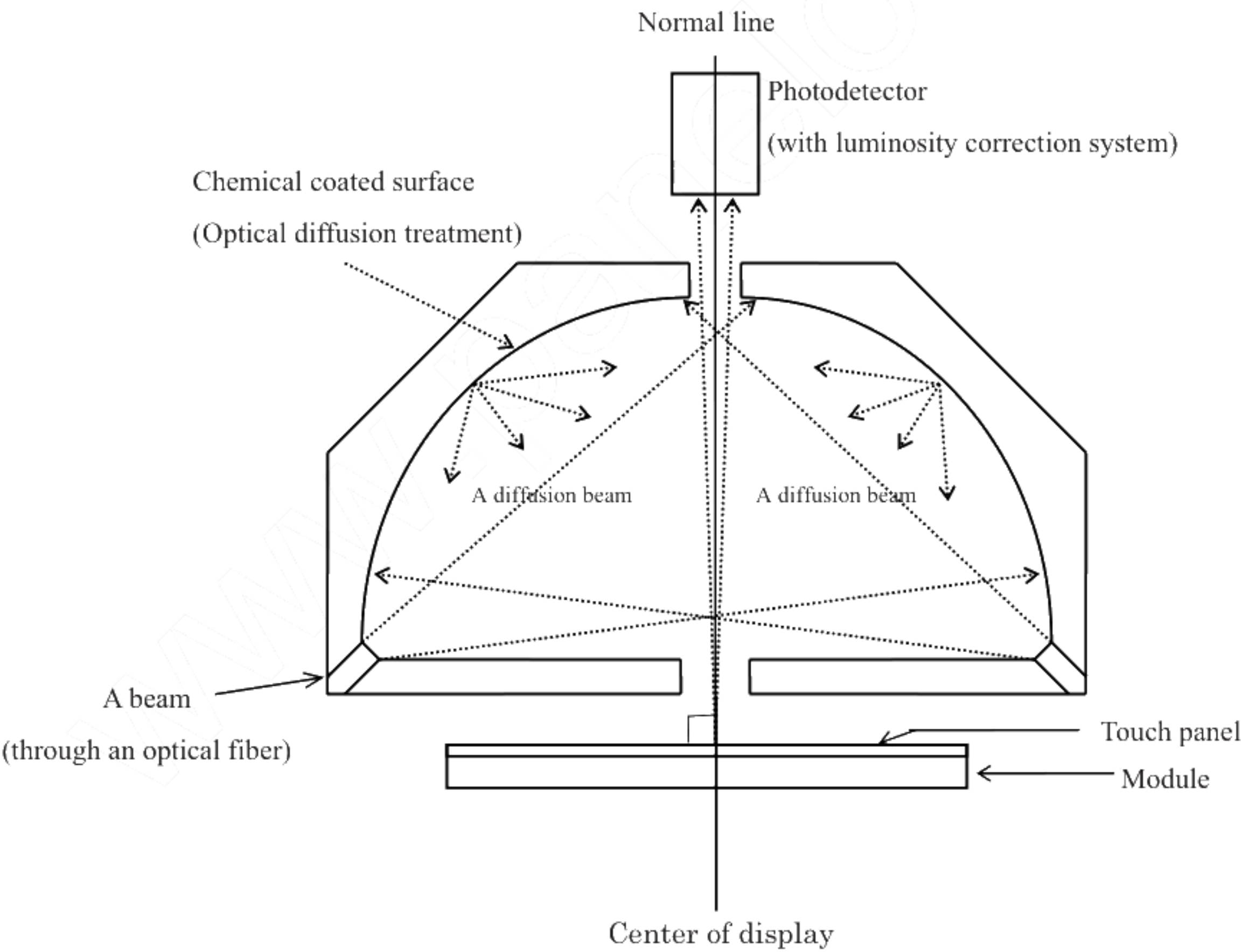
Measuring method (a) for optical characteristics
