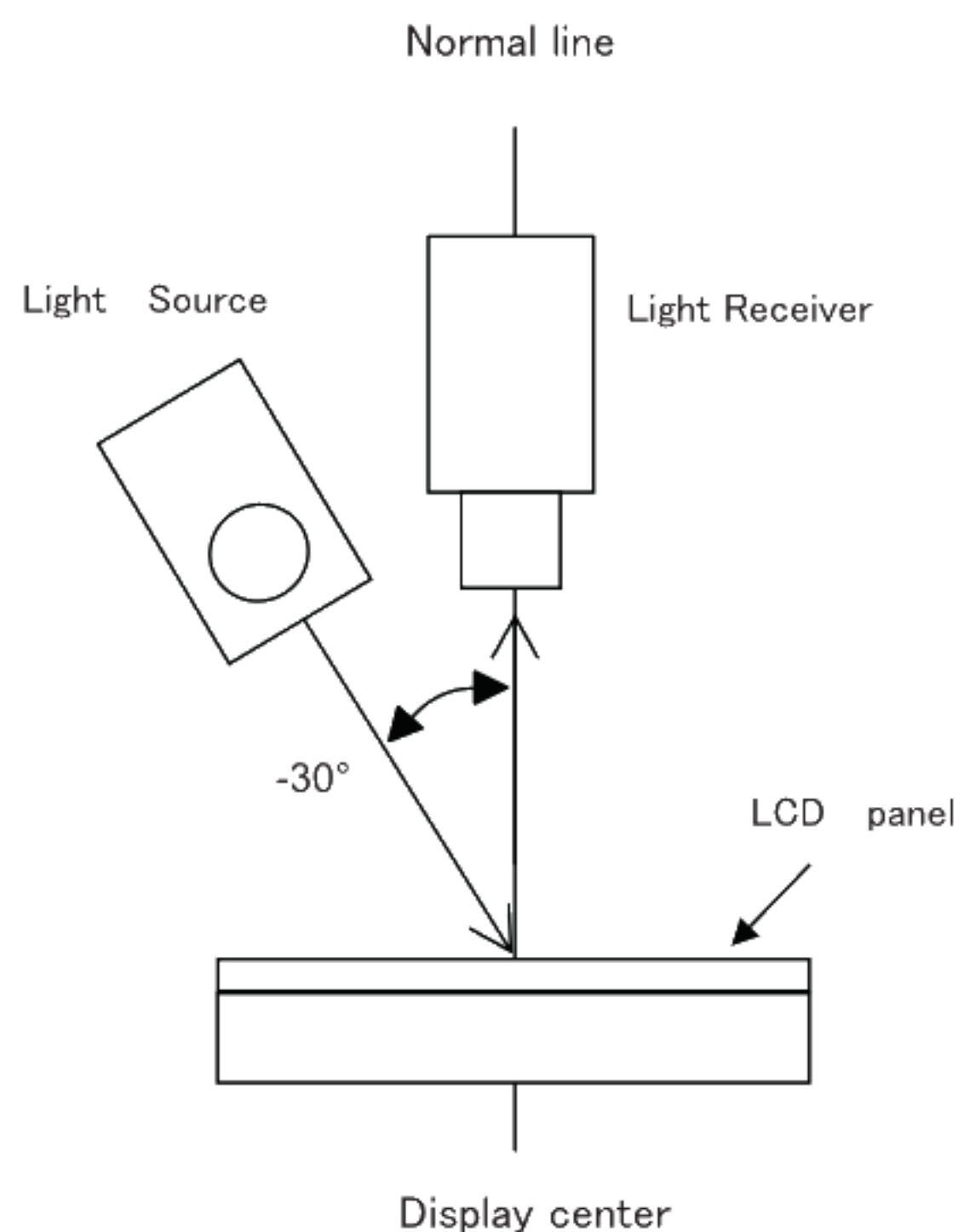
Figure 7-3 Response time
