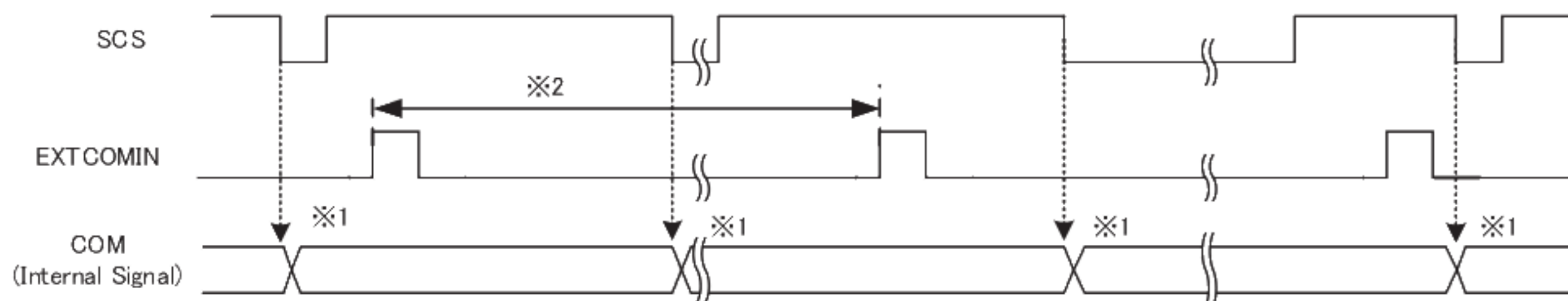
Figure 6-10 COM Inversion (EXTMODE=Hi) 1
