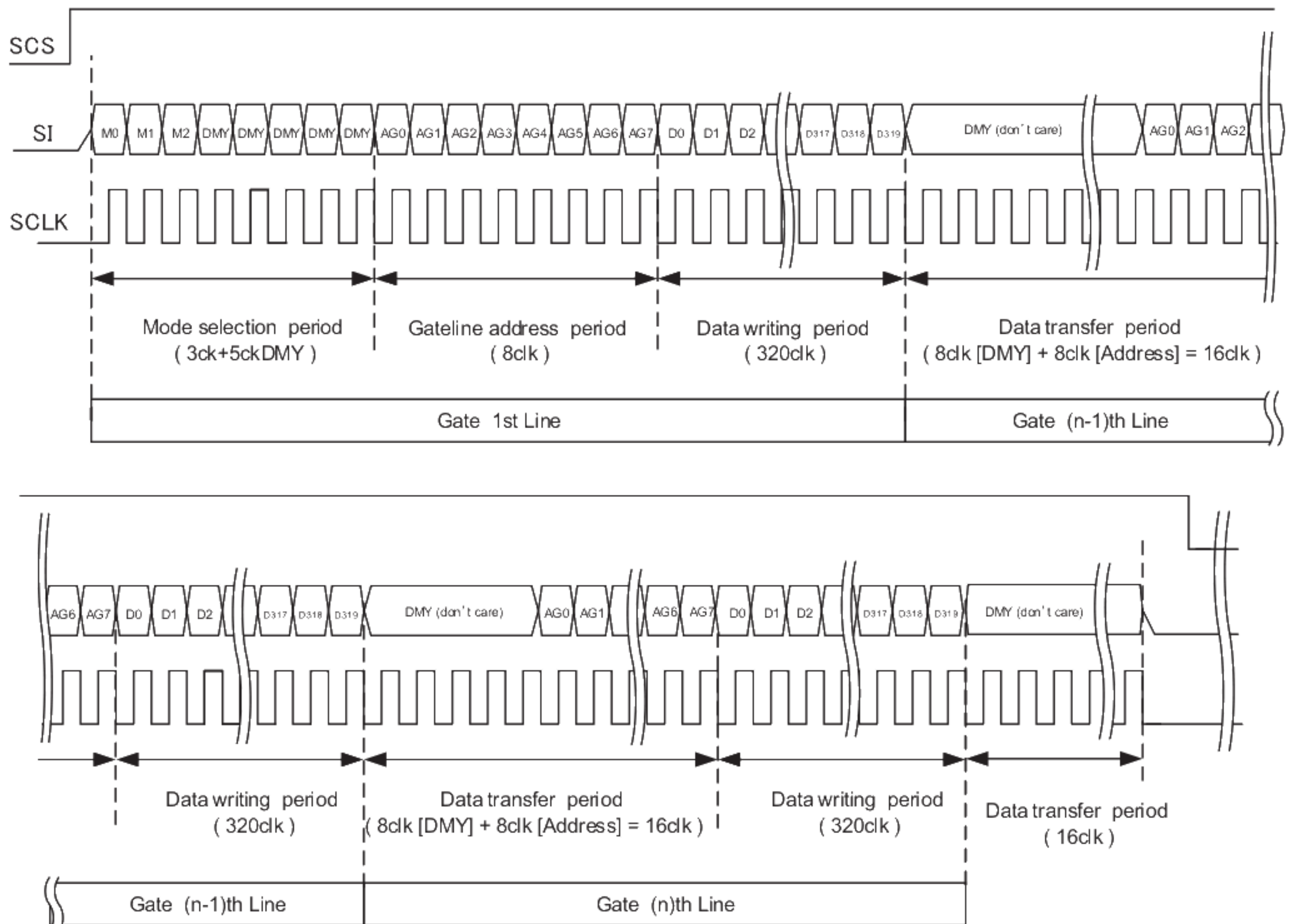
Figure 6-7 Data update mode by Multiple Lines
