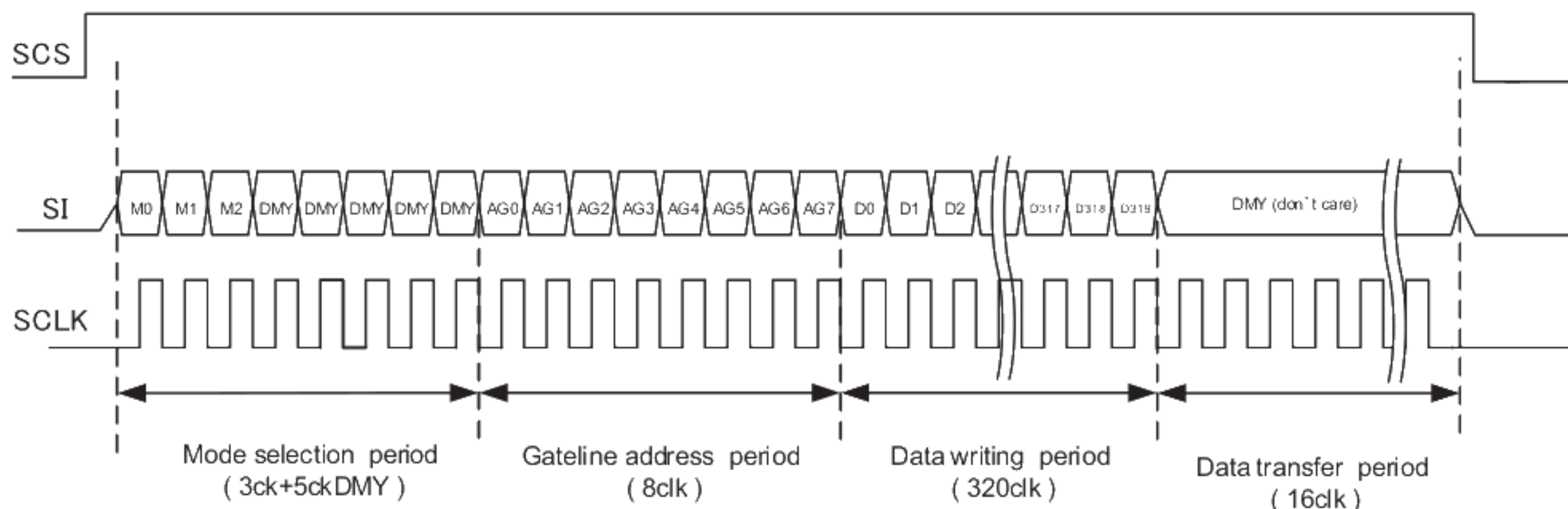
Figure 6-5 Data update mode by 1line
