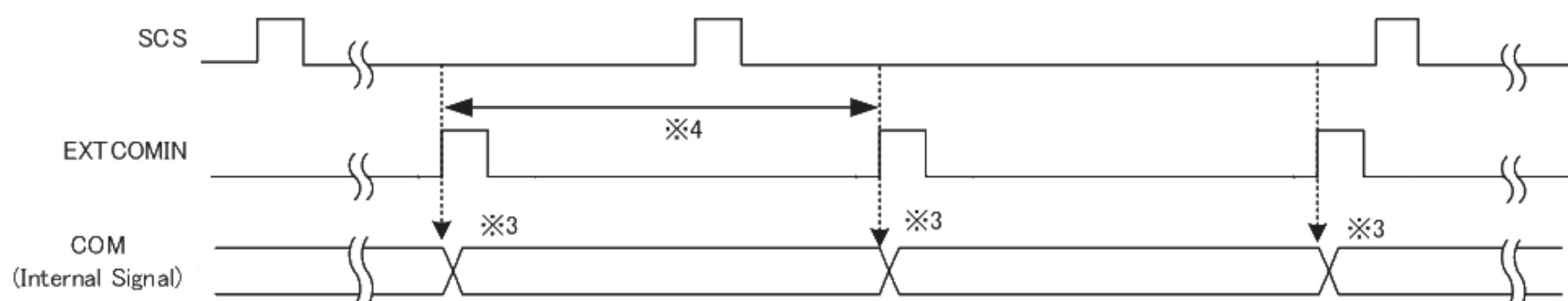
Figure 6-11 COM Inversion (EXTMODE=Hi)2
