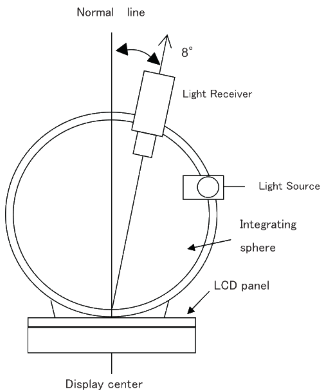
Figure 7-2 Contrast ratio, Reflection ratio, Panel chromaticity
