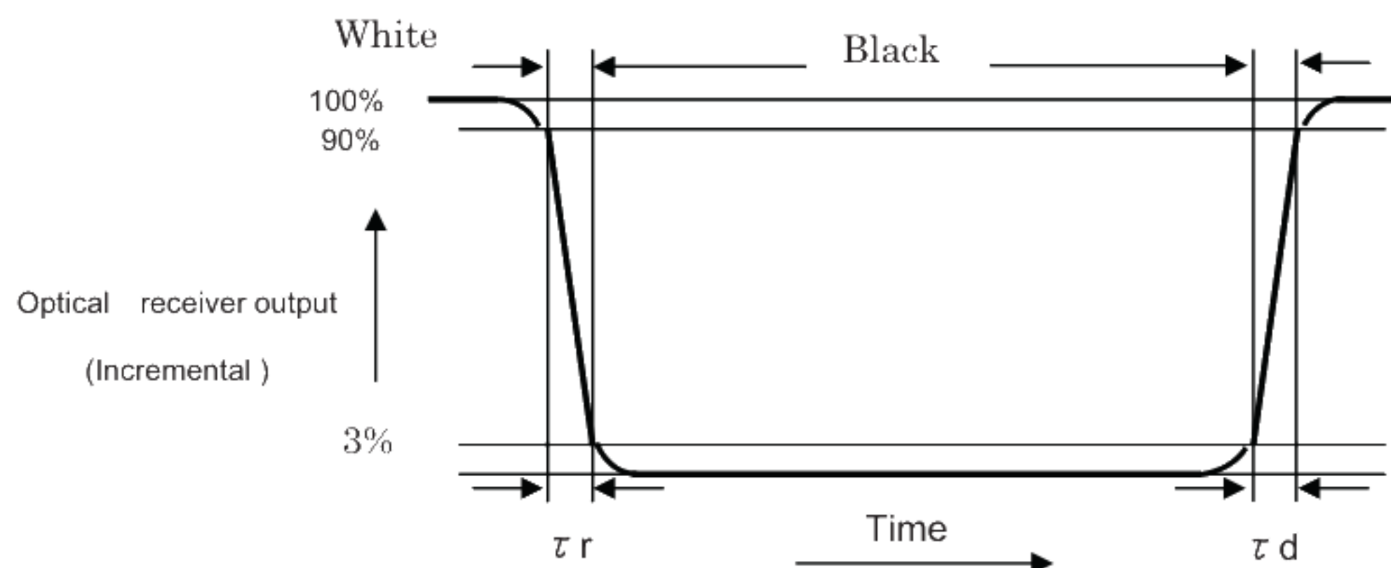
Figure 7-4 Respons time
