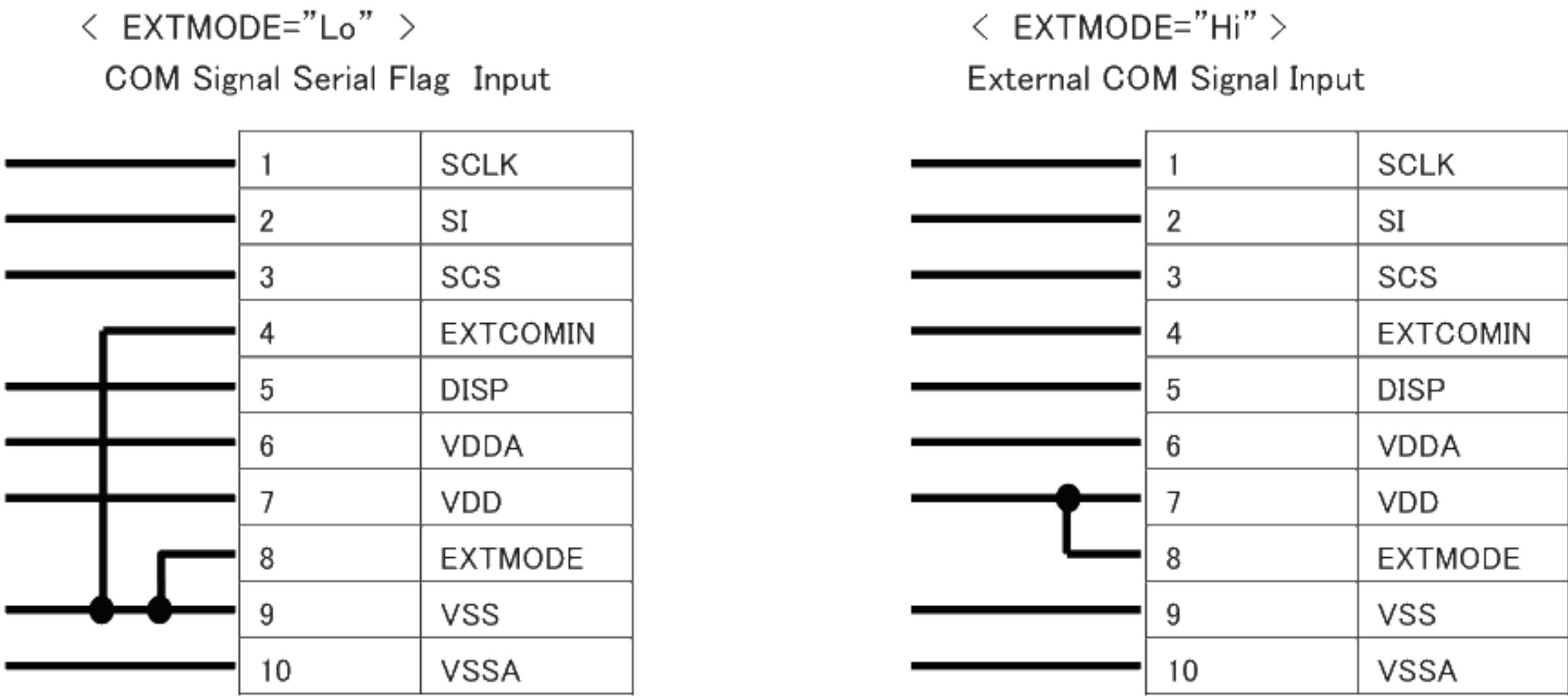
Figure 4-1 Recommended circuit
