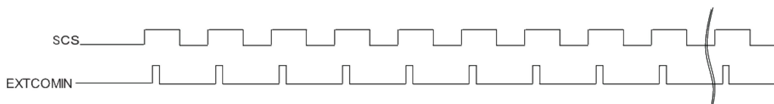
Figure 6-2-1 EXTCOMIN Signal 1
