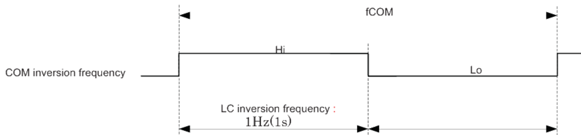
Figure 6-4 COM inversion frequency
