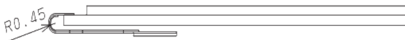
Figure 8-2 FPC Bend Specification
