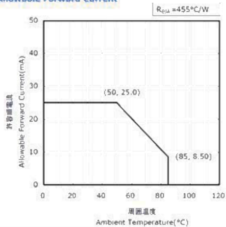
Fig.1 LED Characteristic (De-rating Curve)
