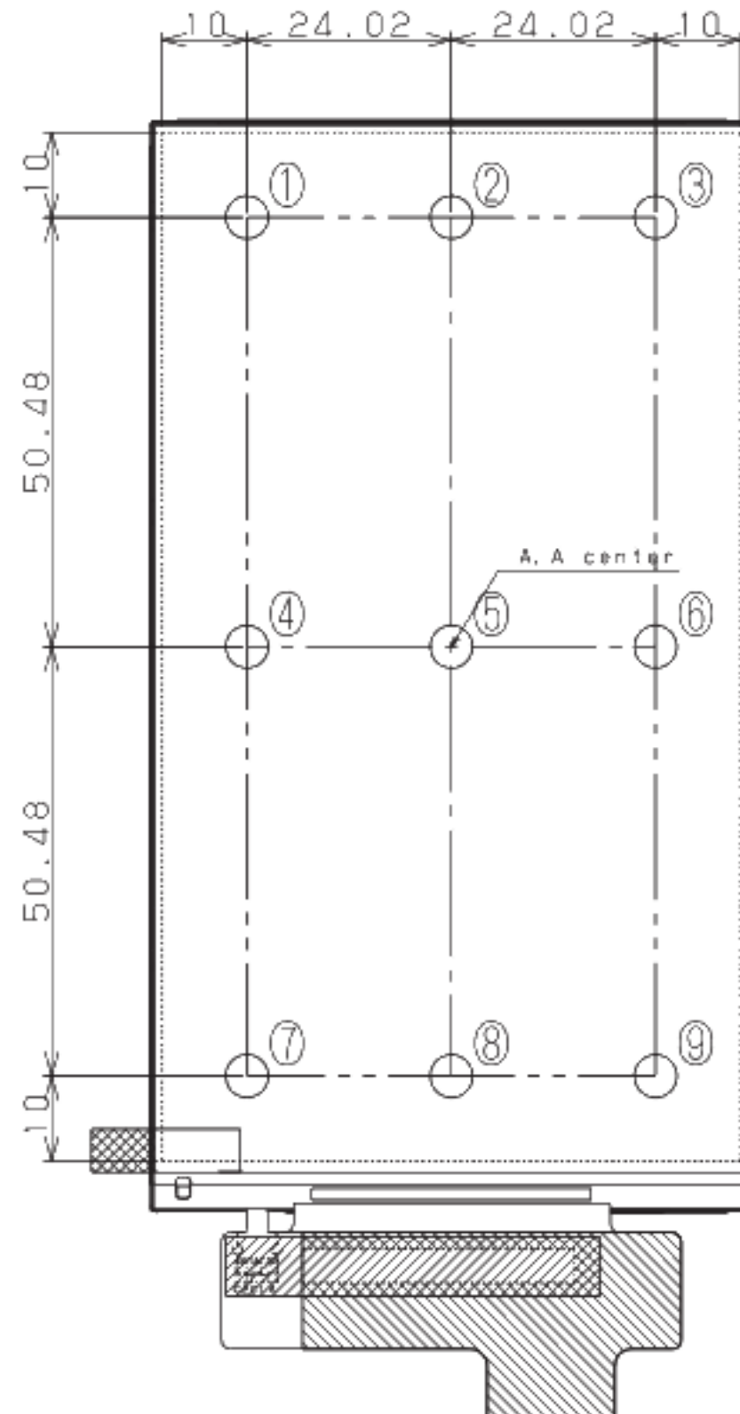
Fig. 9 Measuring Point
