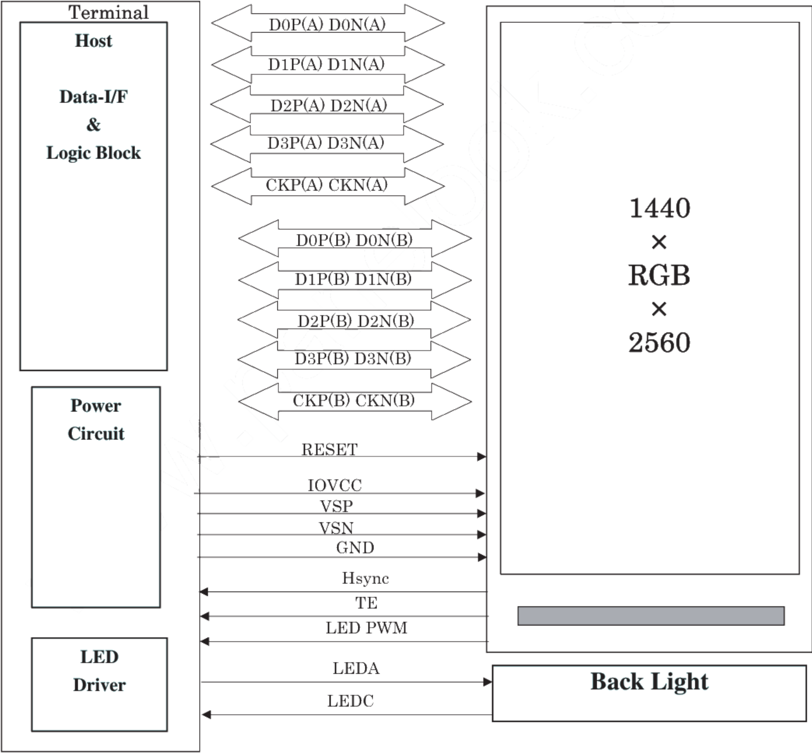
Fig.2 Schematic of LCD module system
