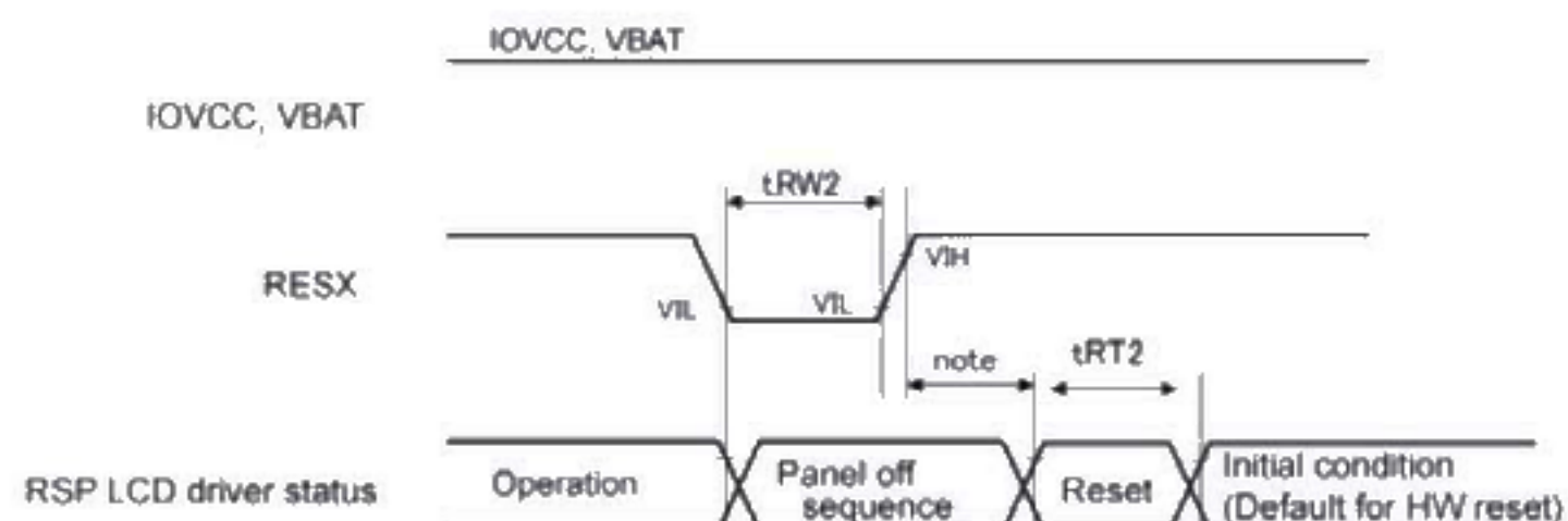
Fig .6 Reset timing characteristics
