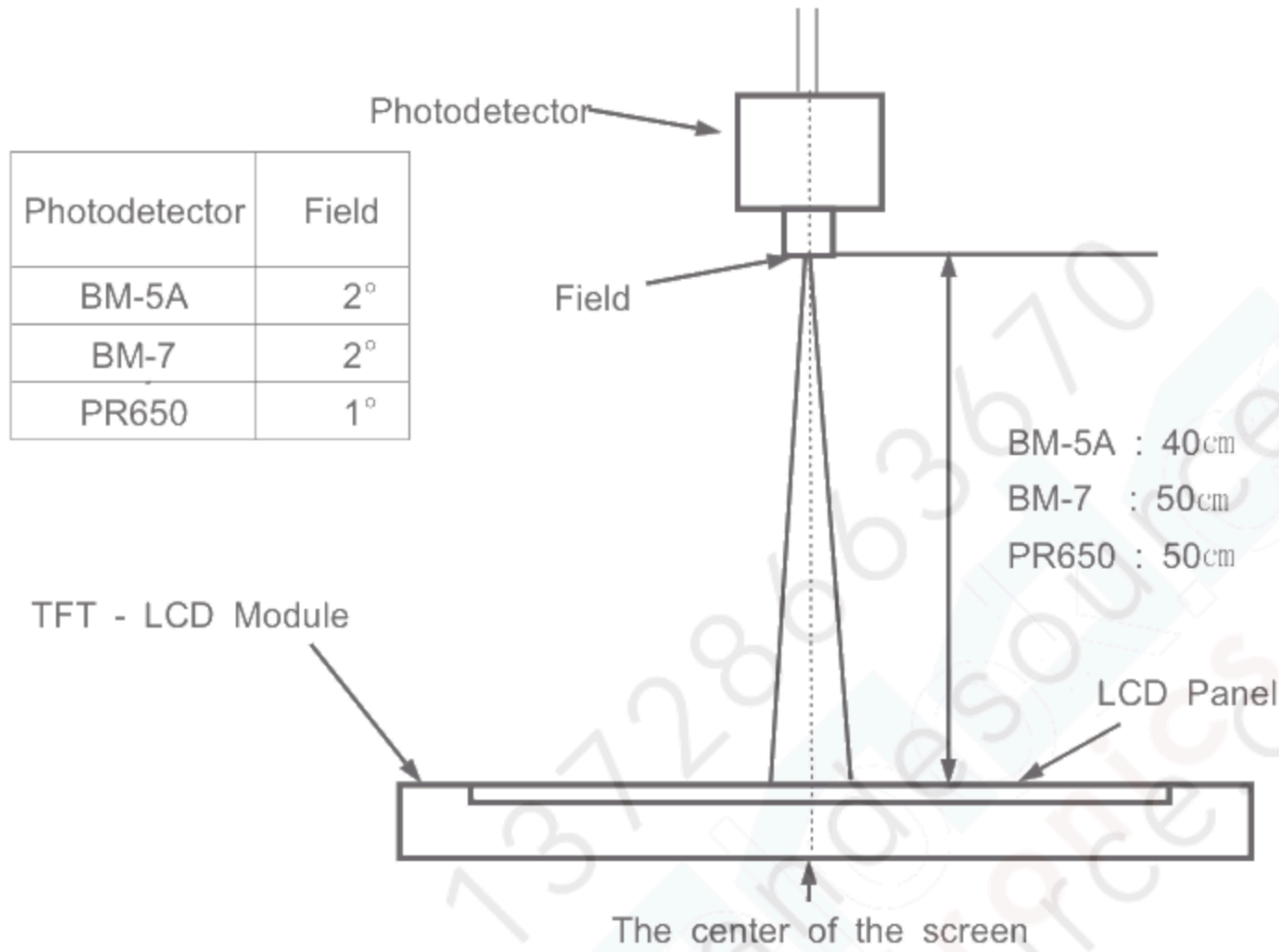
Optical Measuring Equipment Setup
