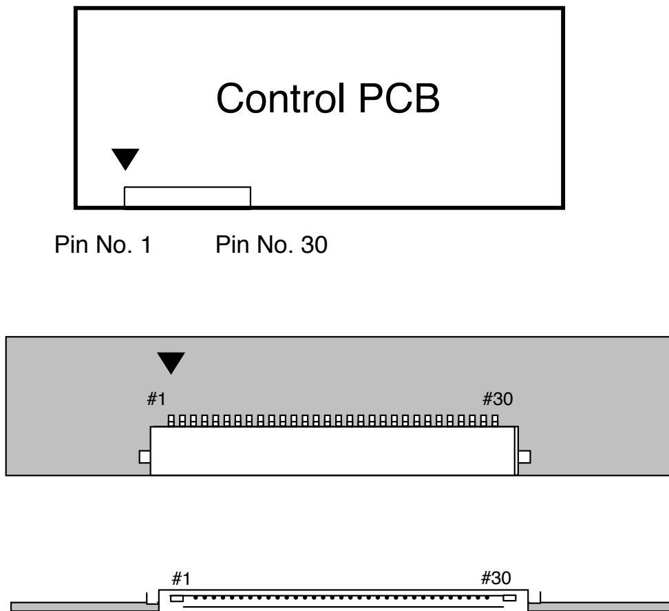
Fig. Connector diagram
