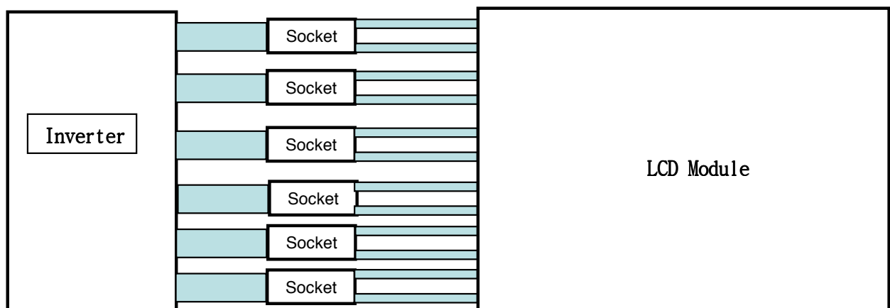
Fig. Measurement point of Lamp Current
