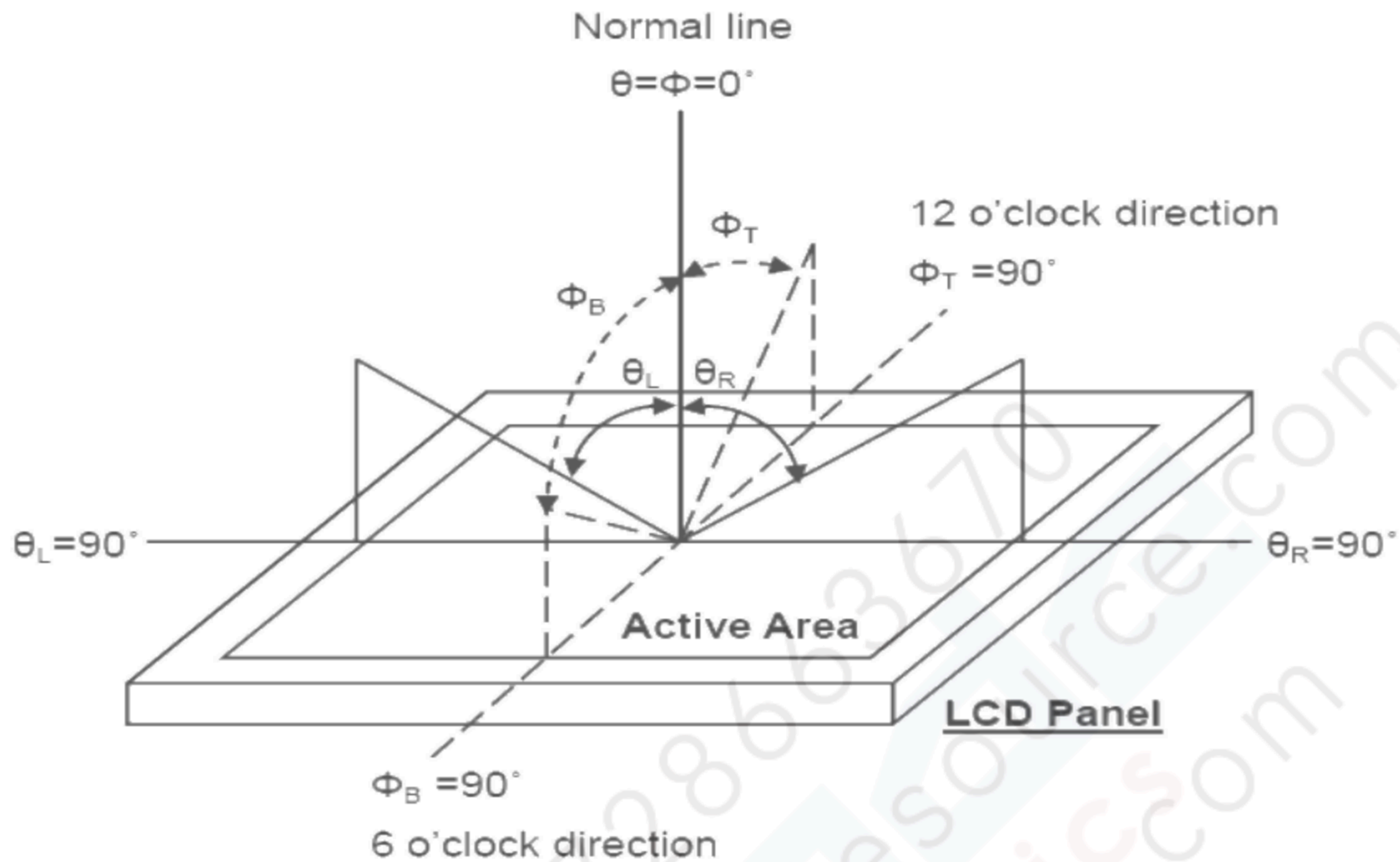
Fig. 7-1 Definition of viewing angle
