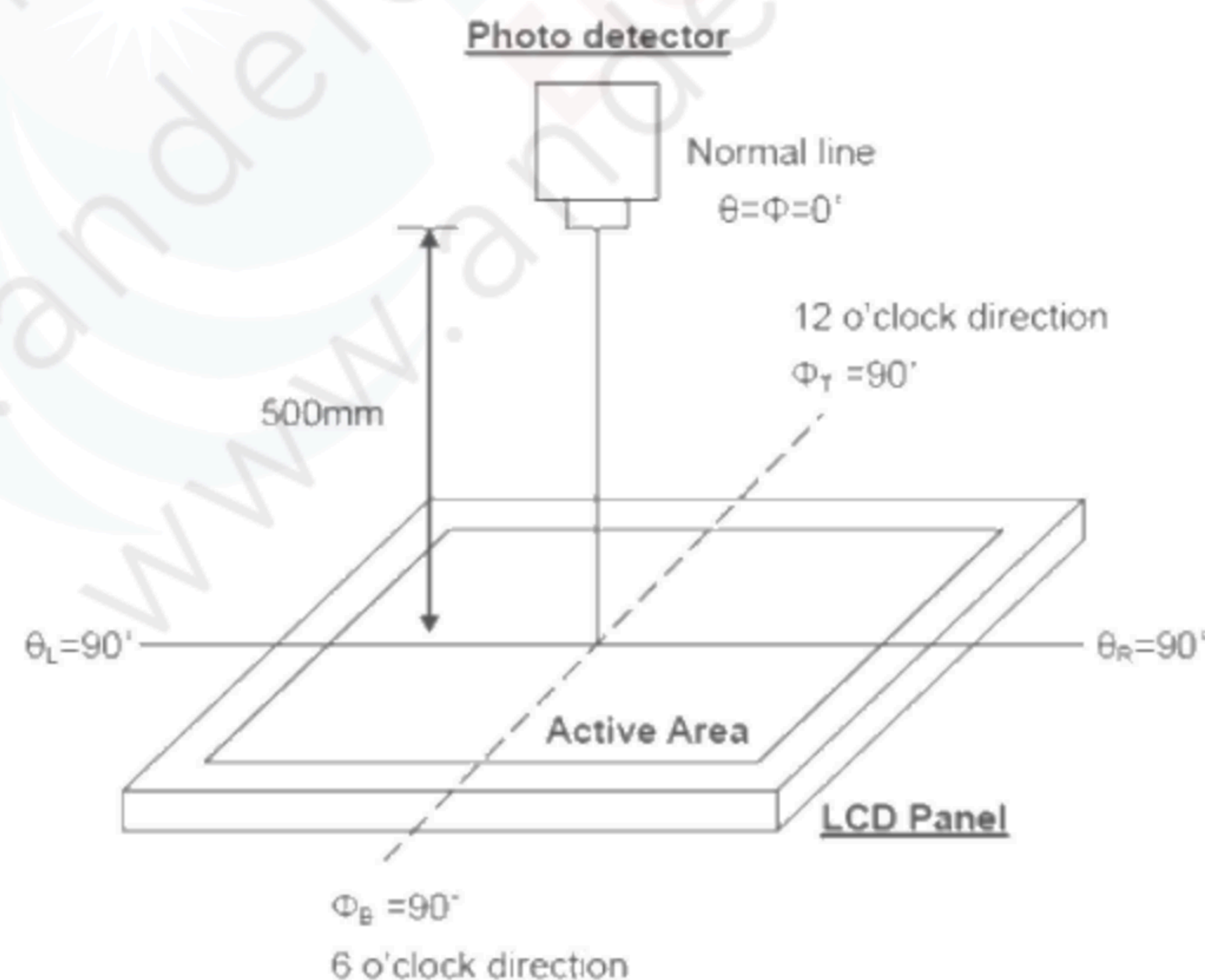
Fig.7-2 Optical measurement system setup
