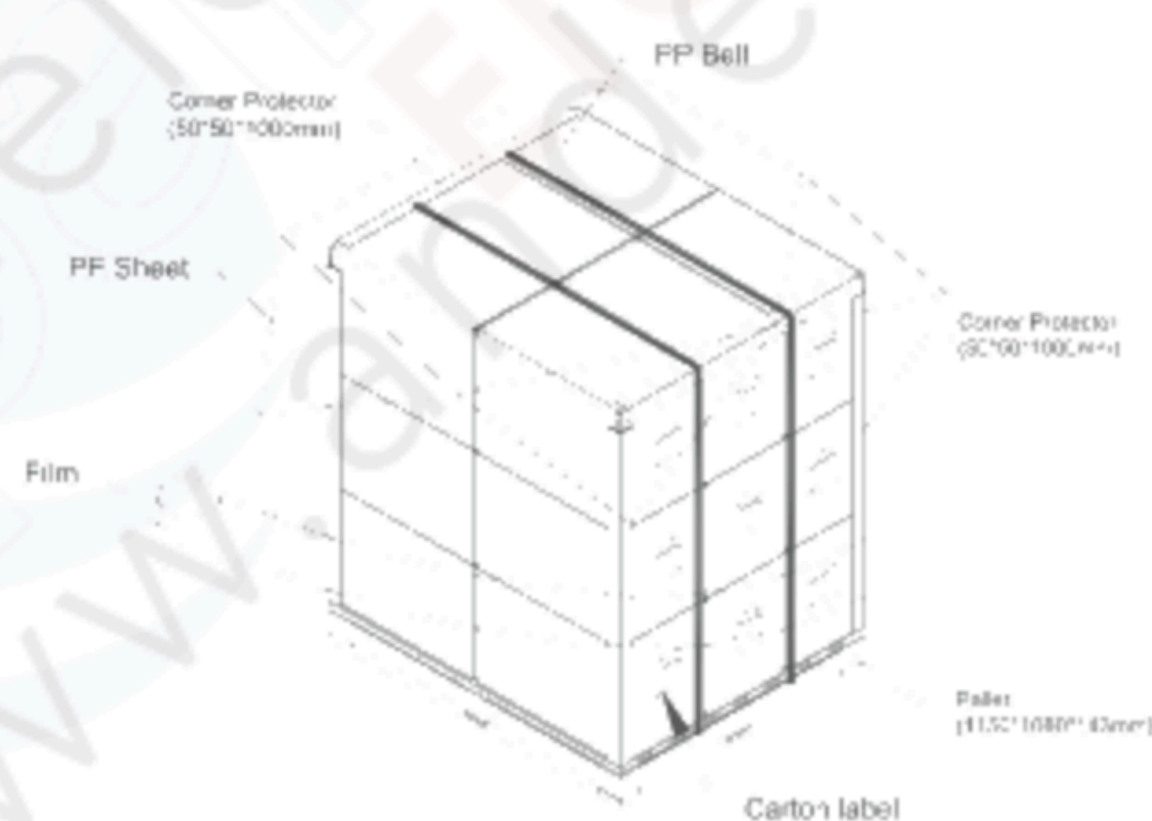
Figure. 7-2 Packing method
