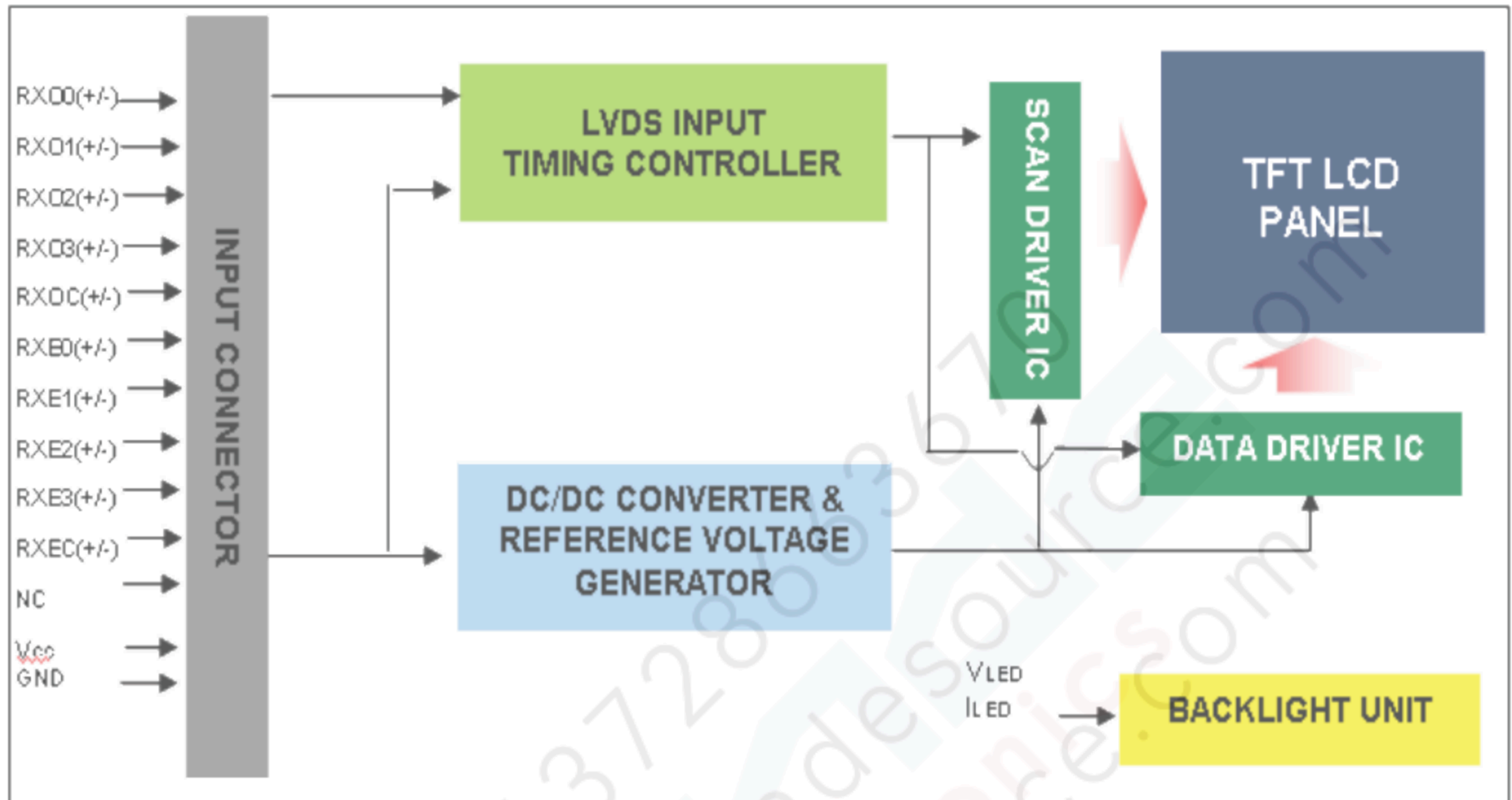
Fig. 4-1 Module Function Block Diagram
