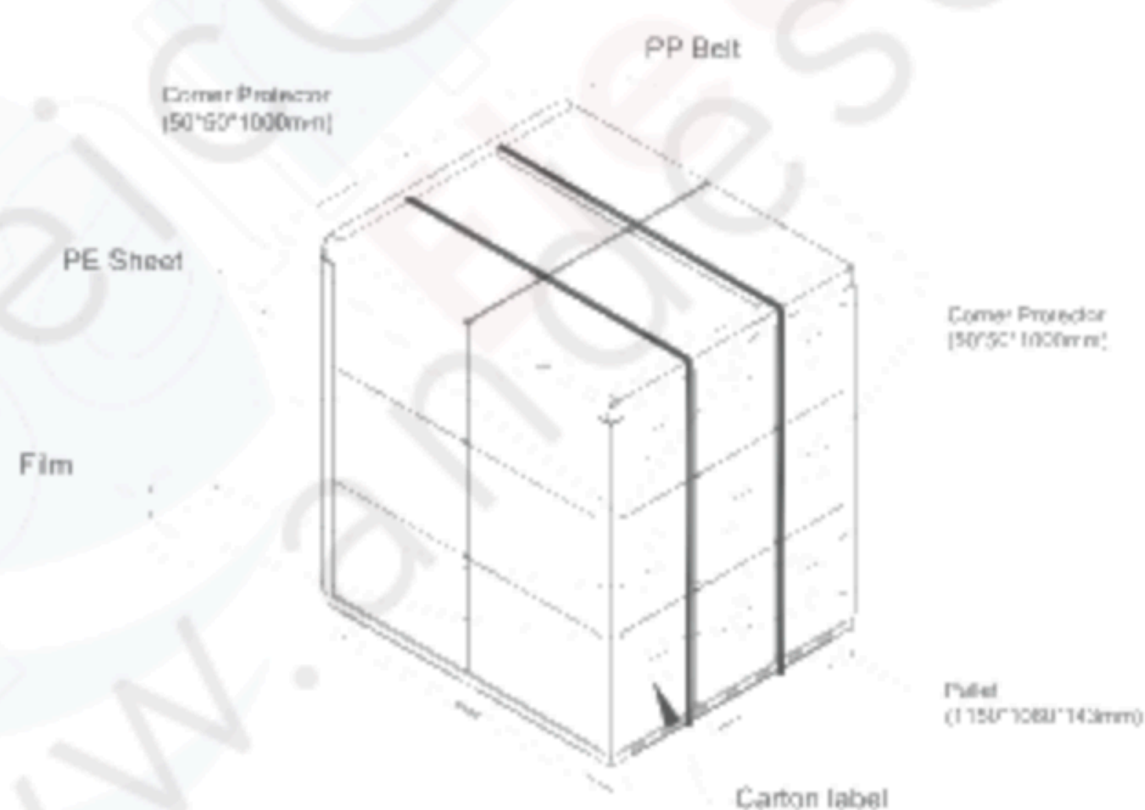
Figure. 7-2 Packing method
