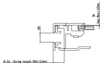
SECTION A-A SCALE 8:1
