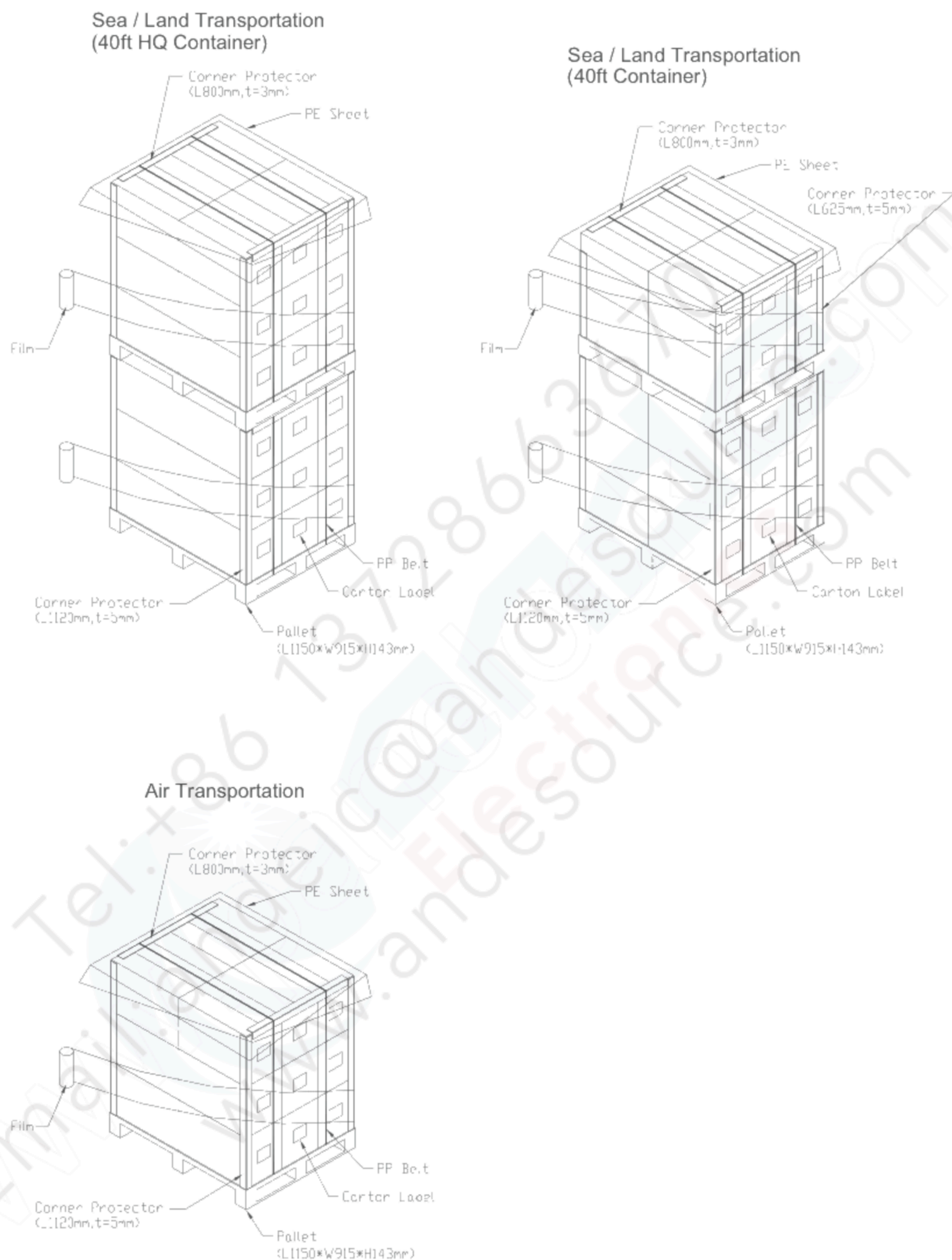
Figure. 8-2 Packing method
