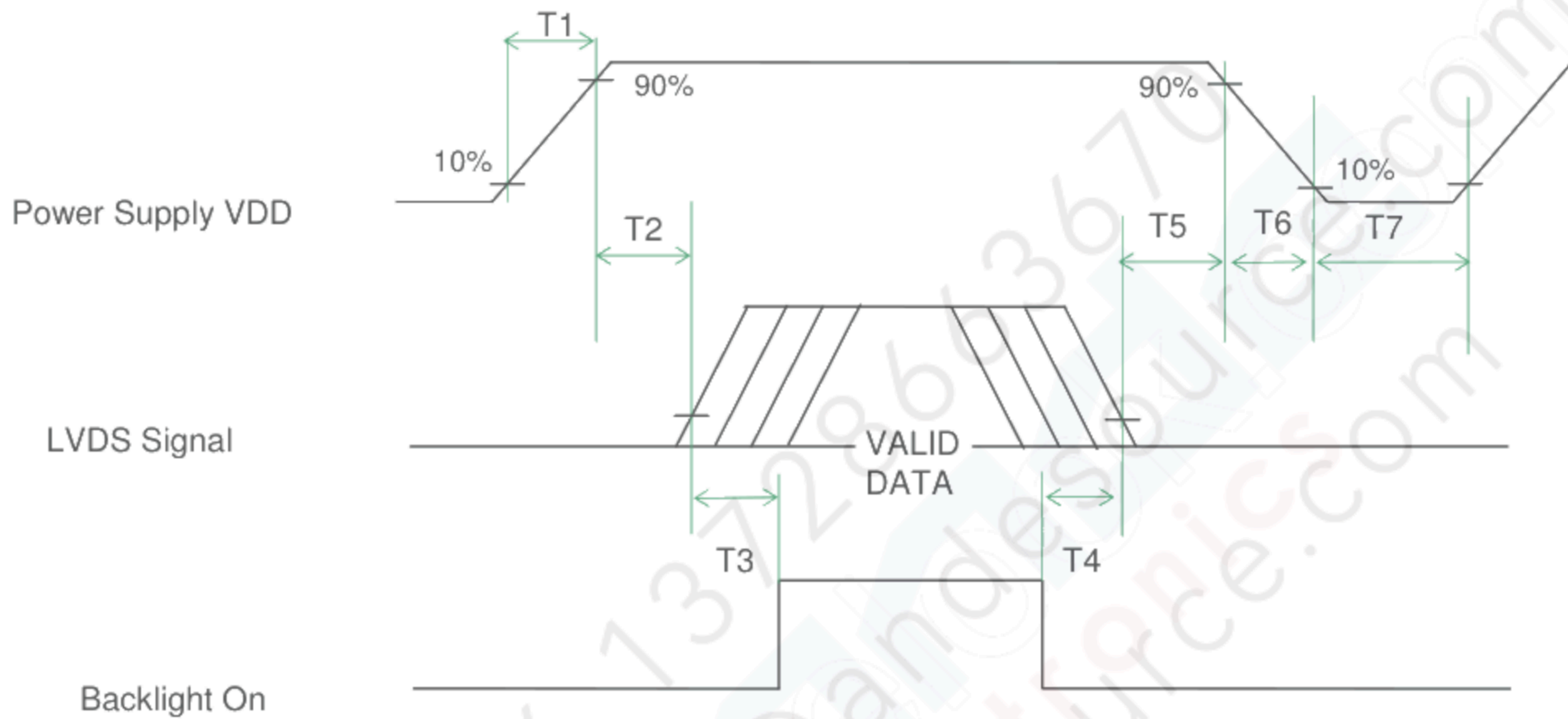
Power Sequence Timing
