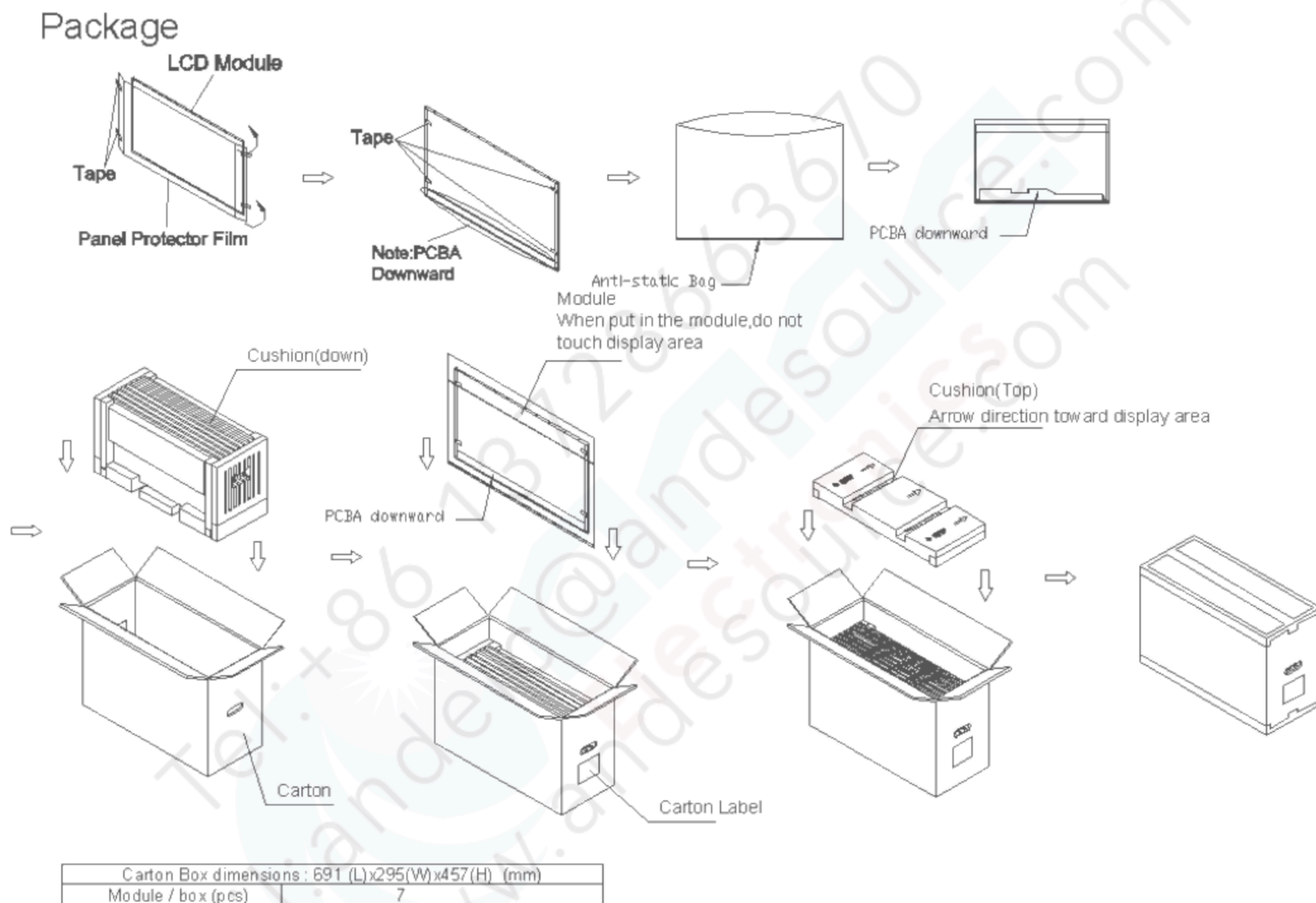
Figure. 8-1 Packing method
