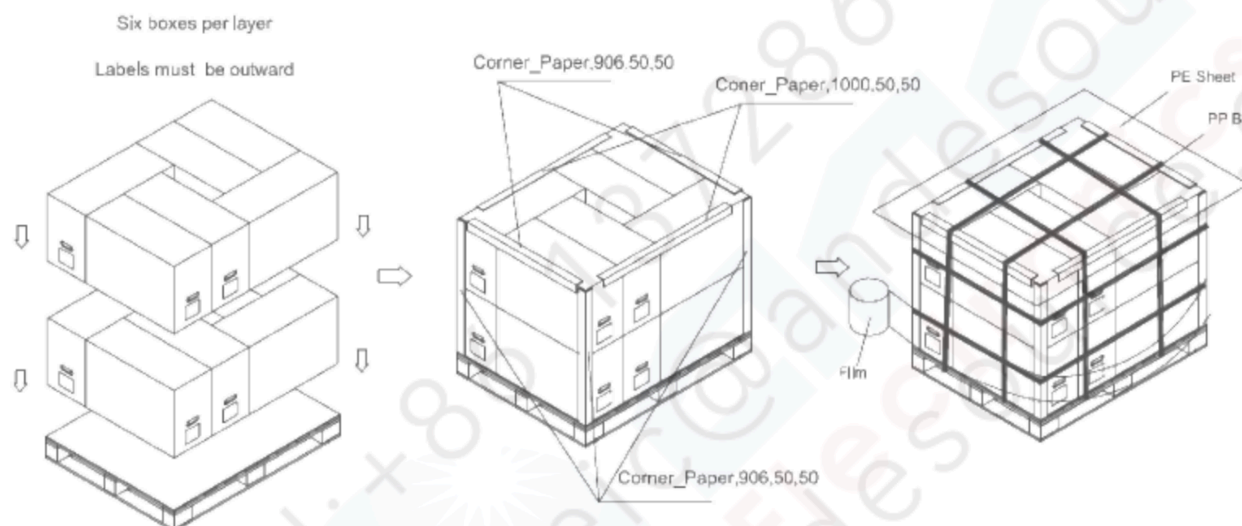
Figure. 8-2 Packing method
