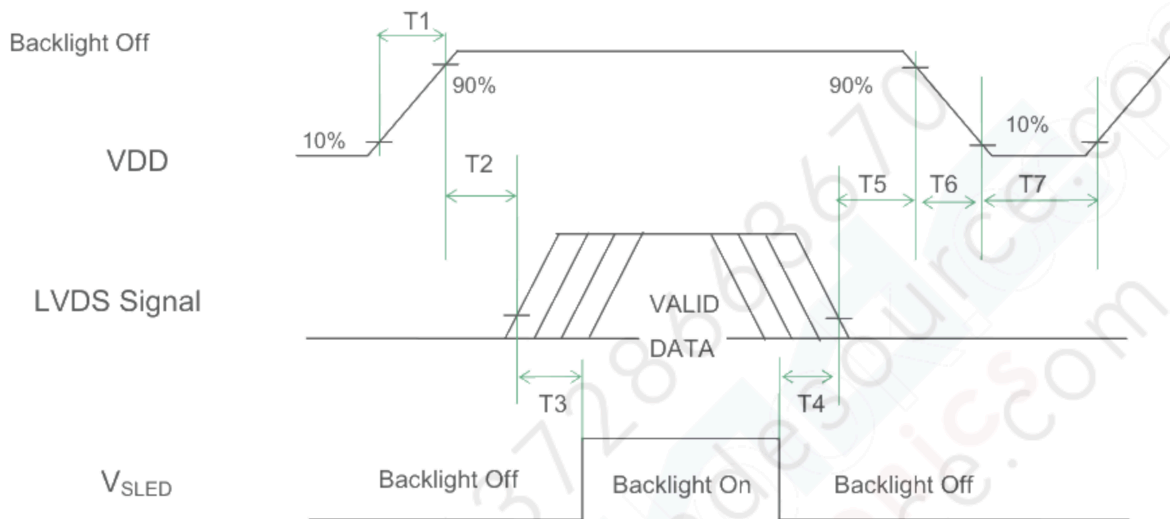
Power Sequence Timing
