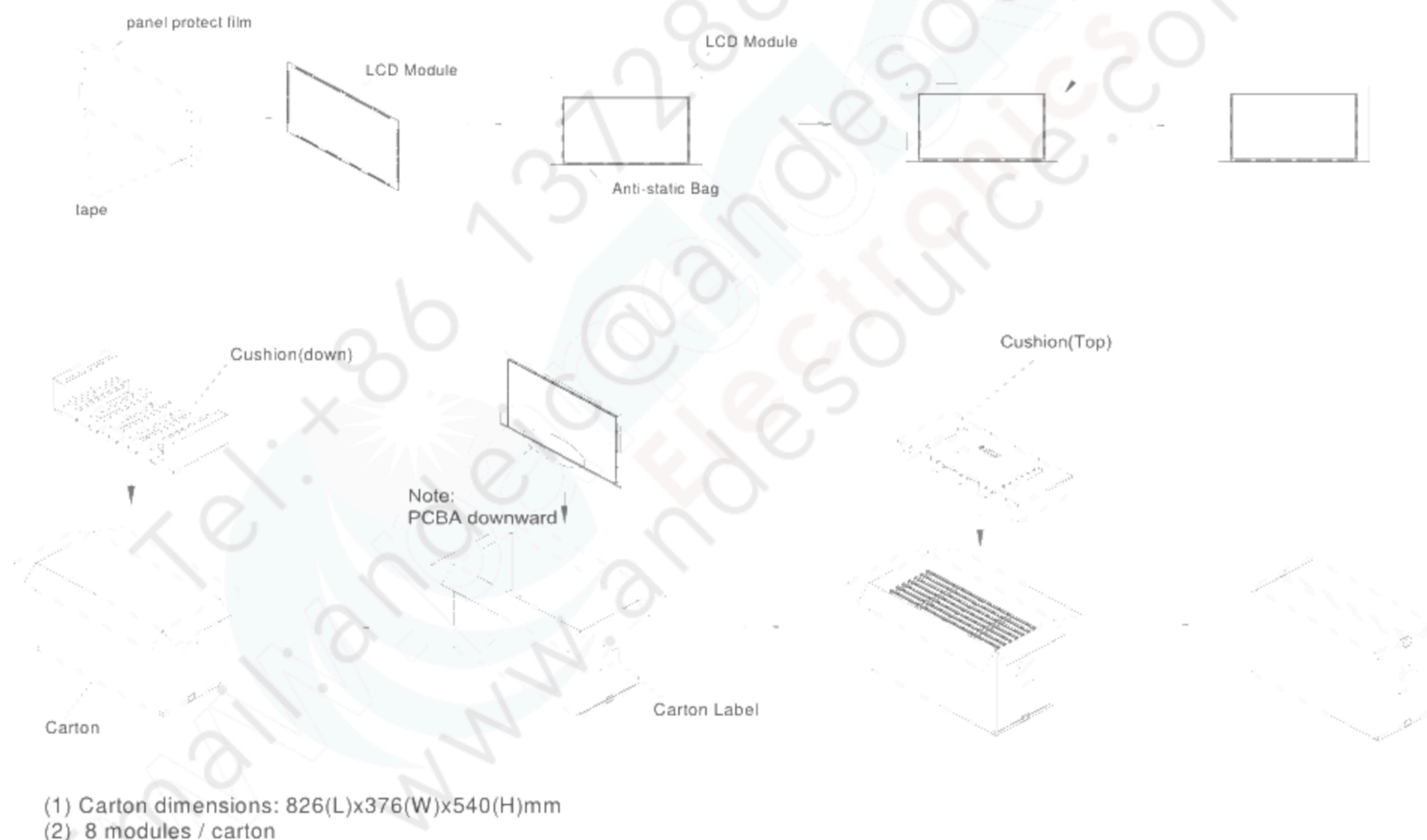
Figure. 8-1 Packing method
