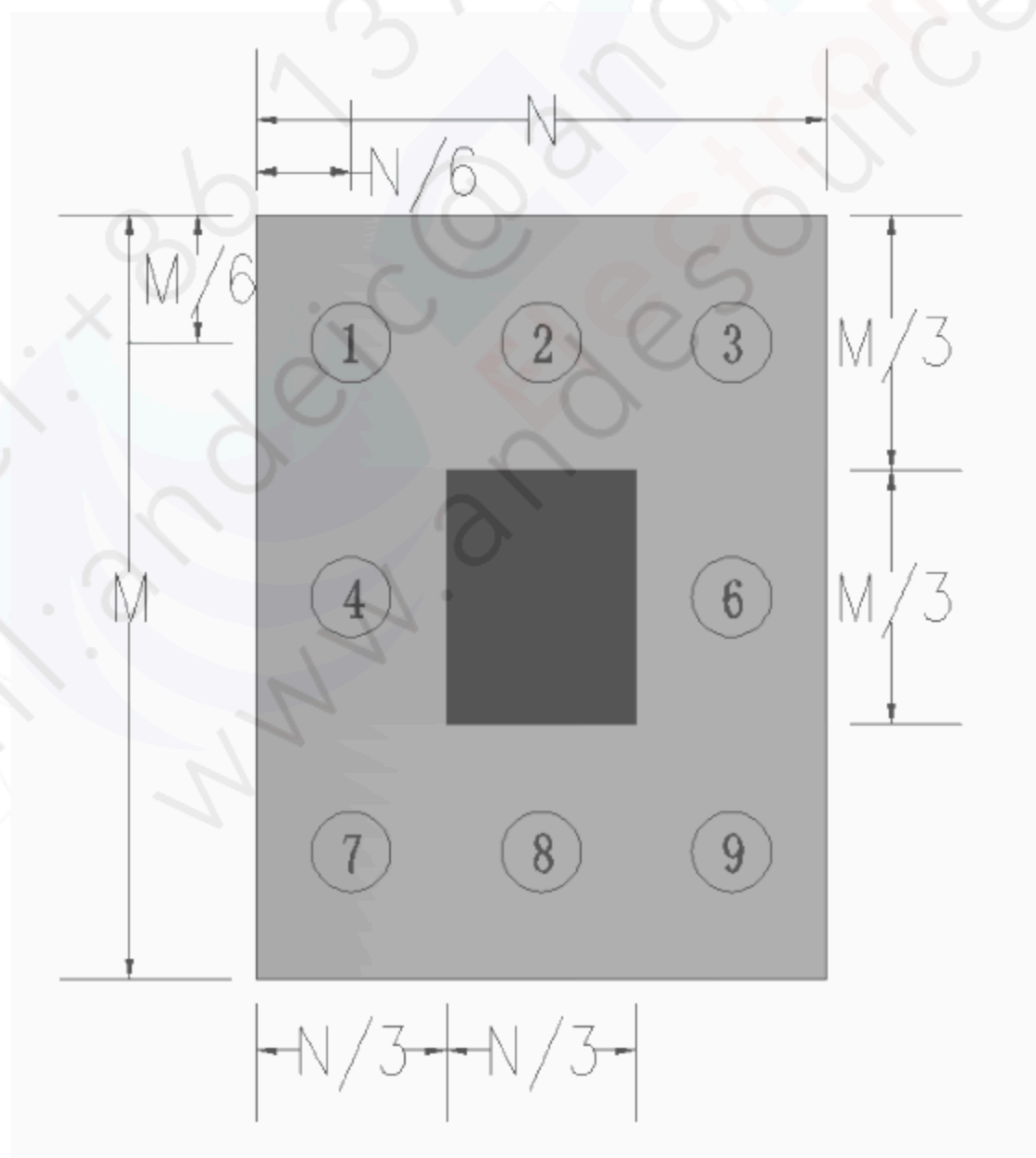
Cross-talk Test Pattern
