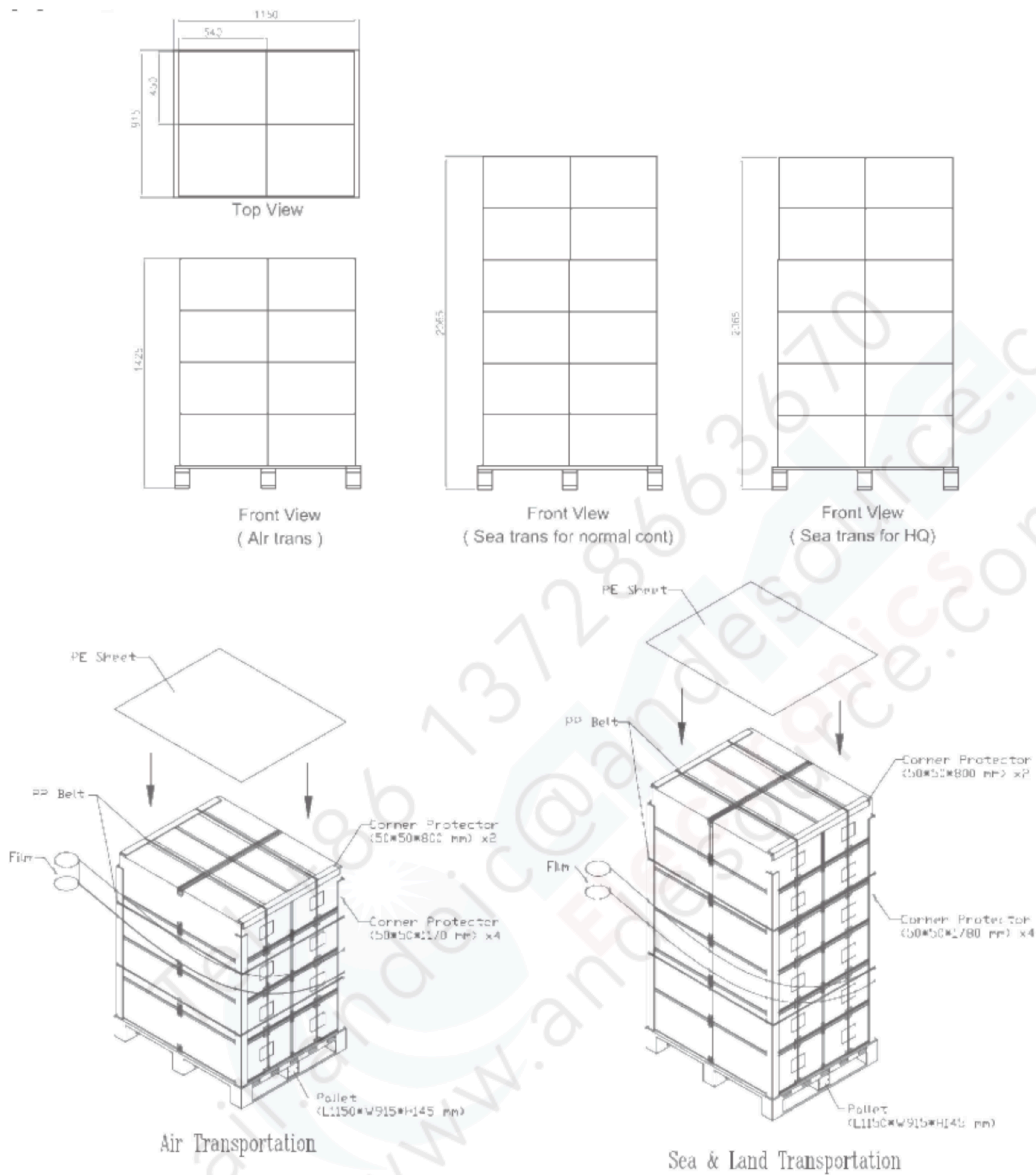
Figure. 7-3 Packing method
