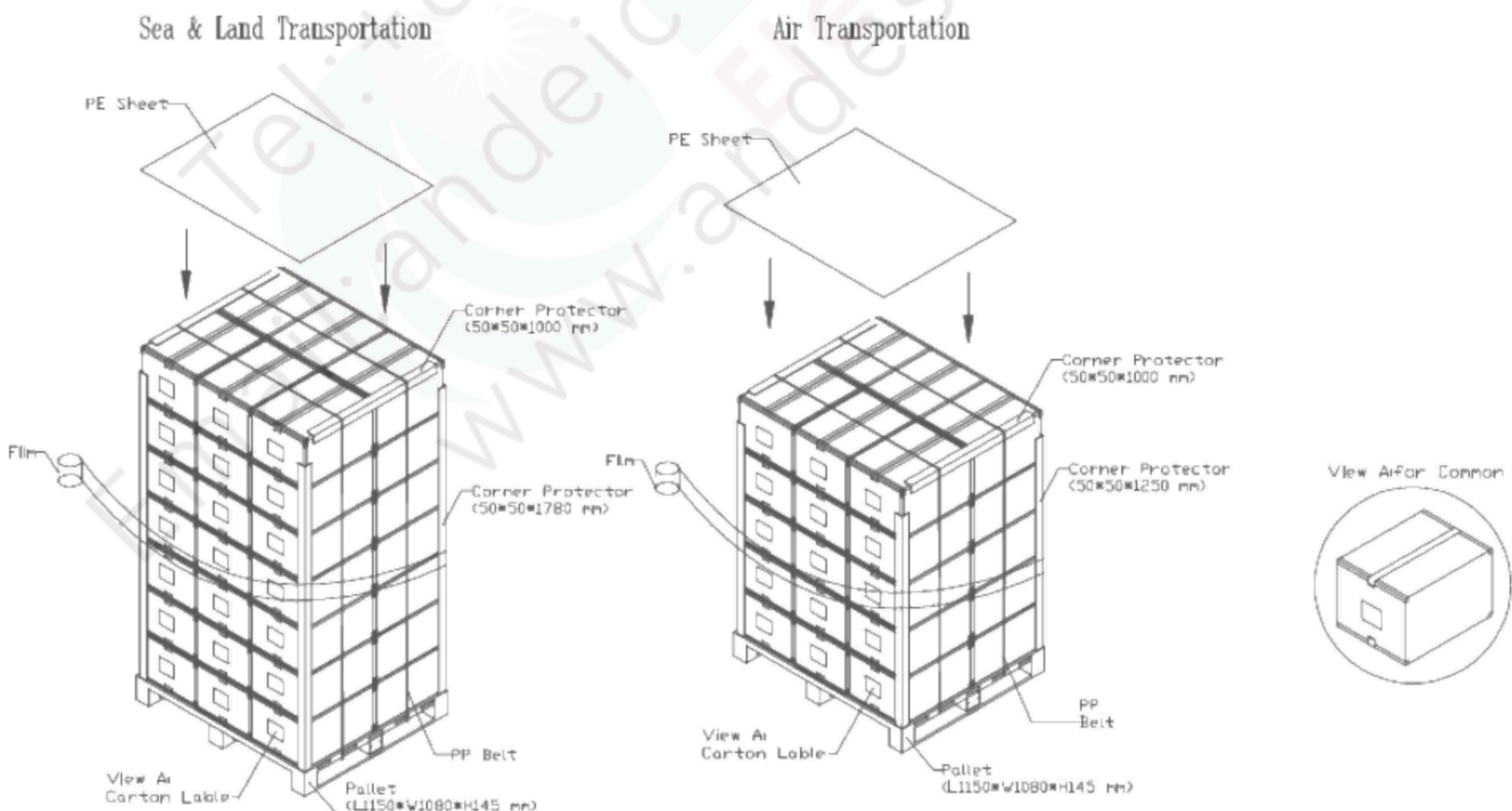
Figure. 7-3 Packing method
