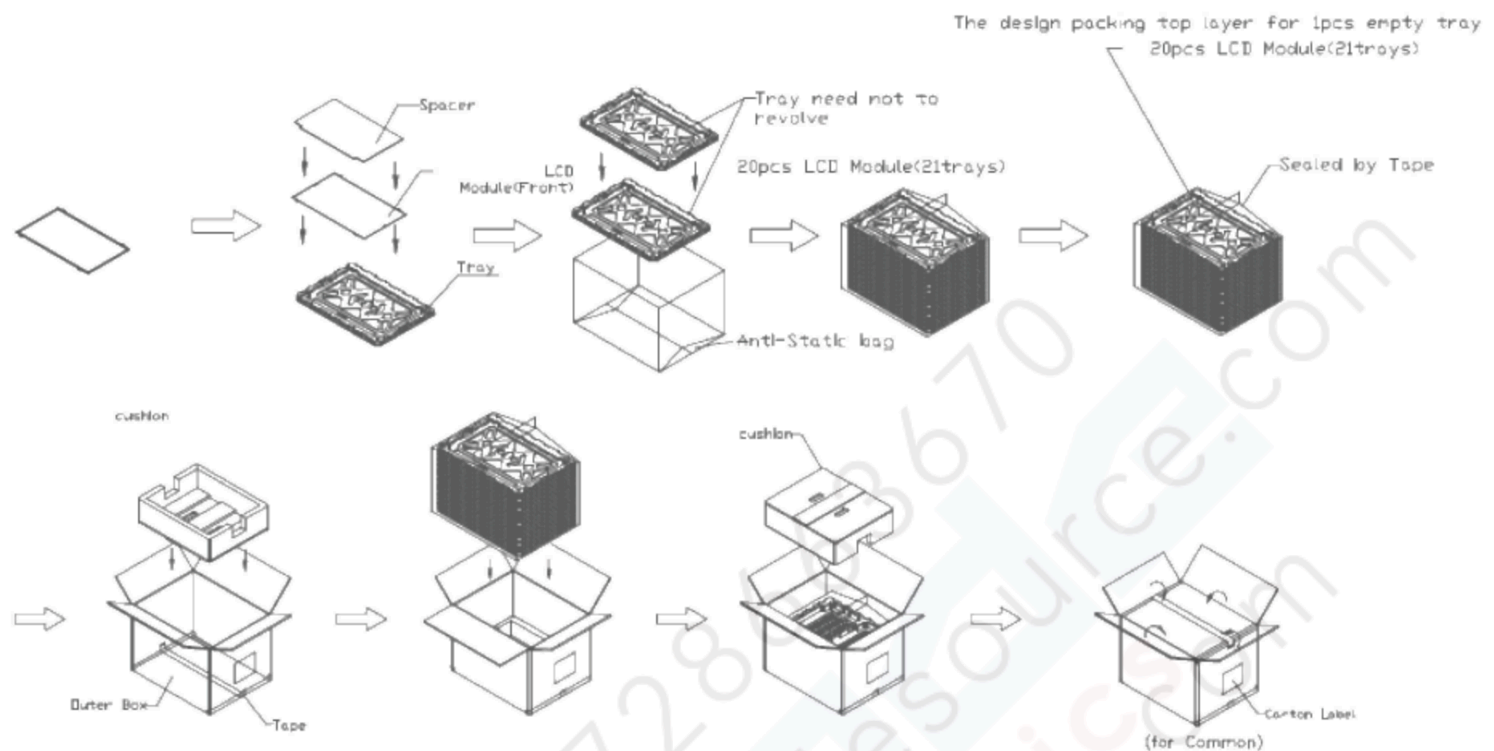
Figure. 7-2 Packing method
