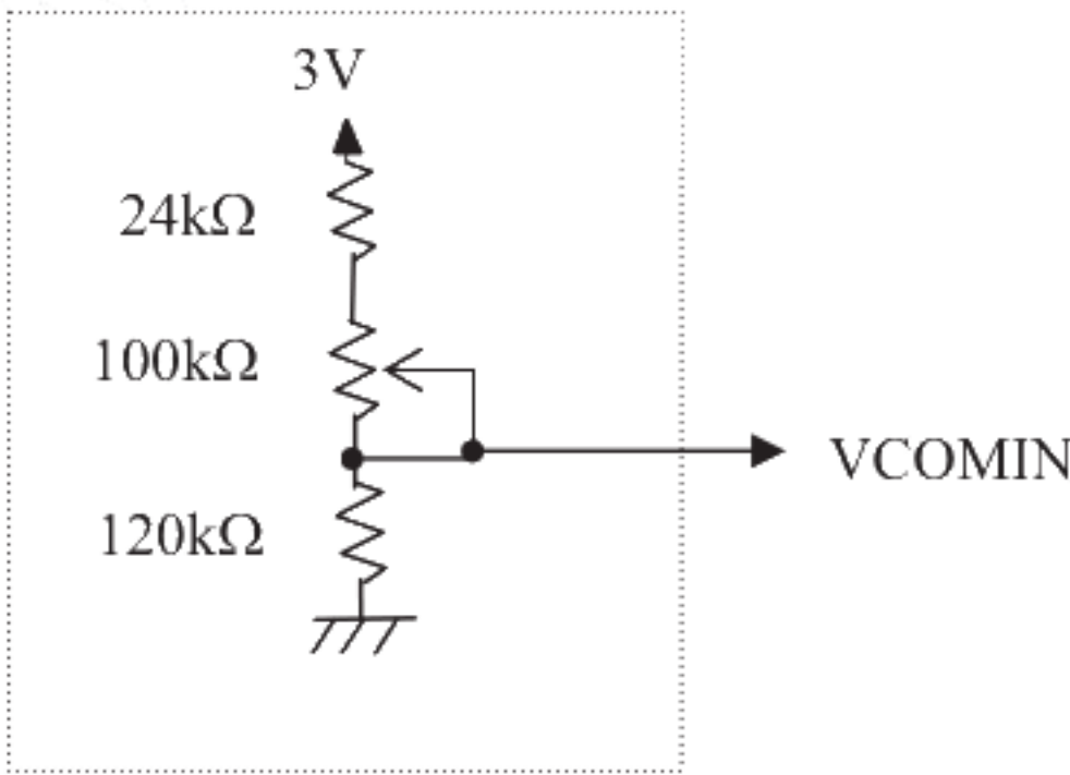
Reference design of COM circuit
