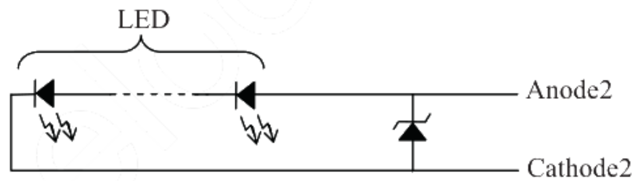
Circuits of backlight
