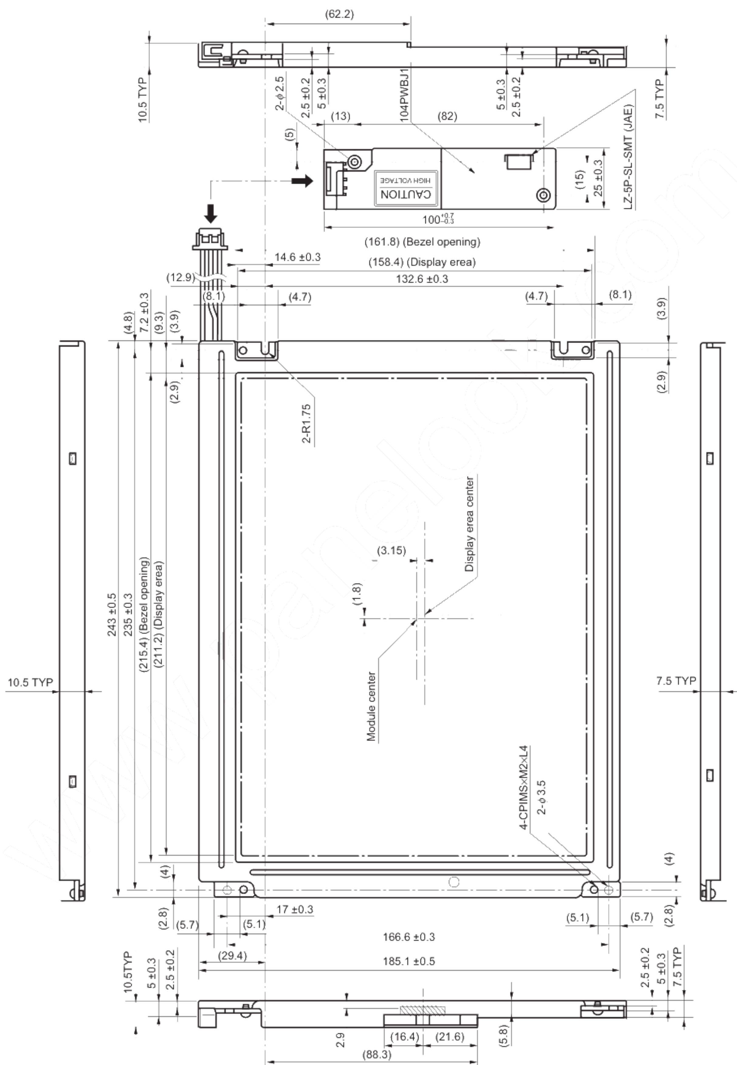
OUTLINE DRAWING: Front View (Unit in mm)
