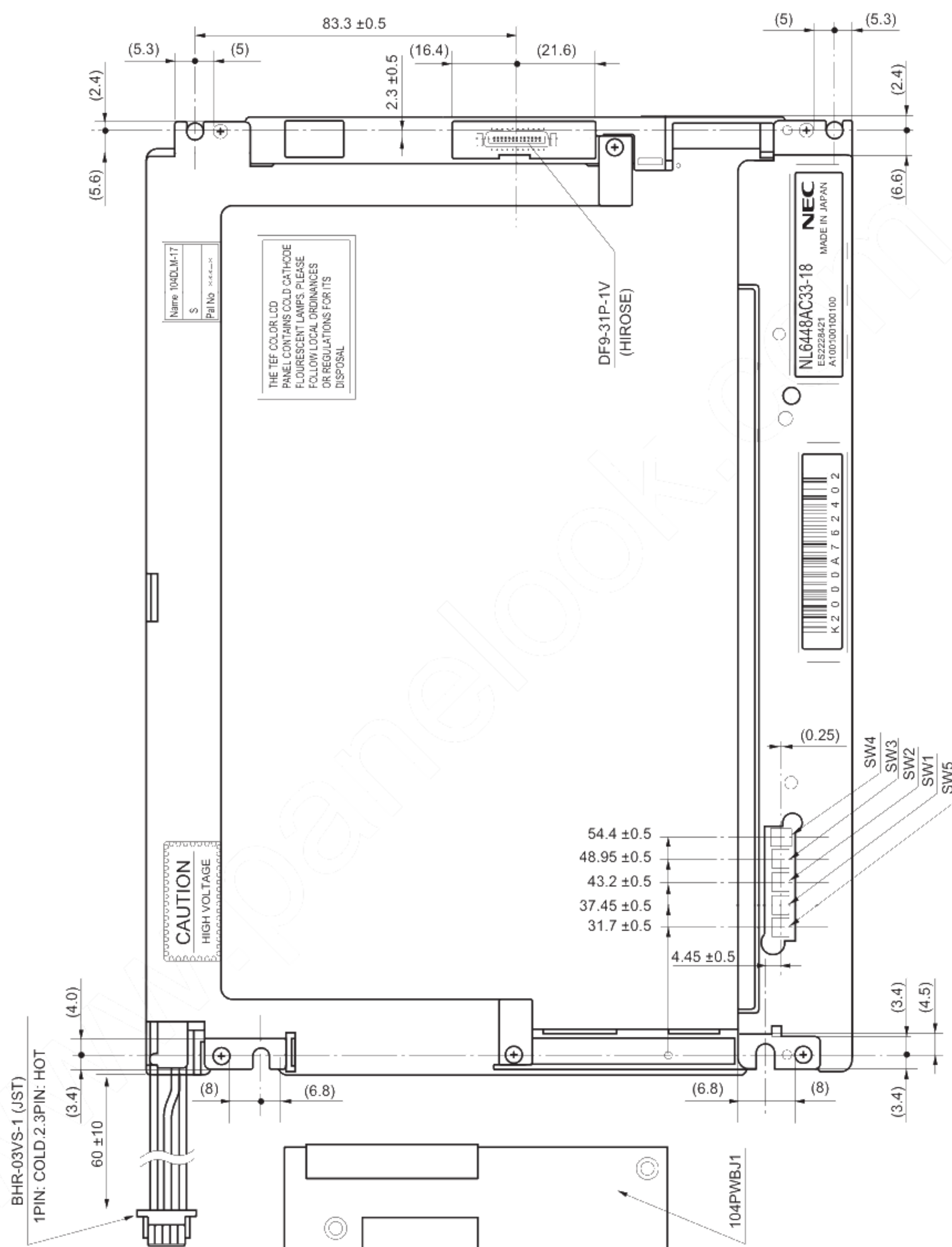
OUTLINE DRAWING: Rear View (Unit in mm)
