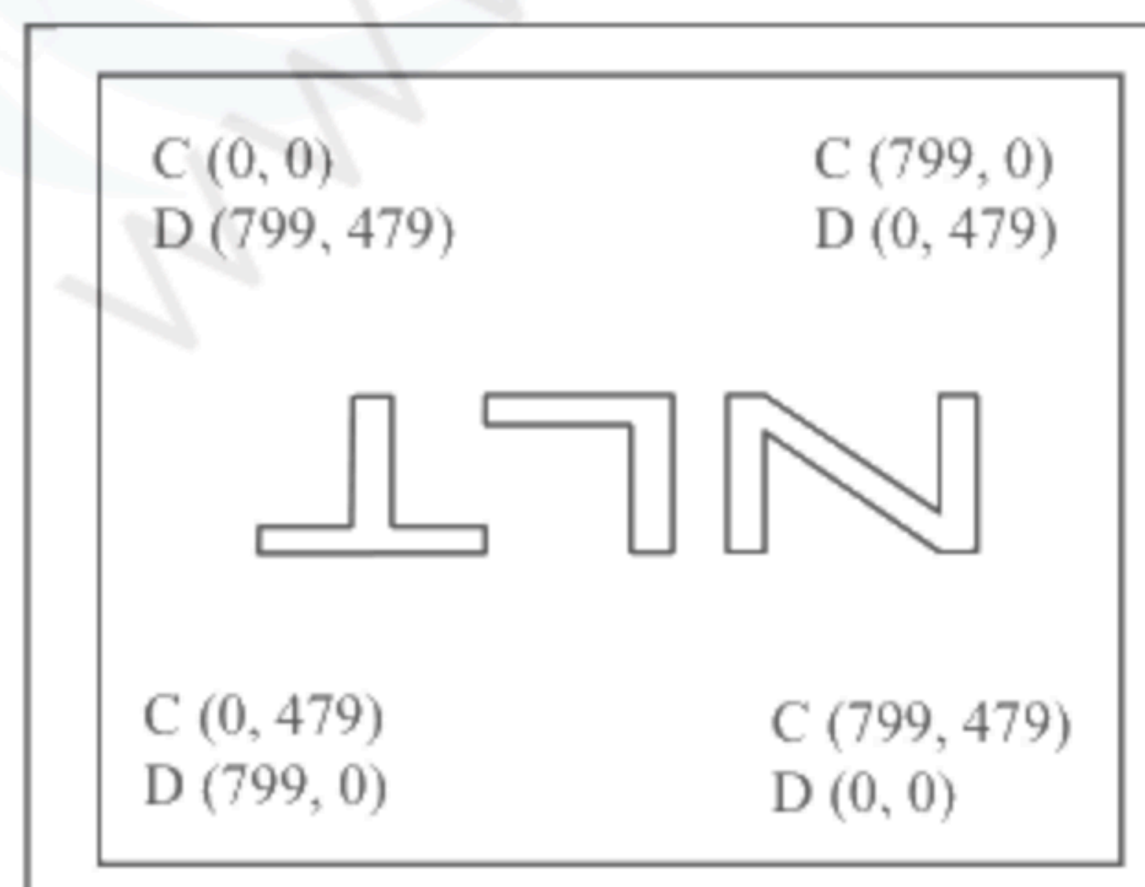
Figure2. Reverse scan (DPS: High)
