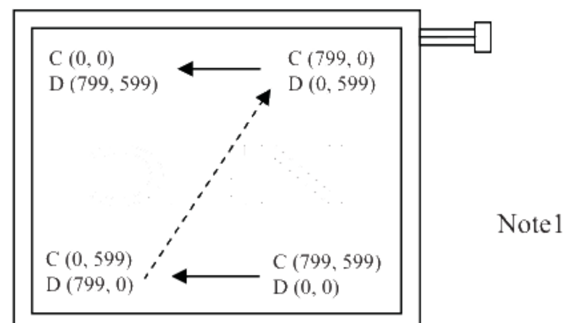
Figure 2. Reverse scan (DPS: Low or Open)
