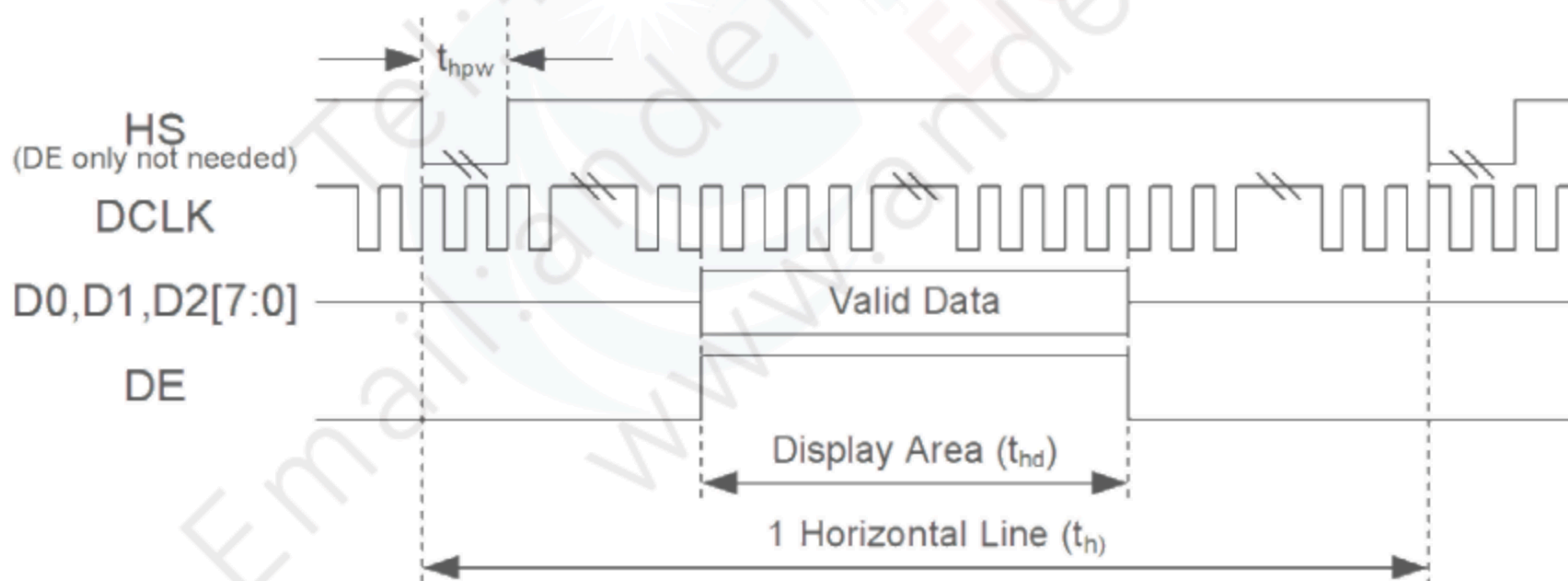
Figure 6.4.1 Horizontal input timing at DE only mode
