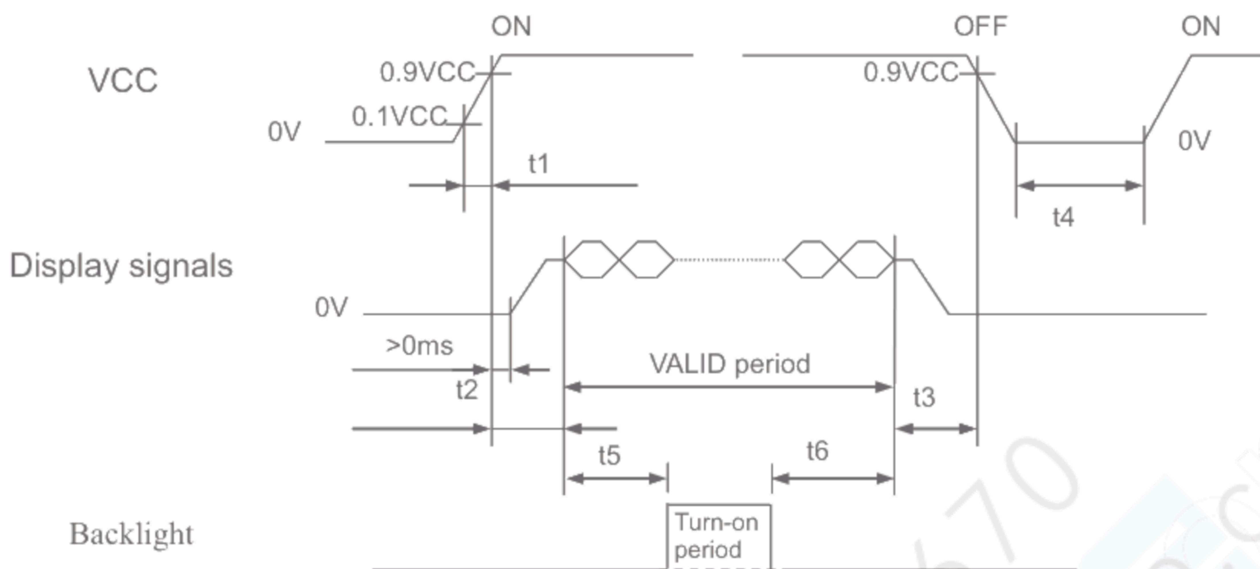
Figure 5.3 Power on/off sequence
