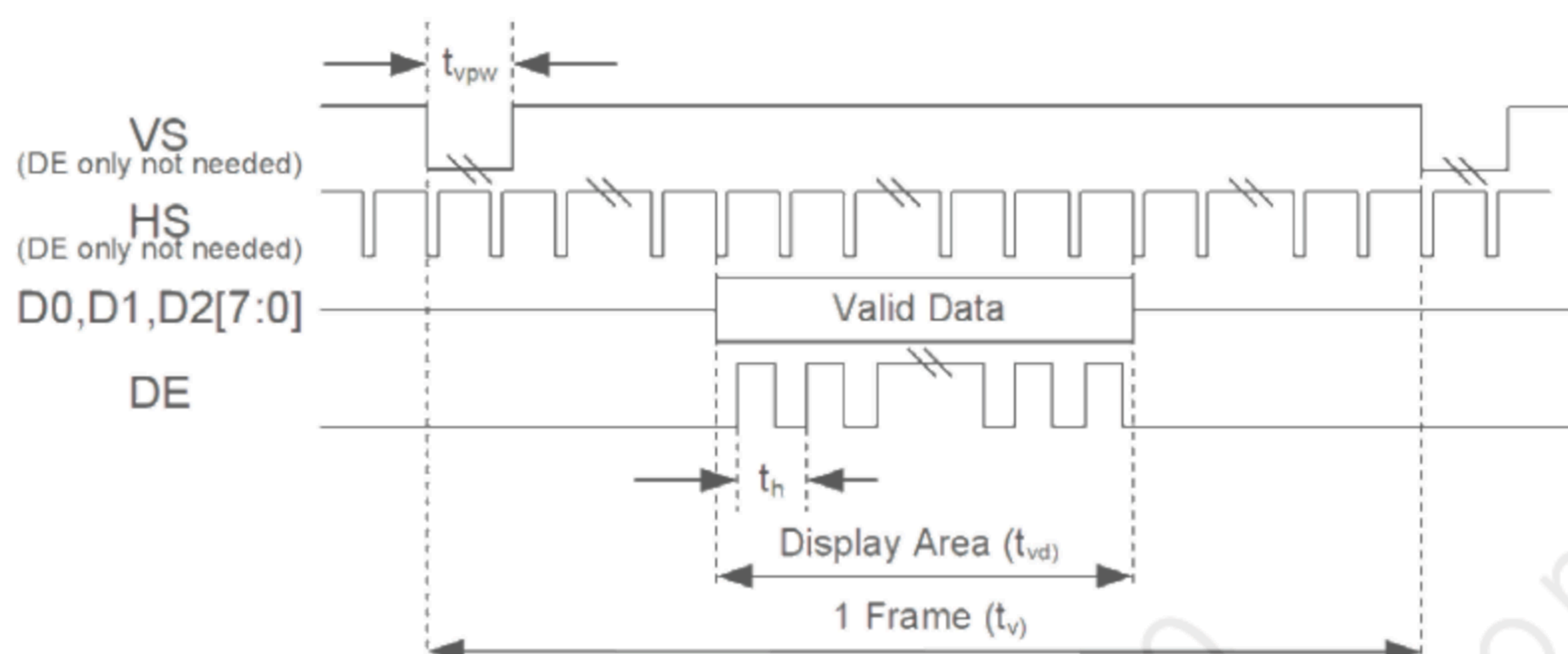
Figure 6.4.2 Vertical input timing at DE only mode
