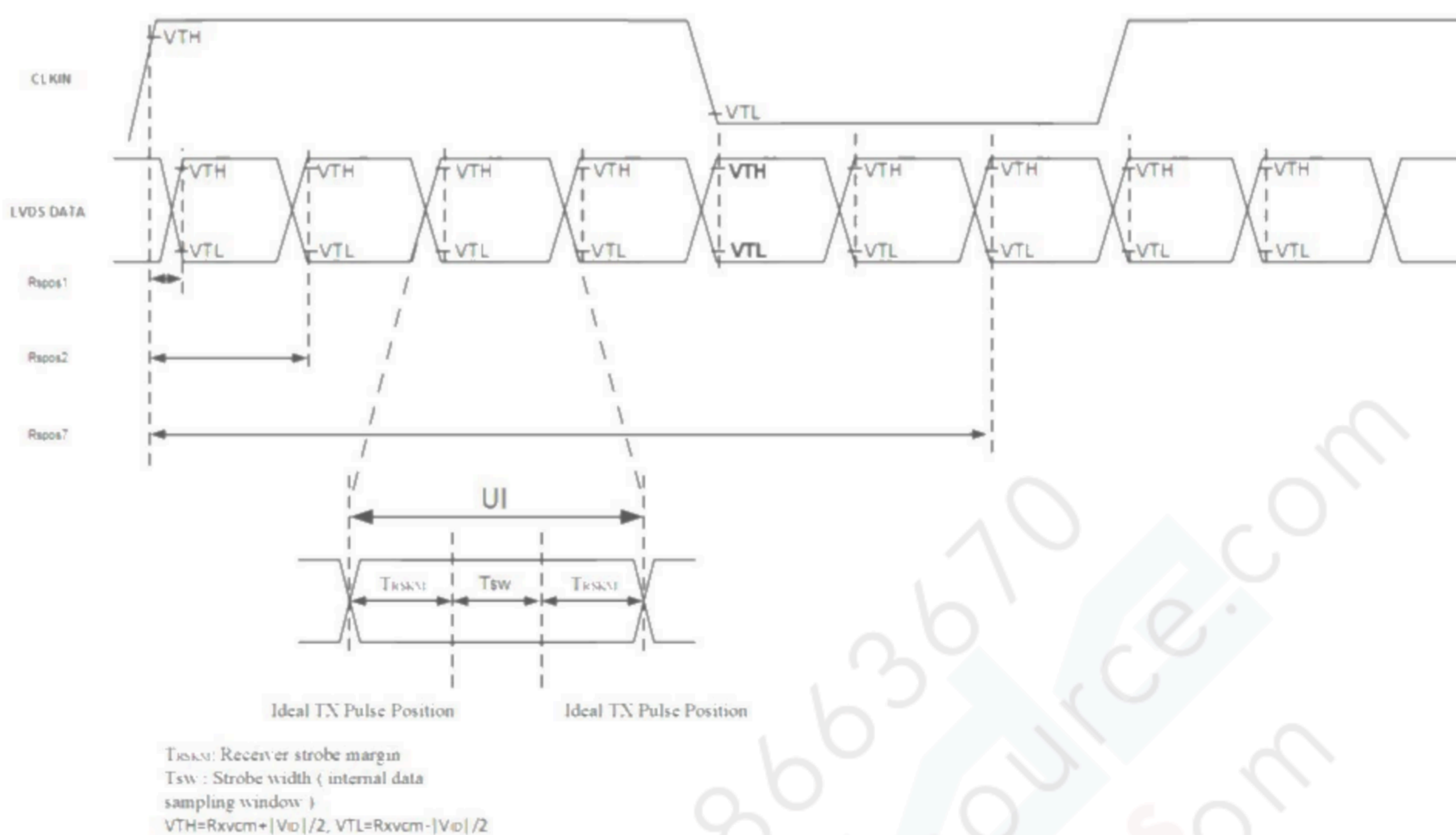
Figure 5.2.2 LVDS mode AC electrical characteristics 2
