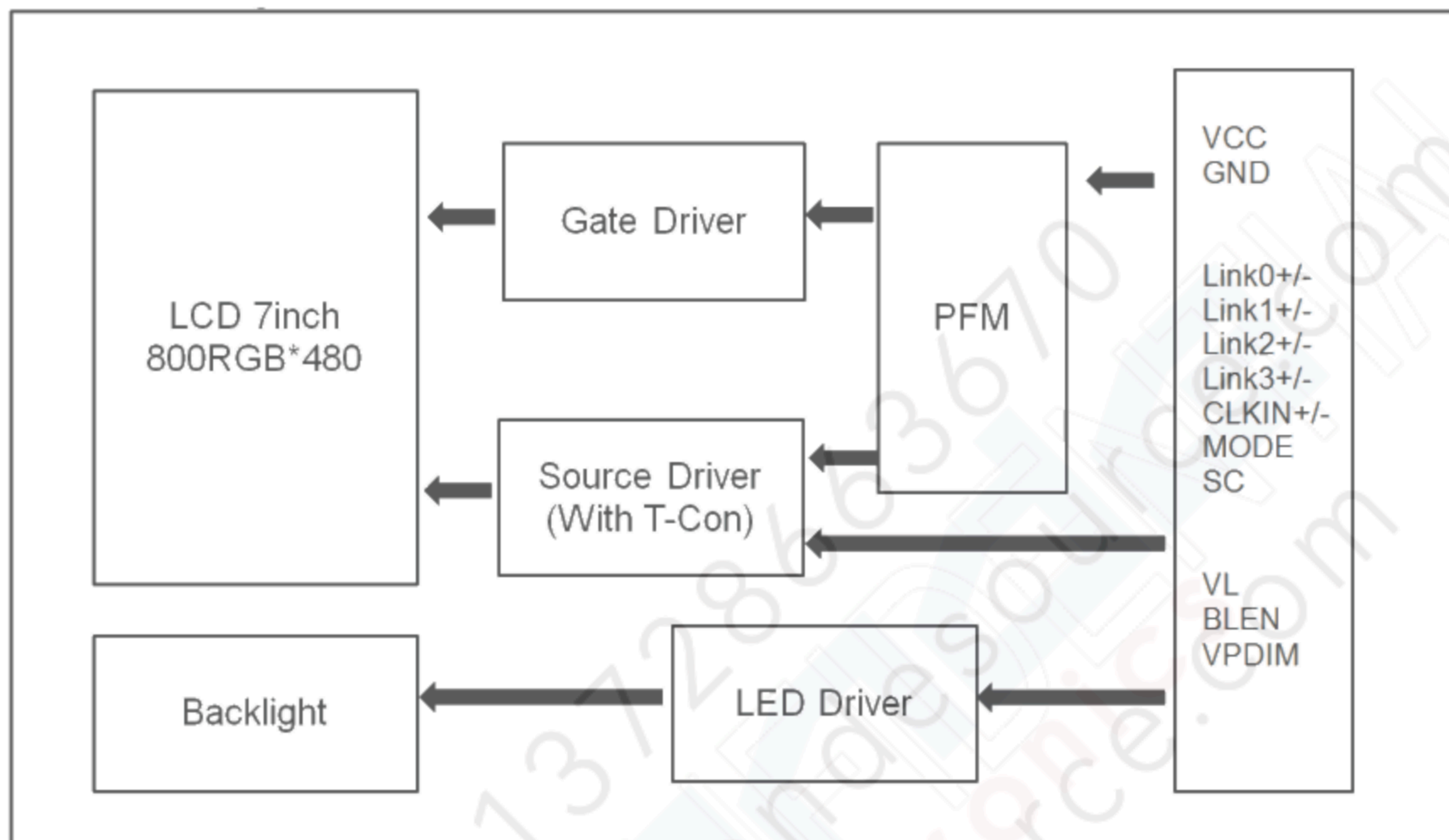
Figure 5.5 Block Diagram
