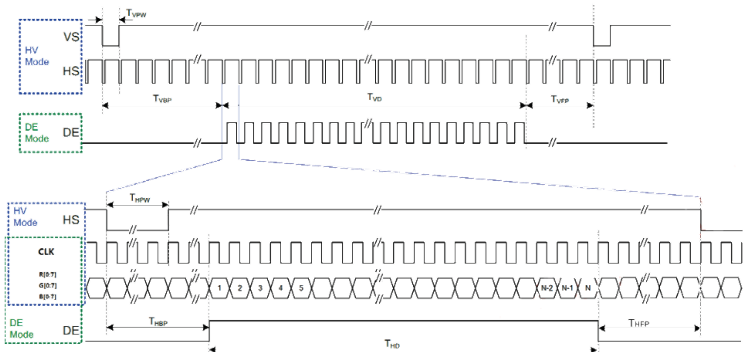
Figure 5.3 Recommended input timing of LVDS transmitter
