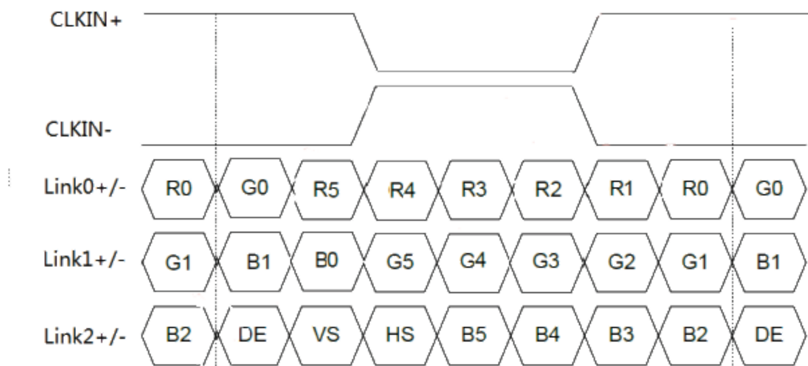
Figure 5.1.2 LVDS data map
