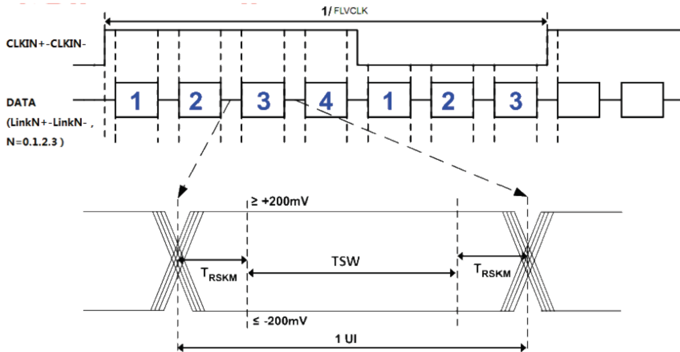
Figure 5.4.1 LVDS Data Skew
