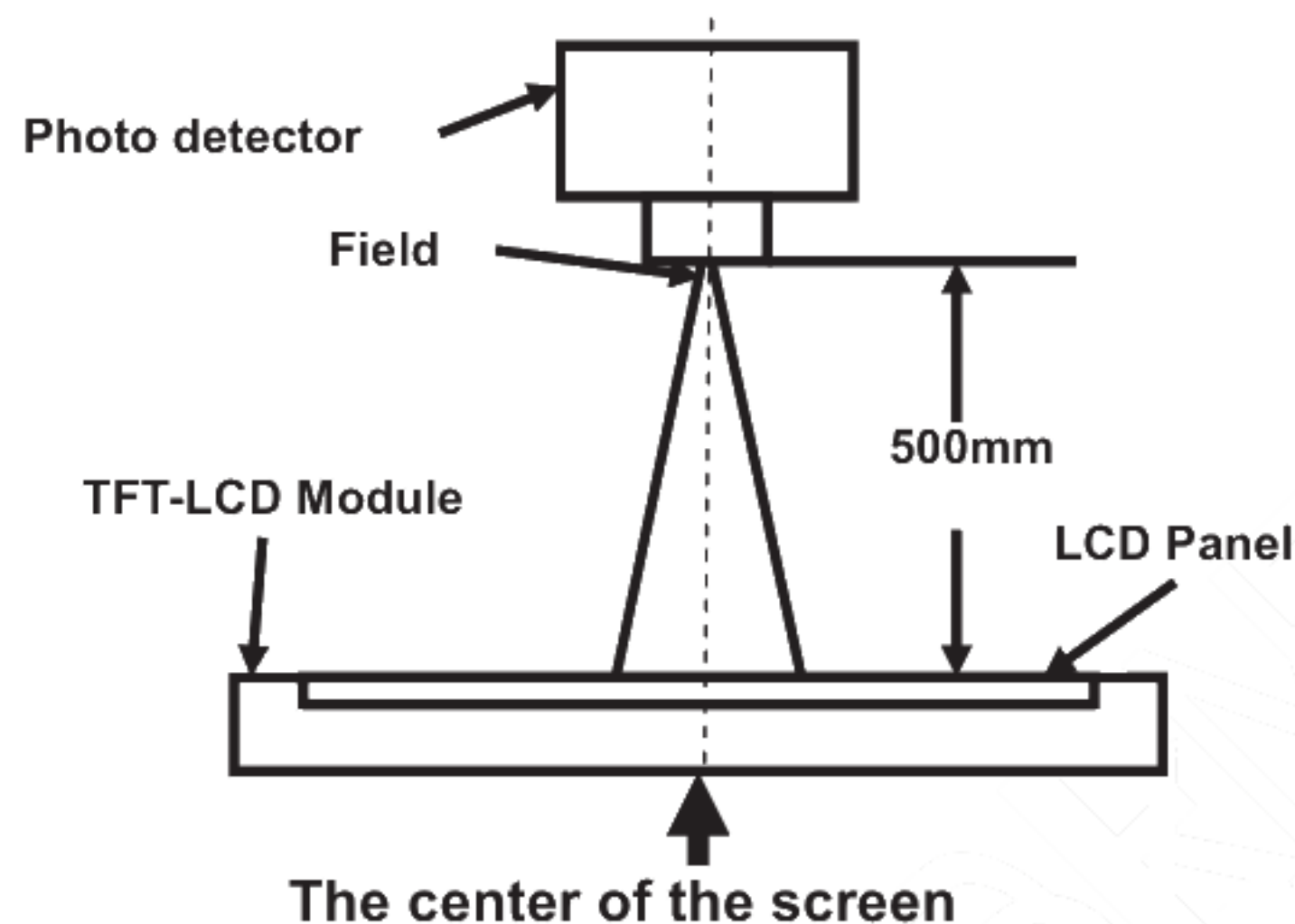
Figure 6.1 Definition of optical measurement system
