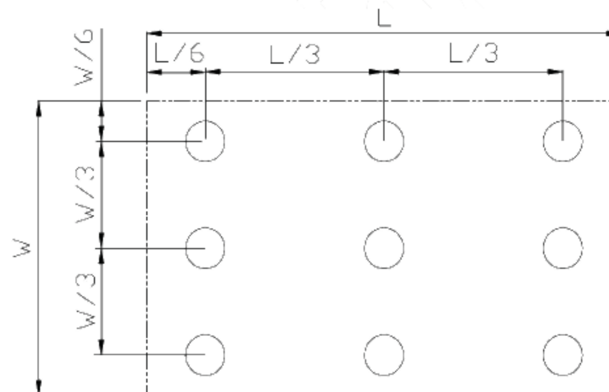
Figure 6.3 Definition of uniformity
