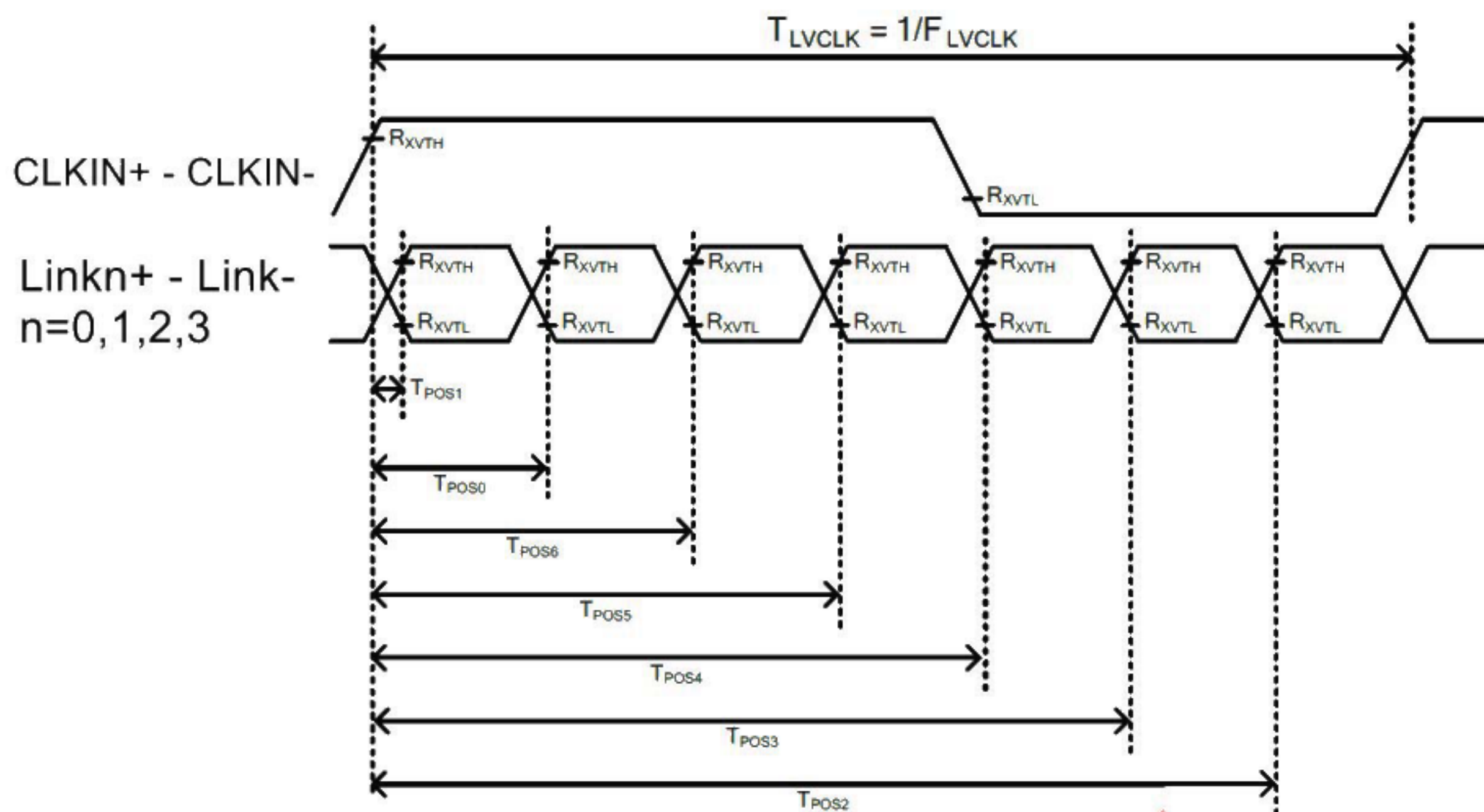
Figure 5.4.2 LVDS input timing
