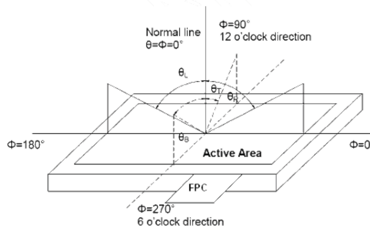
Figure 6.2 Definition of viewing angle
