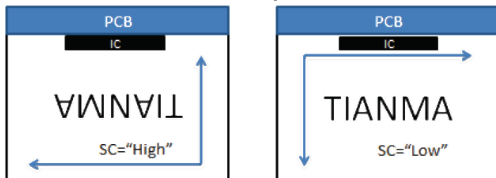
Figure2.1 Scanning diagram
