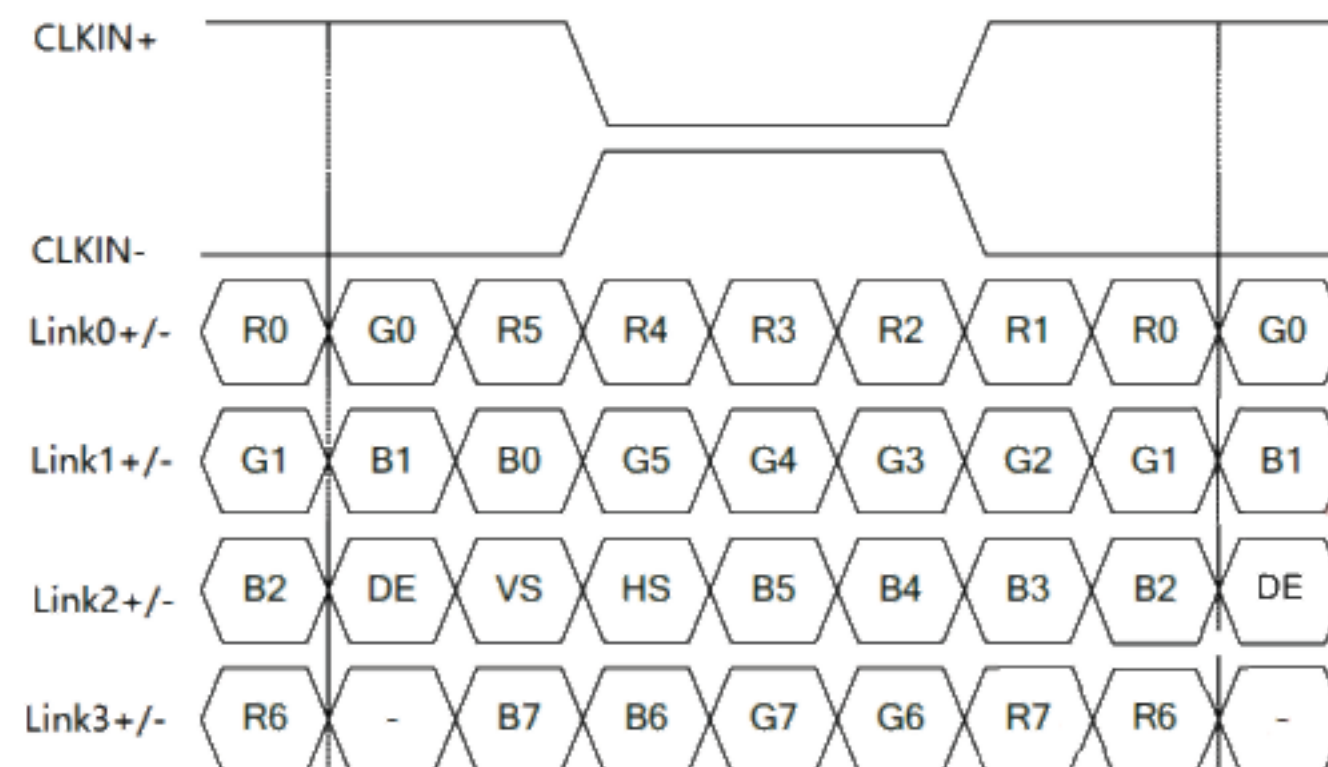
Figure 5.1.1 8-bit LVDS data map
