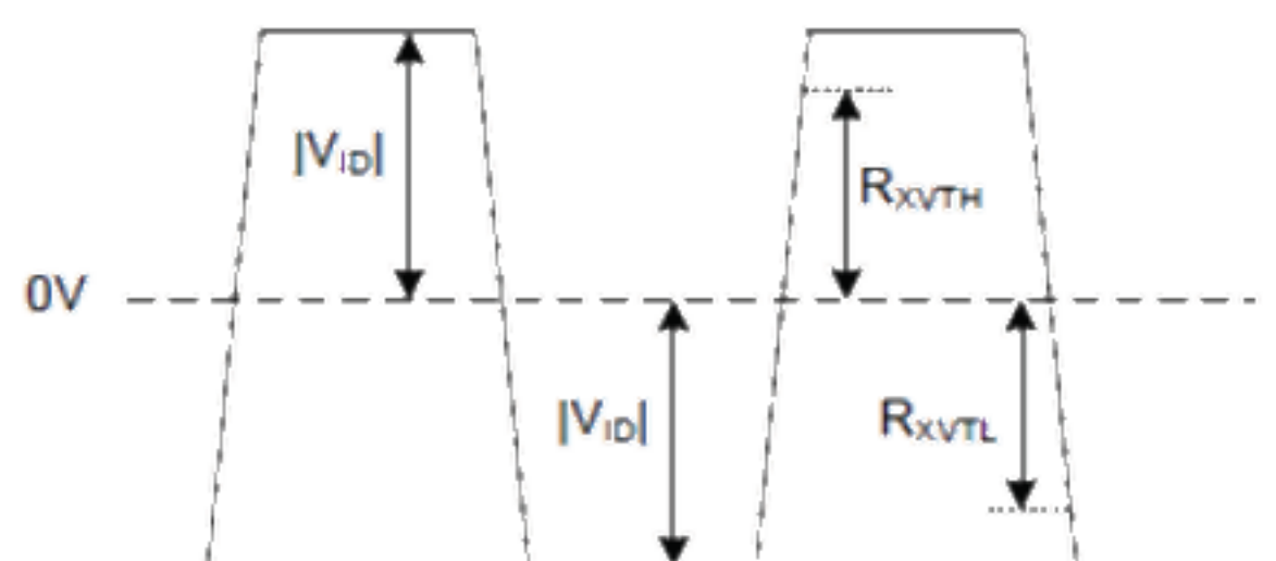
Figure4.1 LVDS DC Diagram
