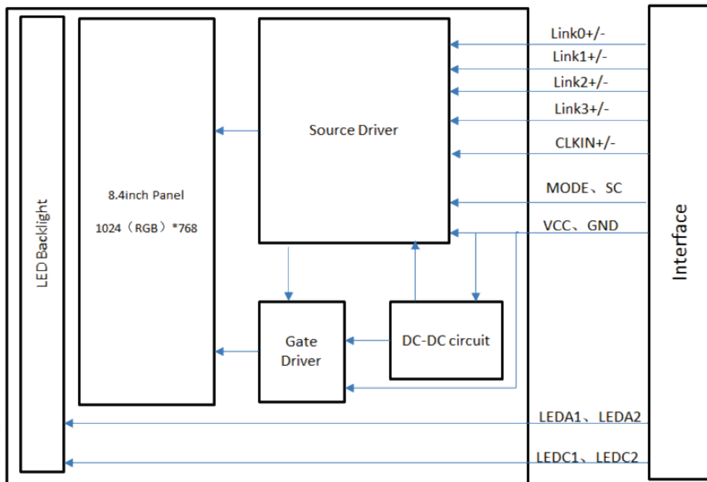
Figure 4.3 LCD Module Block Diagram
