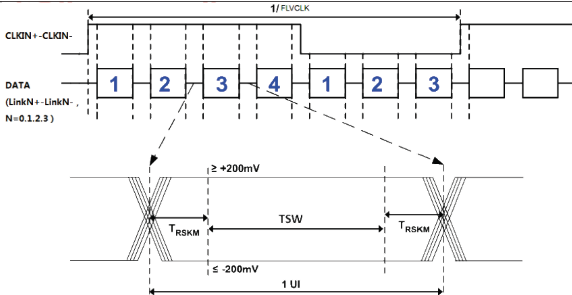
Figure 5.4.1 LVDS Data Skew
