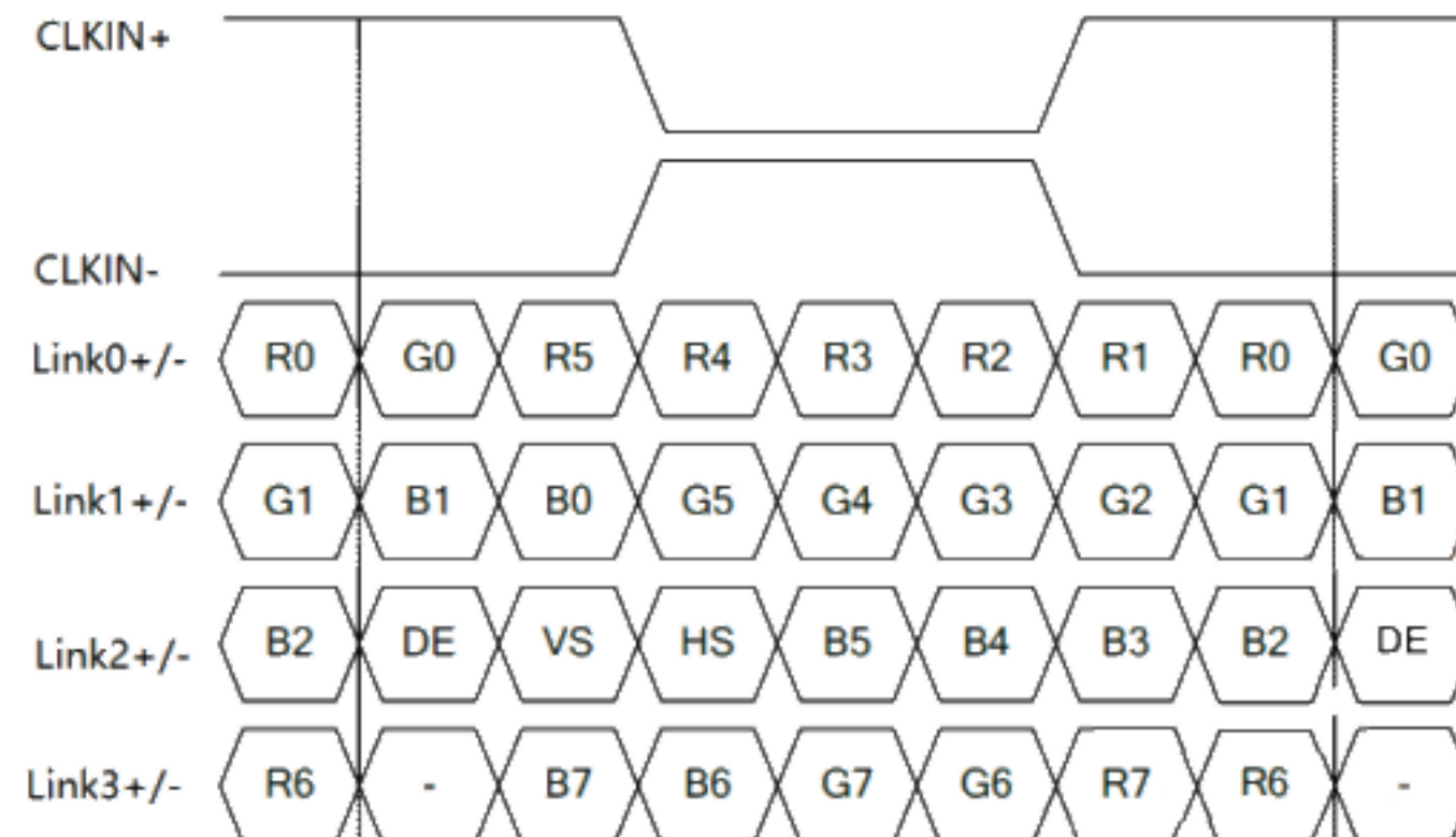
Figure 5.1.1 LVDS data map
