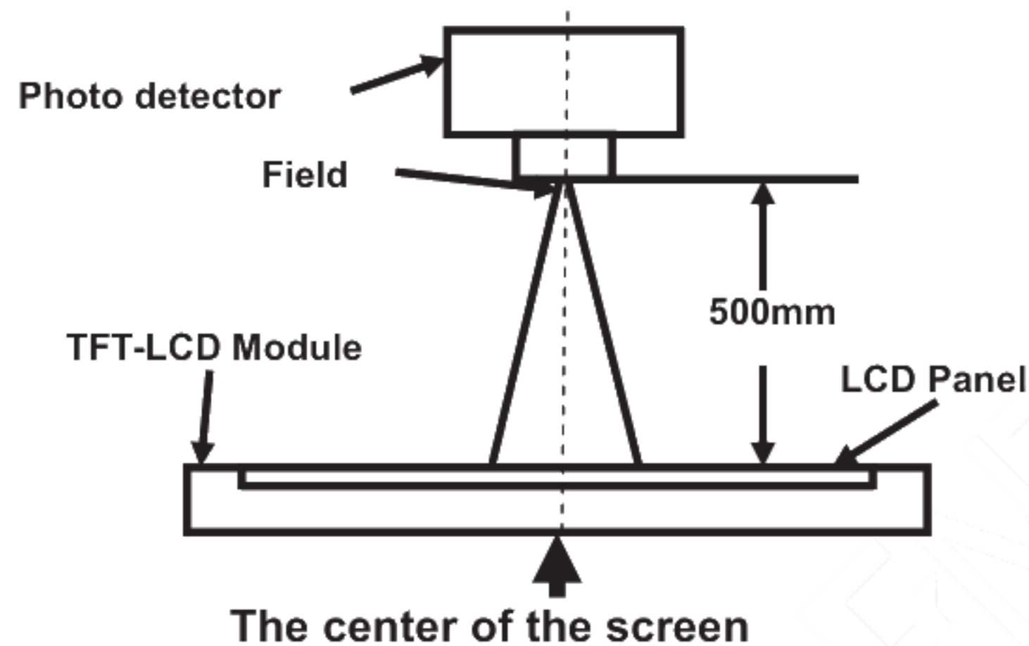
Figure 6.1 Definition of optical measurement system
