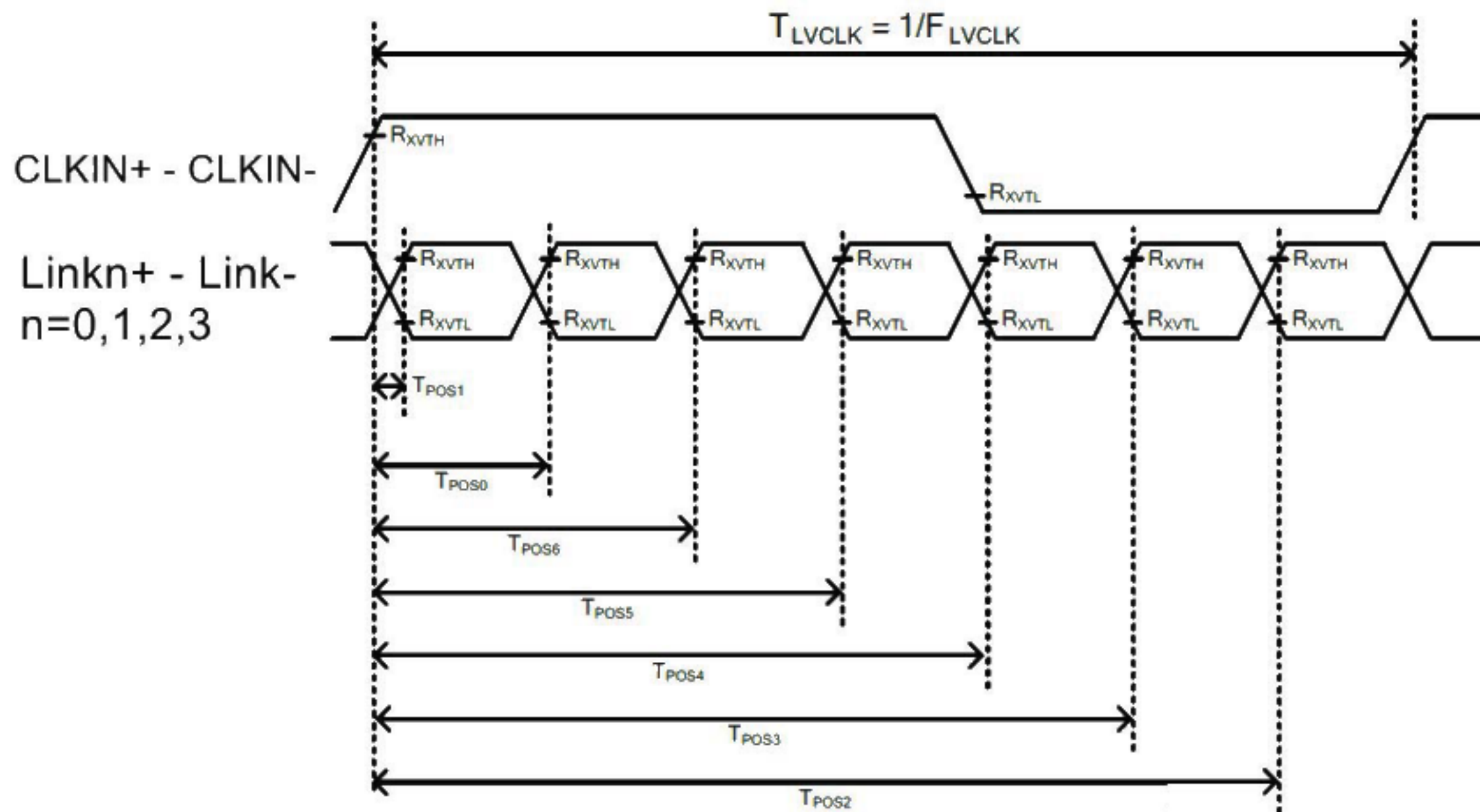
Figure 5.4.2 LVDS input timing
