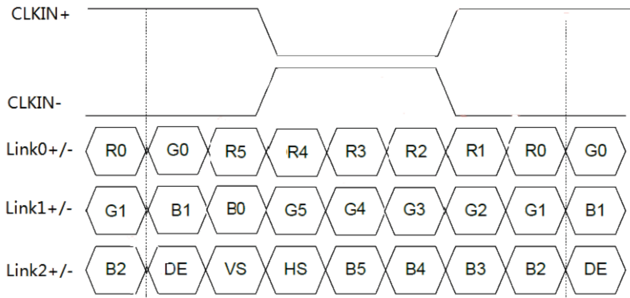
Figure5.1.1 LVDS data map
