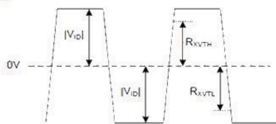
LVDS DC Diagram
