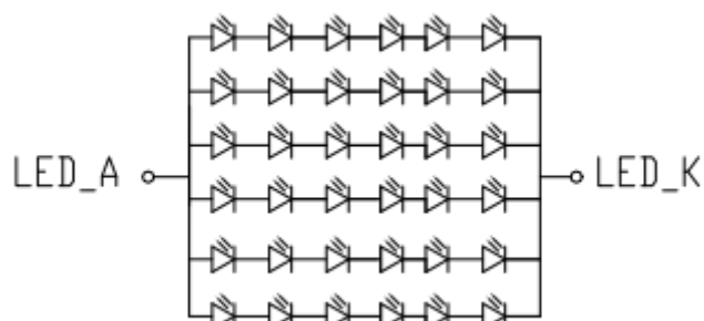
Figure 5.2 LED circuit
