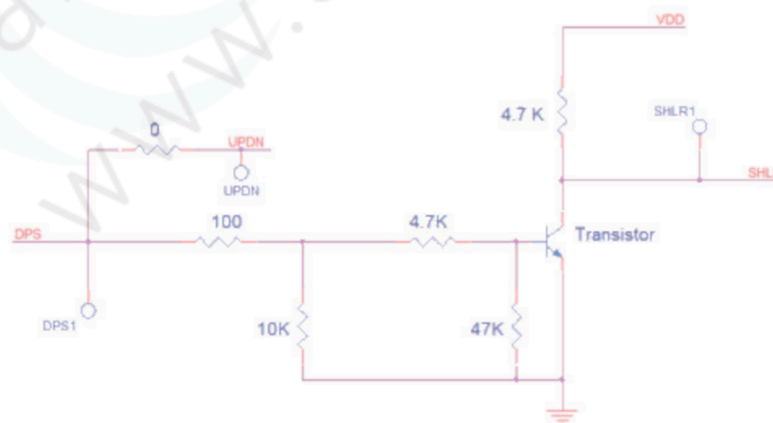
Figure 3.1.3 DPS Schematic
