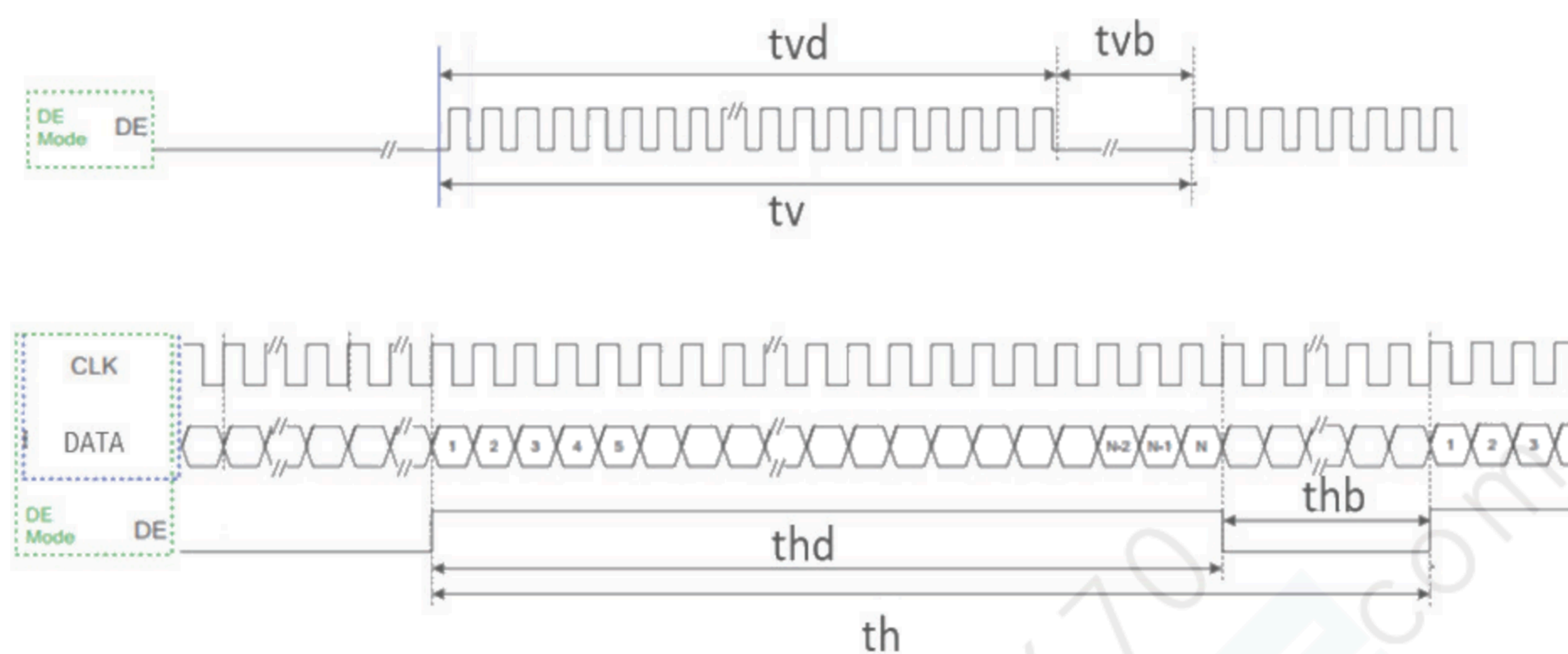
Figure 6.3.1 Clock and Data Input Timing Diagram
