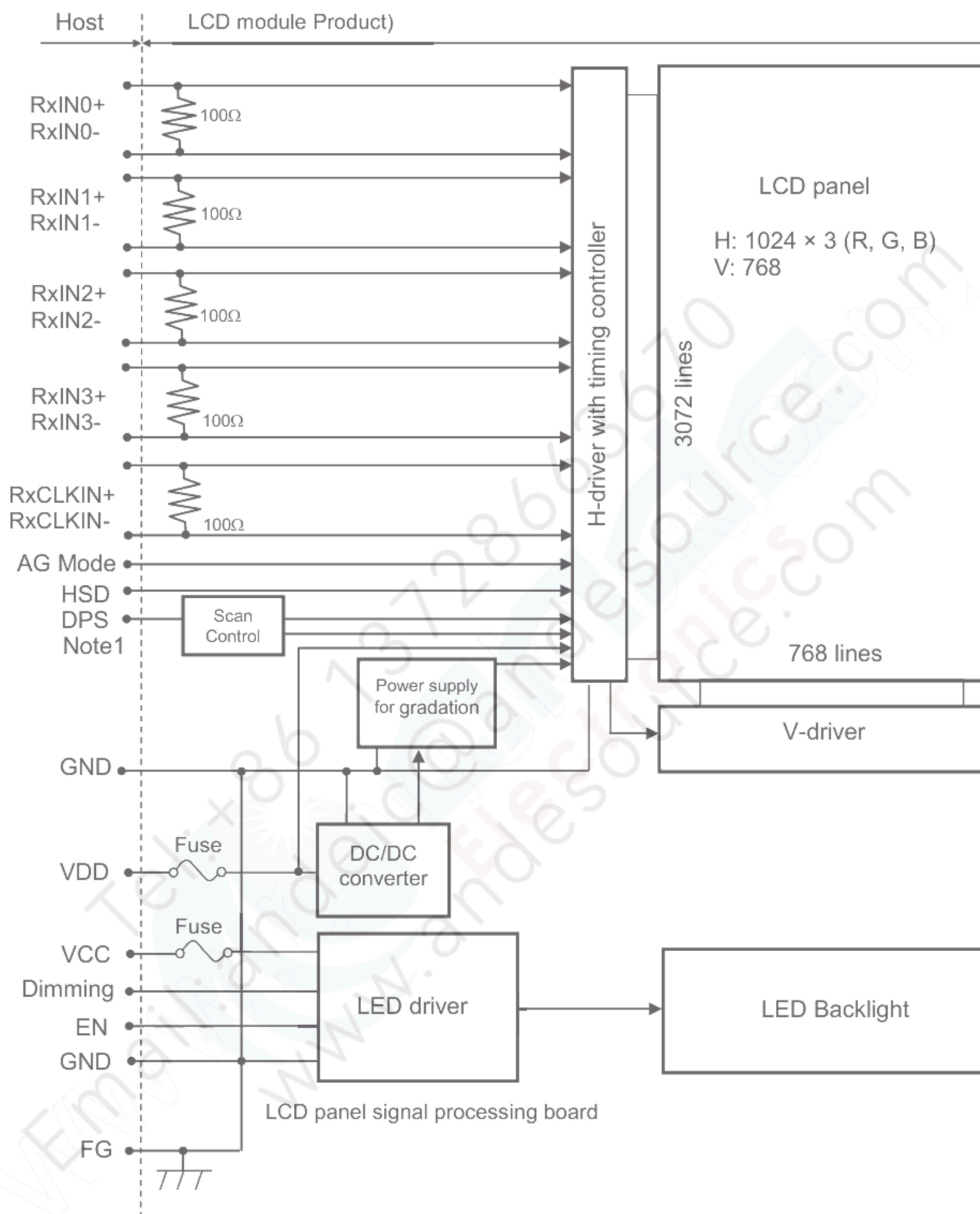
Figure 5.4.1 LCD Module Block Diagram
