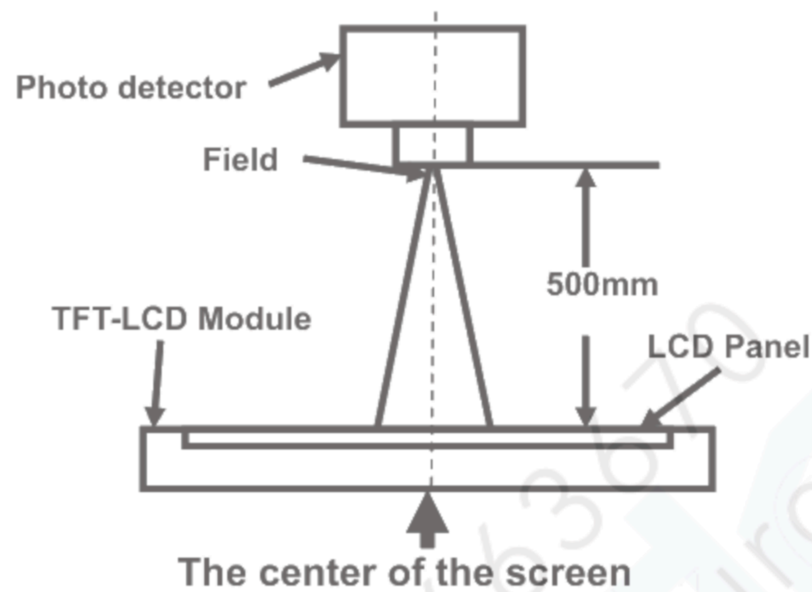
Fig1. Measurement Set Up
