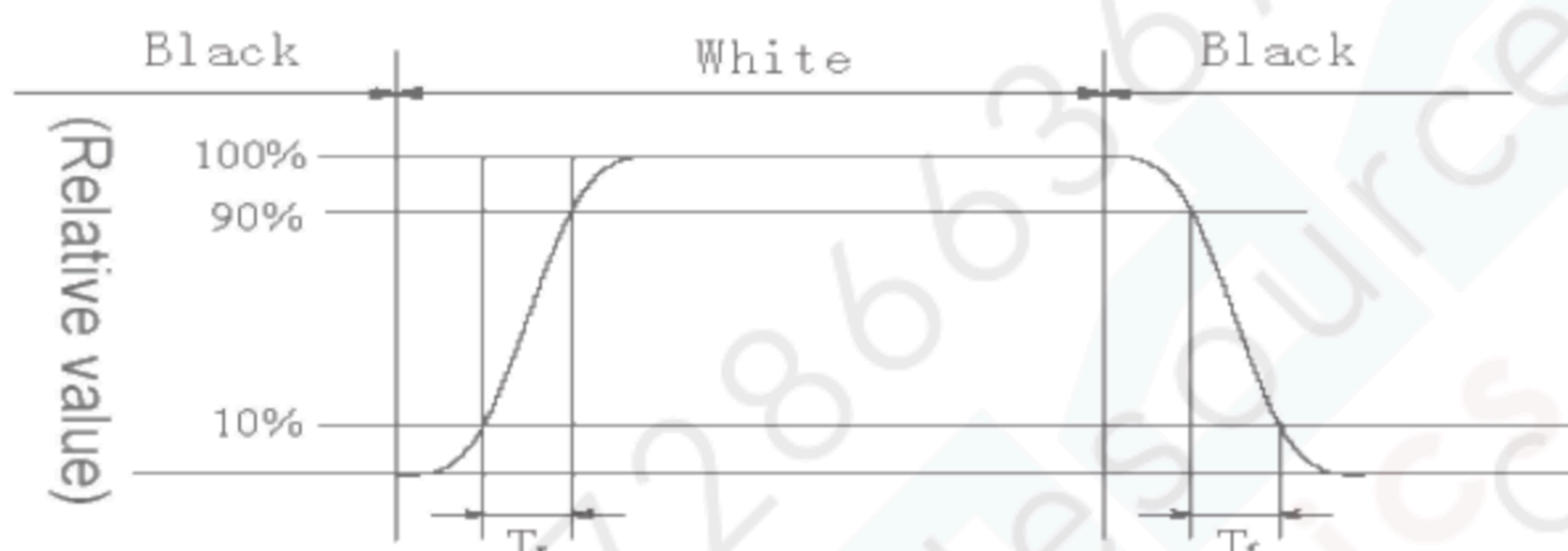
Fig4. Response Time Testing(SFT)
