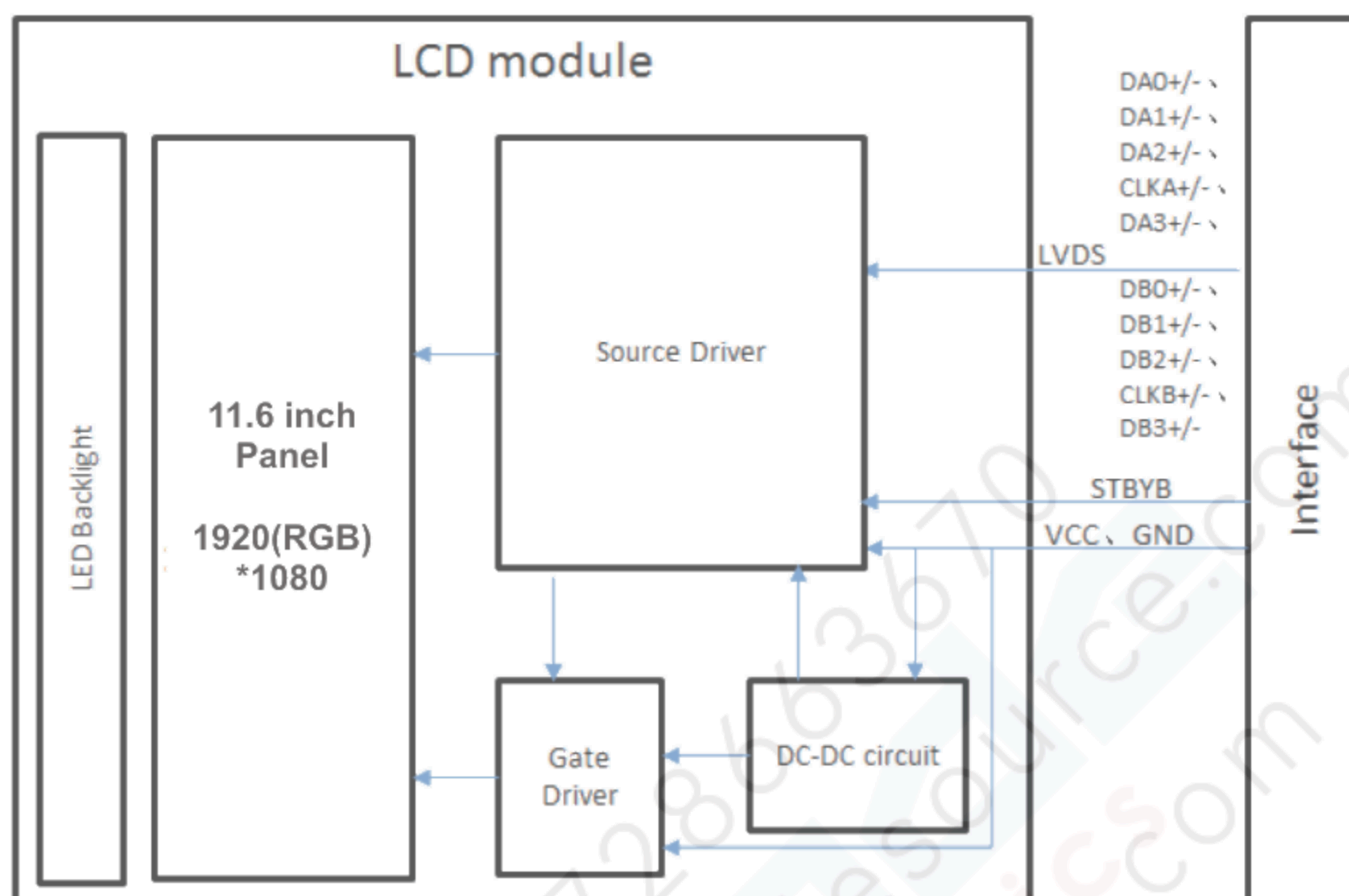
Figure 5.5.1 LCD Module Block Diagram
