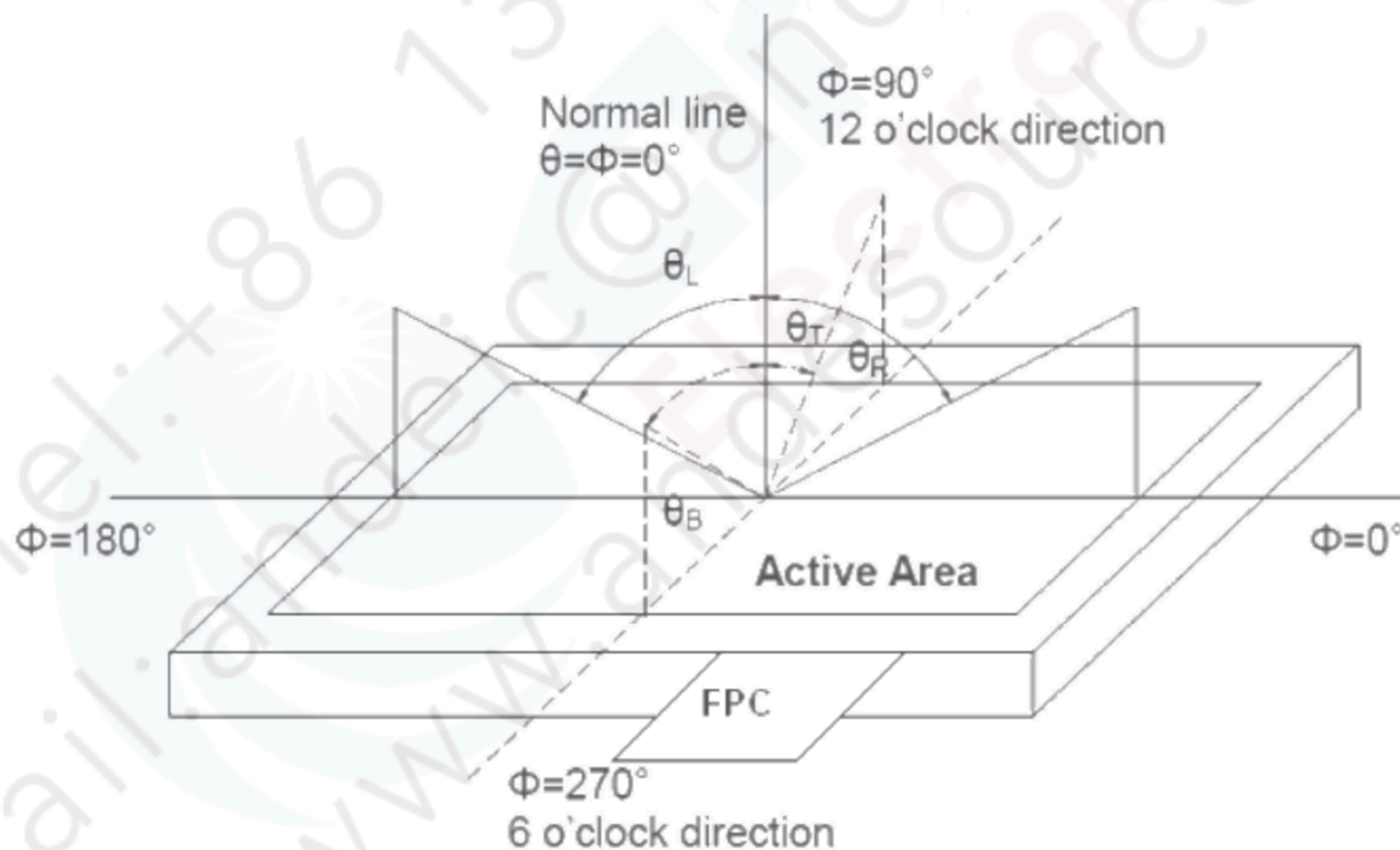
Fig2. Measurement viewing angle
