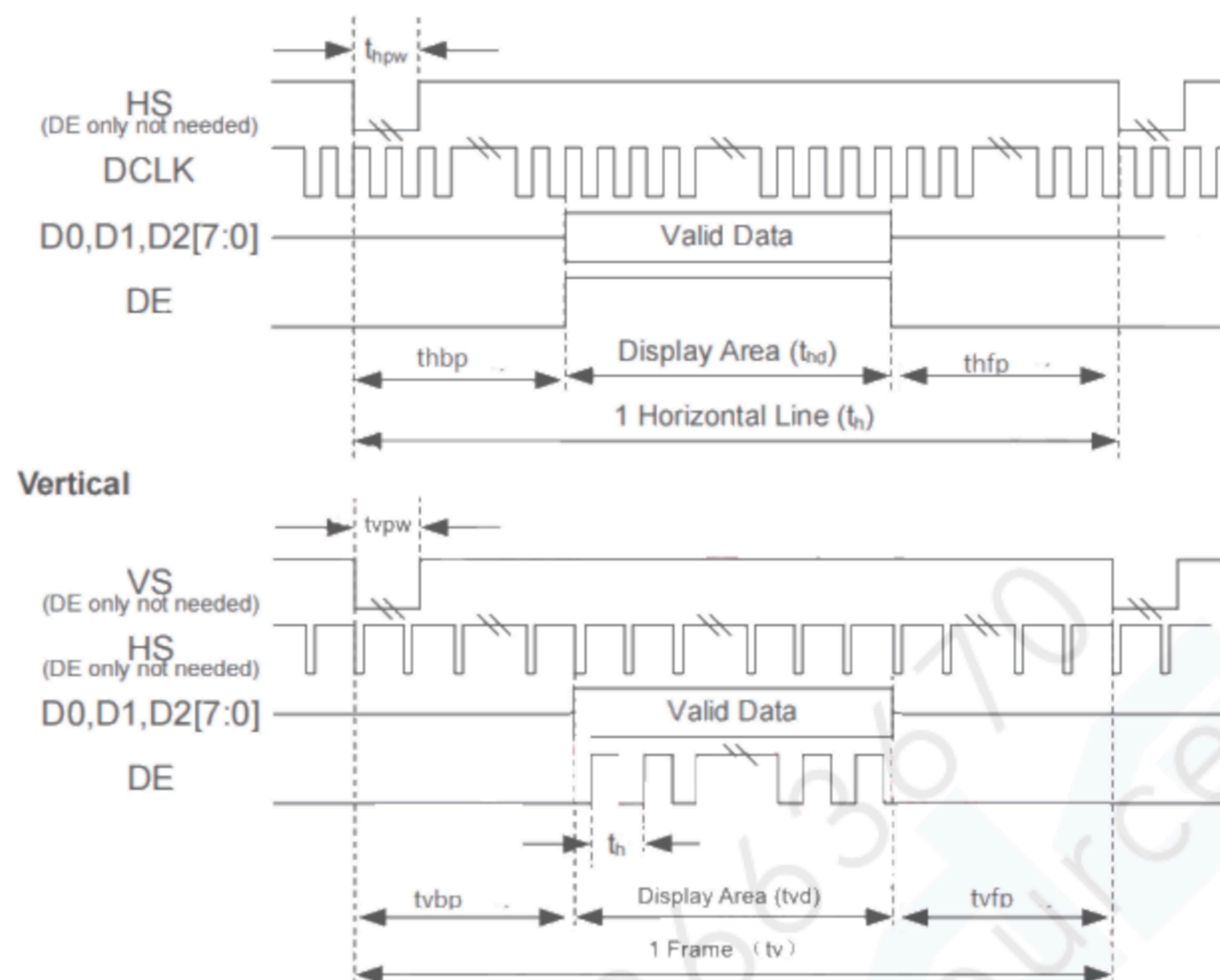
Figure 6.4.1 Data Input Timing Diagram Under DE Mode
