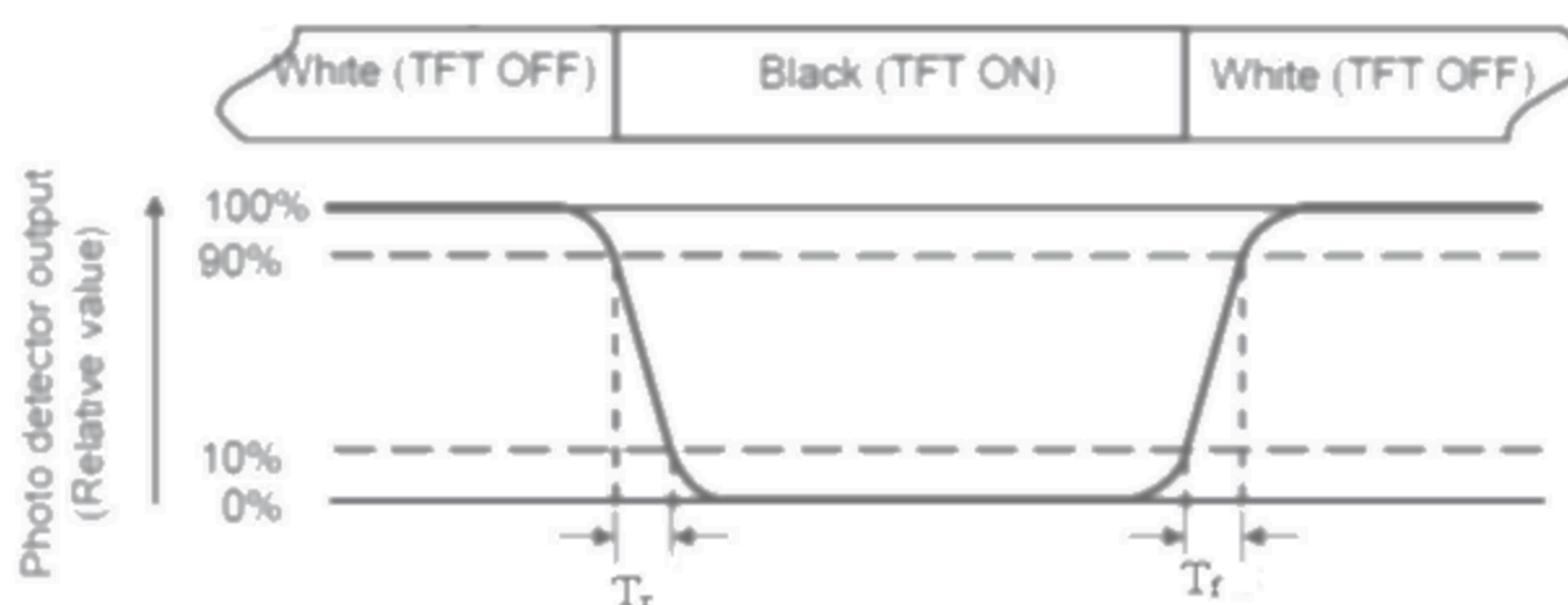
Fig3. Response Time Testing(TN)
