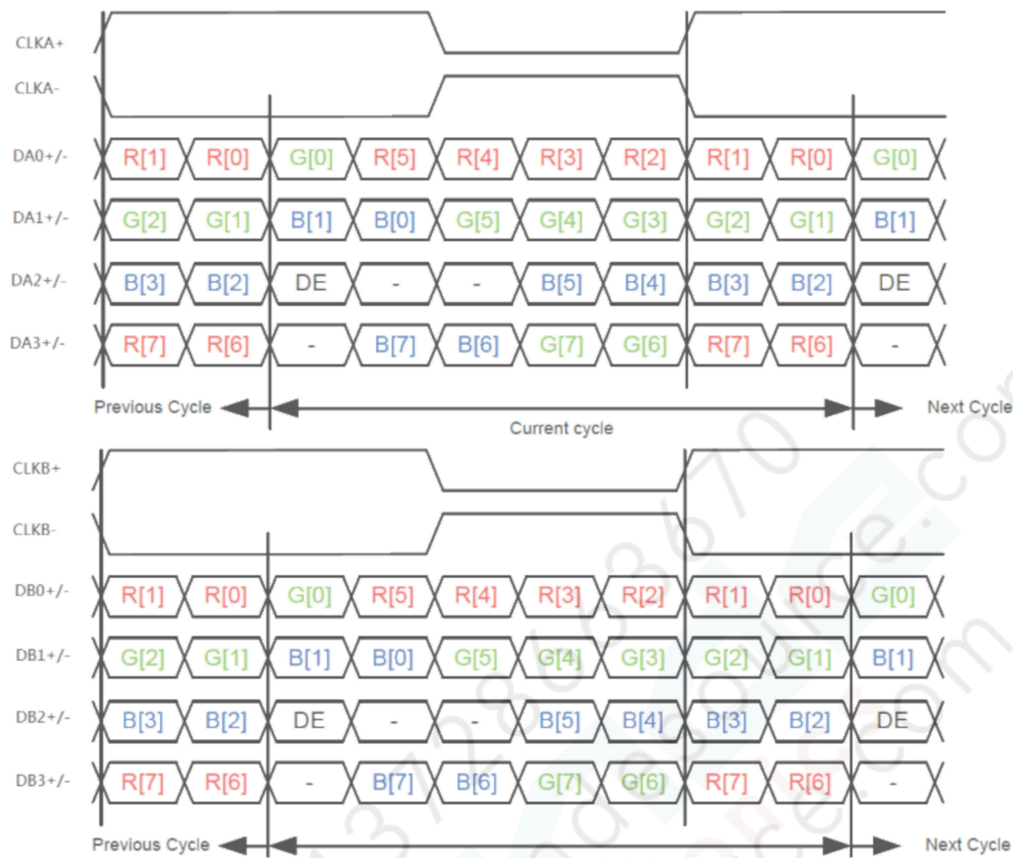
Figure 6.1.3 2-port LVDS signals, VESA format
