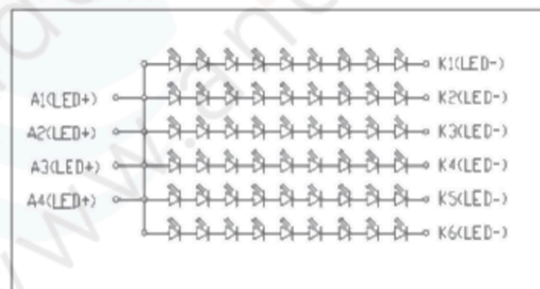
Backlight Circuit Diagram 9S-6P; IF=60mA/LED
