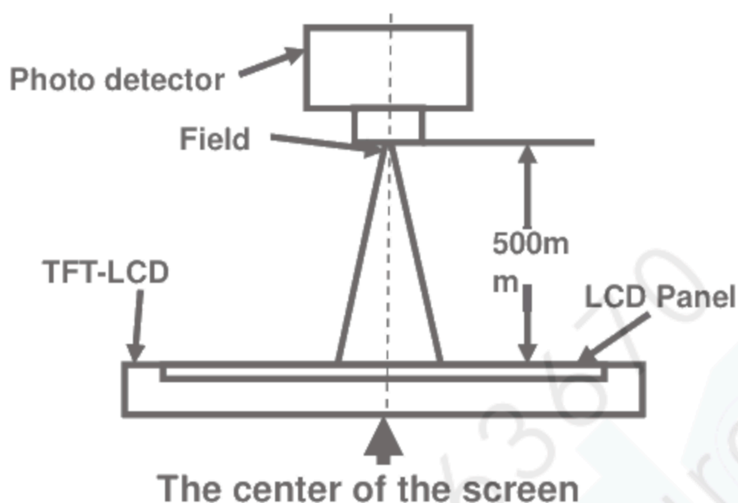
Fig1. Measurement Set Up
