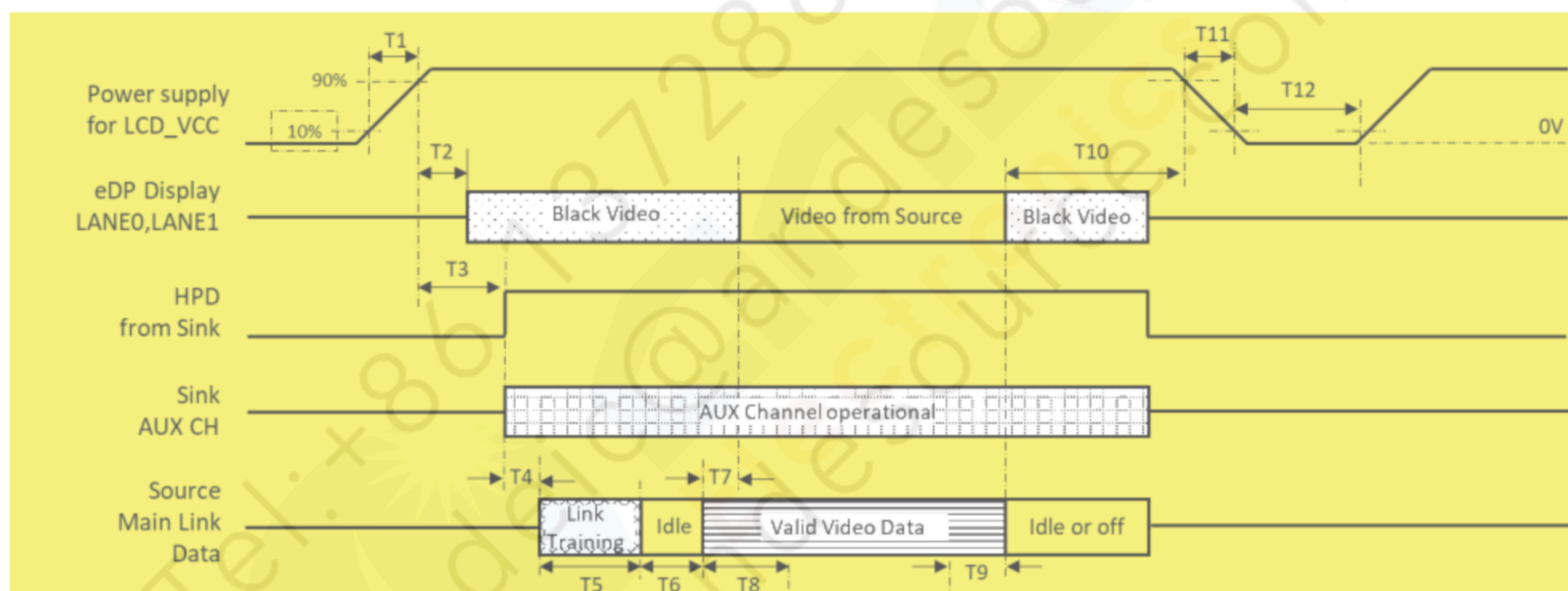
Figure 5.3.1 Power on sequence
