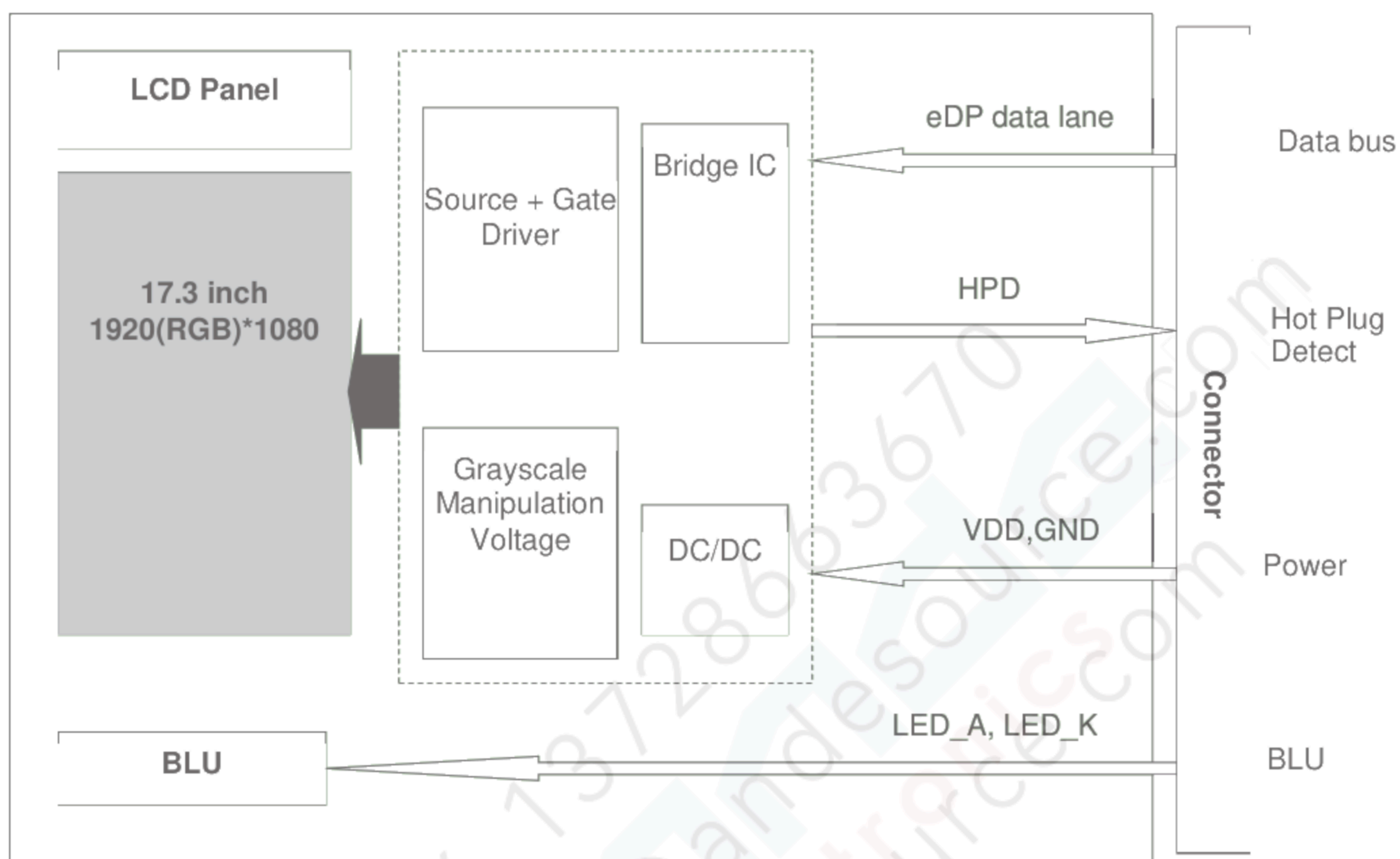
Figure 5.4.1 LCD Module Block Diagram
