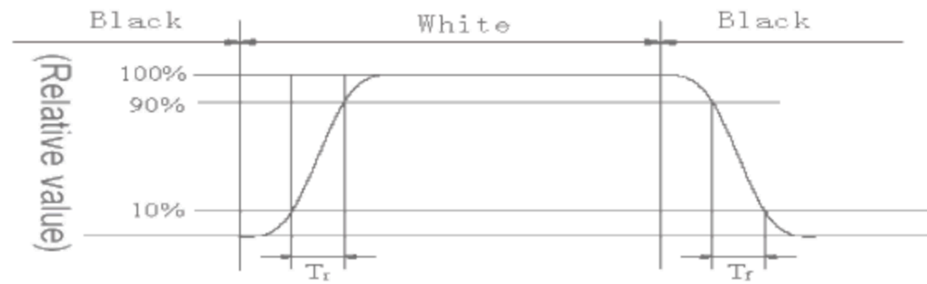
Fig3. Response Time Testing
