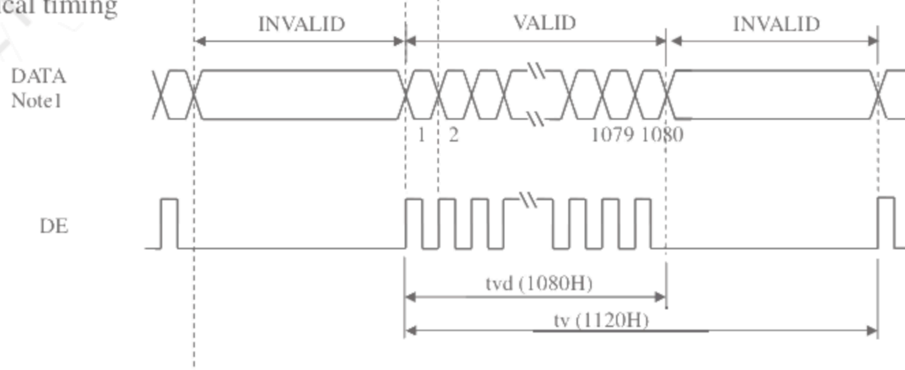
Figure 6.1.1 Input Signal Timings
