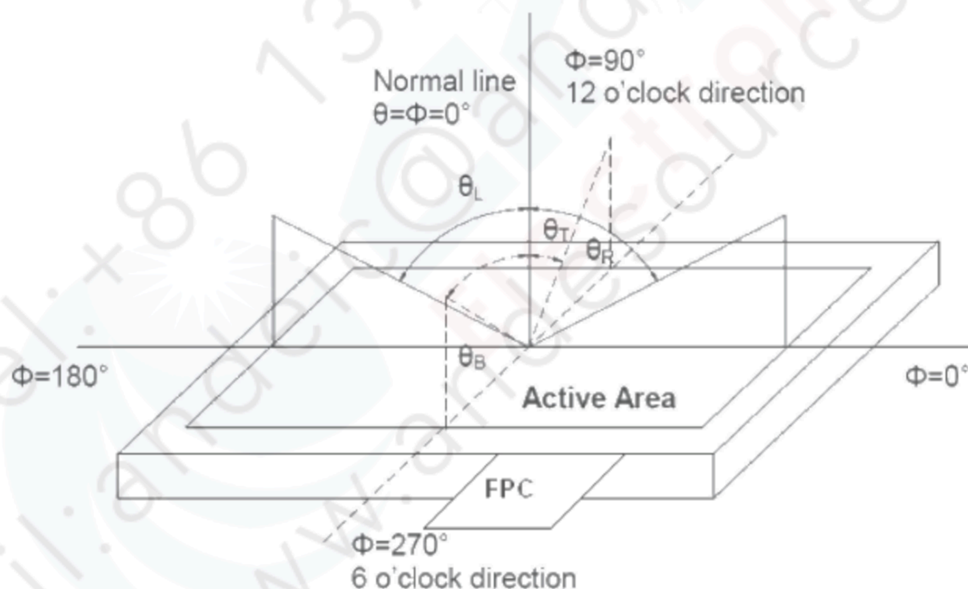
Fig2. Measurement viewing angle
