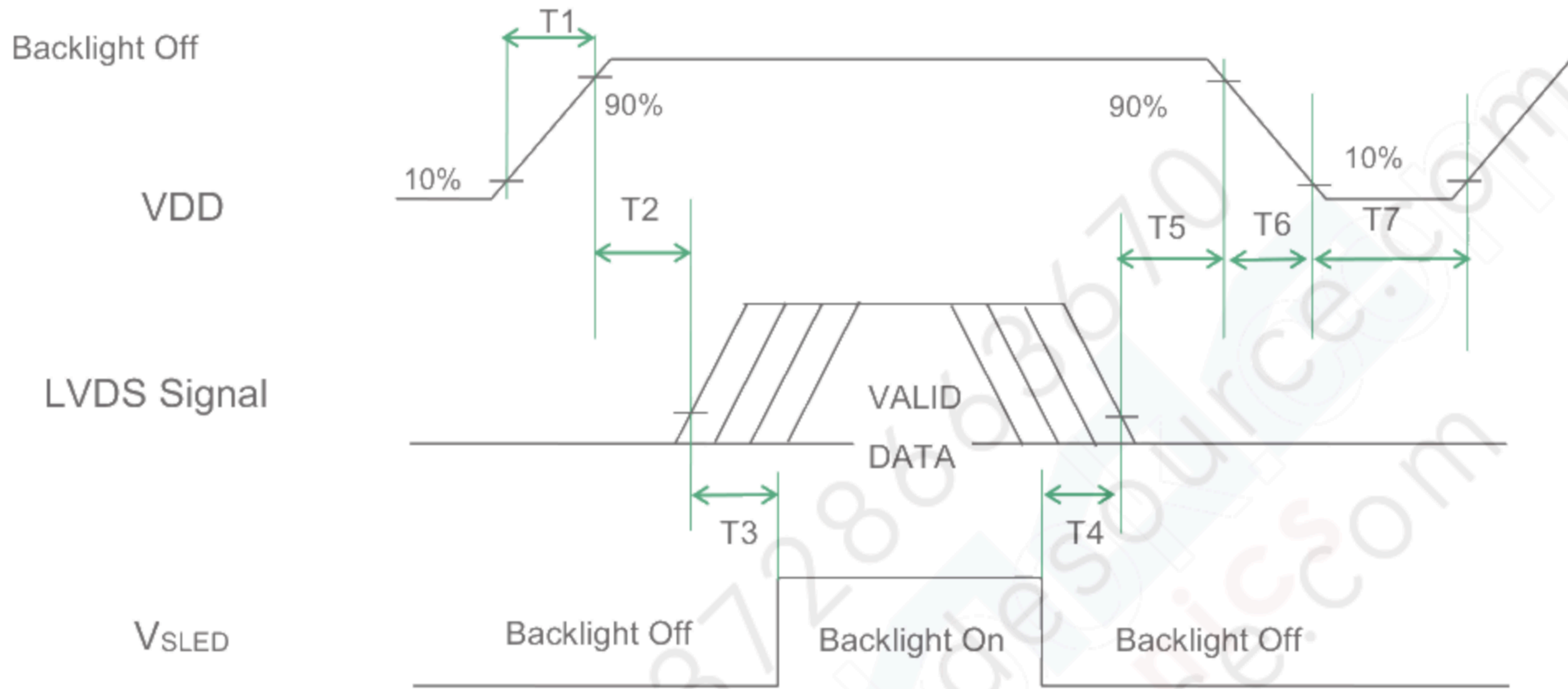
Power Sequence Timing
