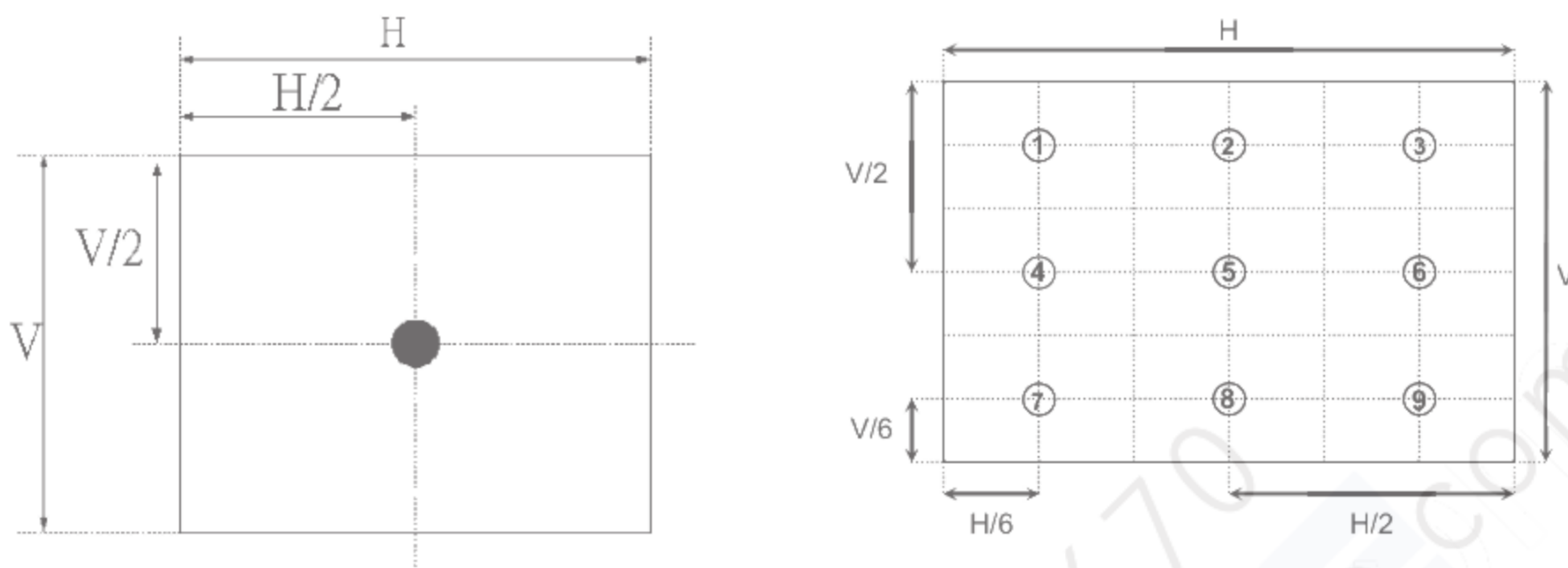
Fig. 3 Luminance
