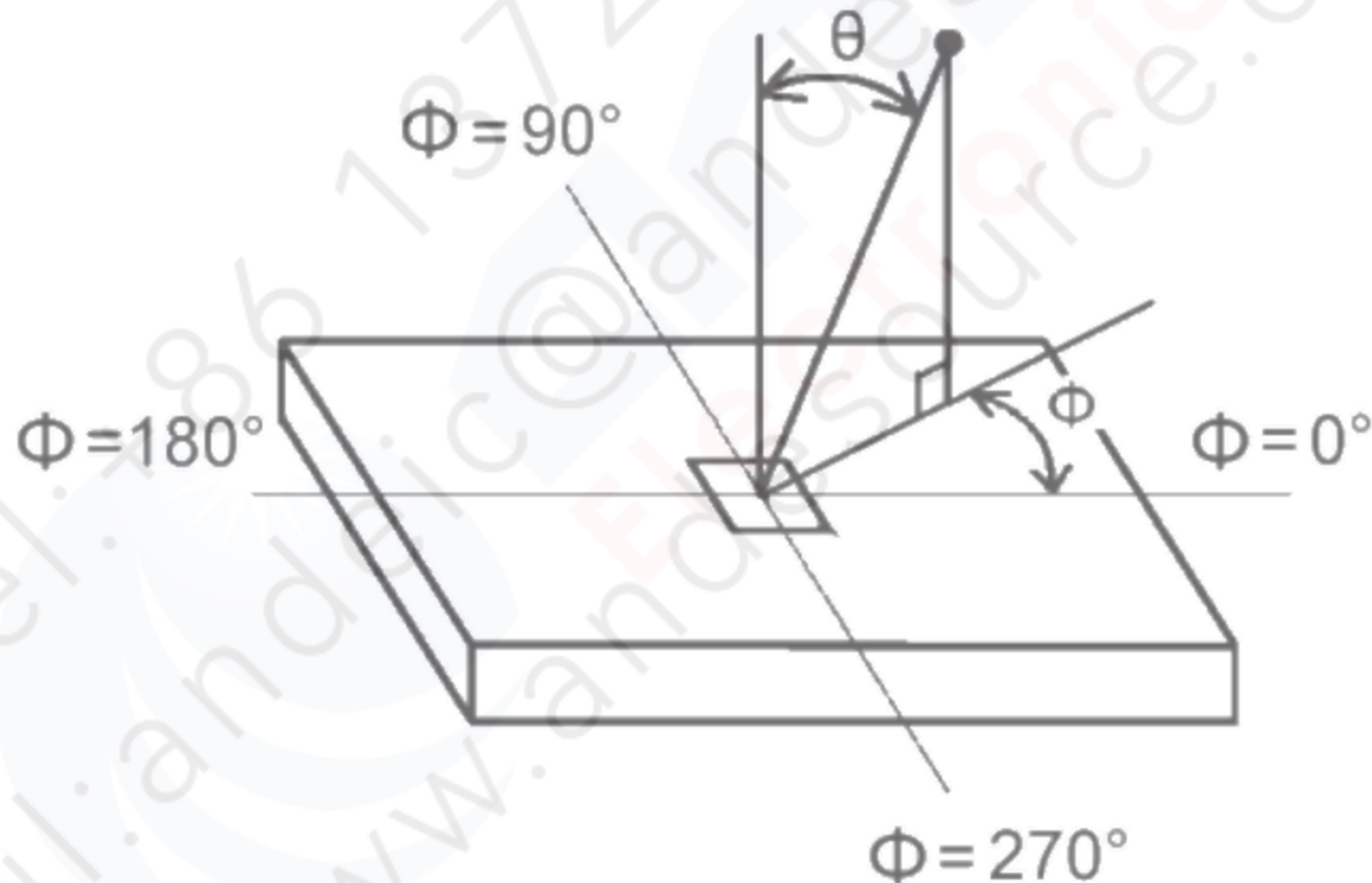
Fig. 4 Viewing Angle
