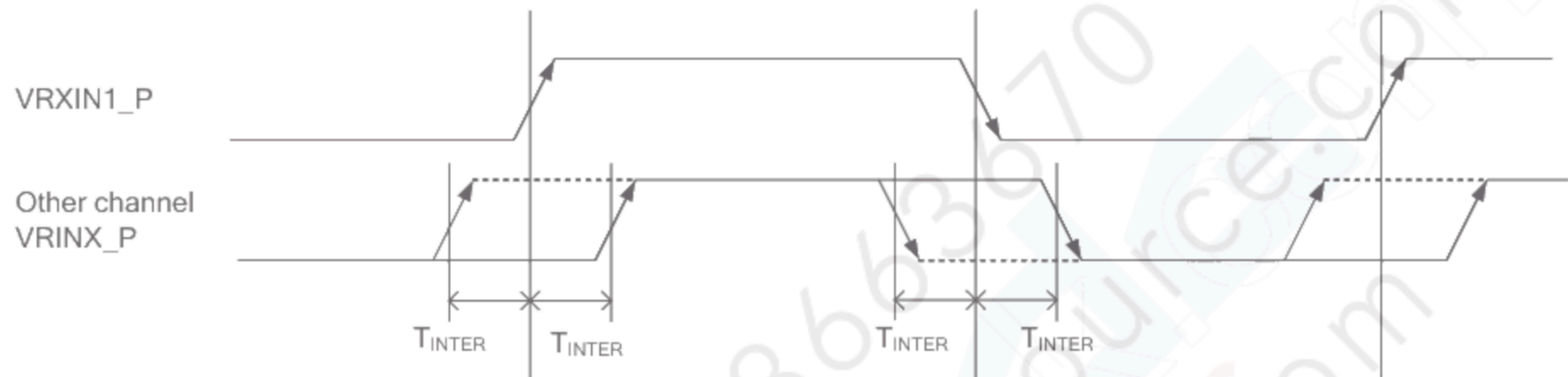
Note8. Eye diagram at receiver
