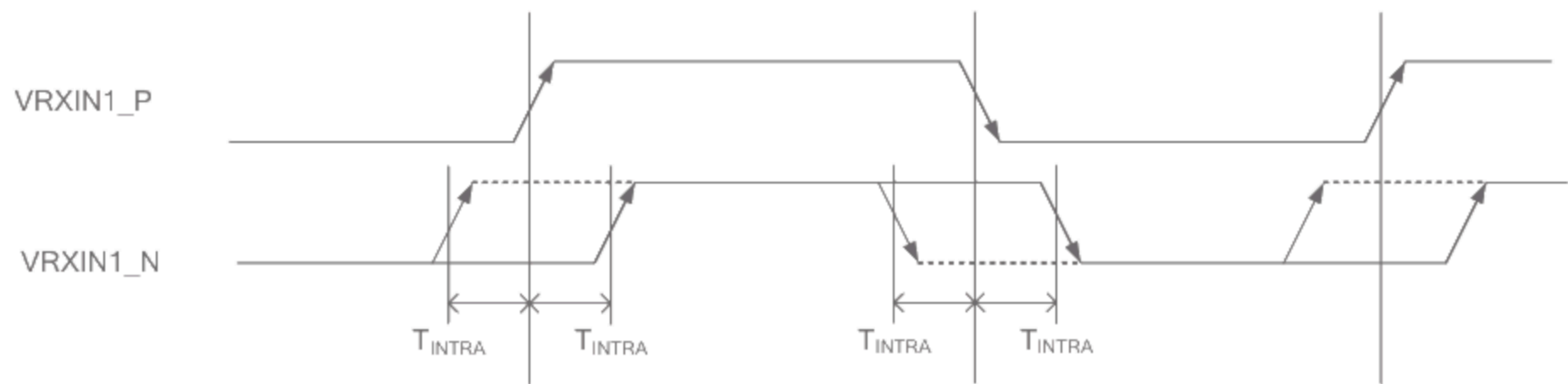
Note7. V-by-one Inter-pair Skew
