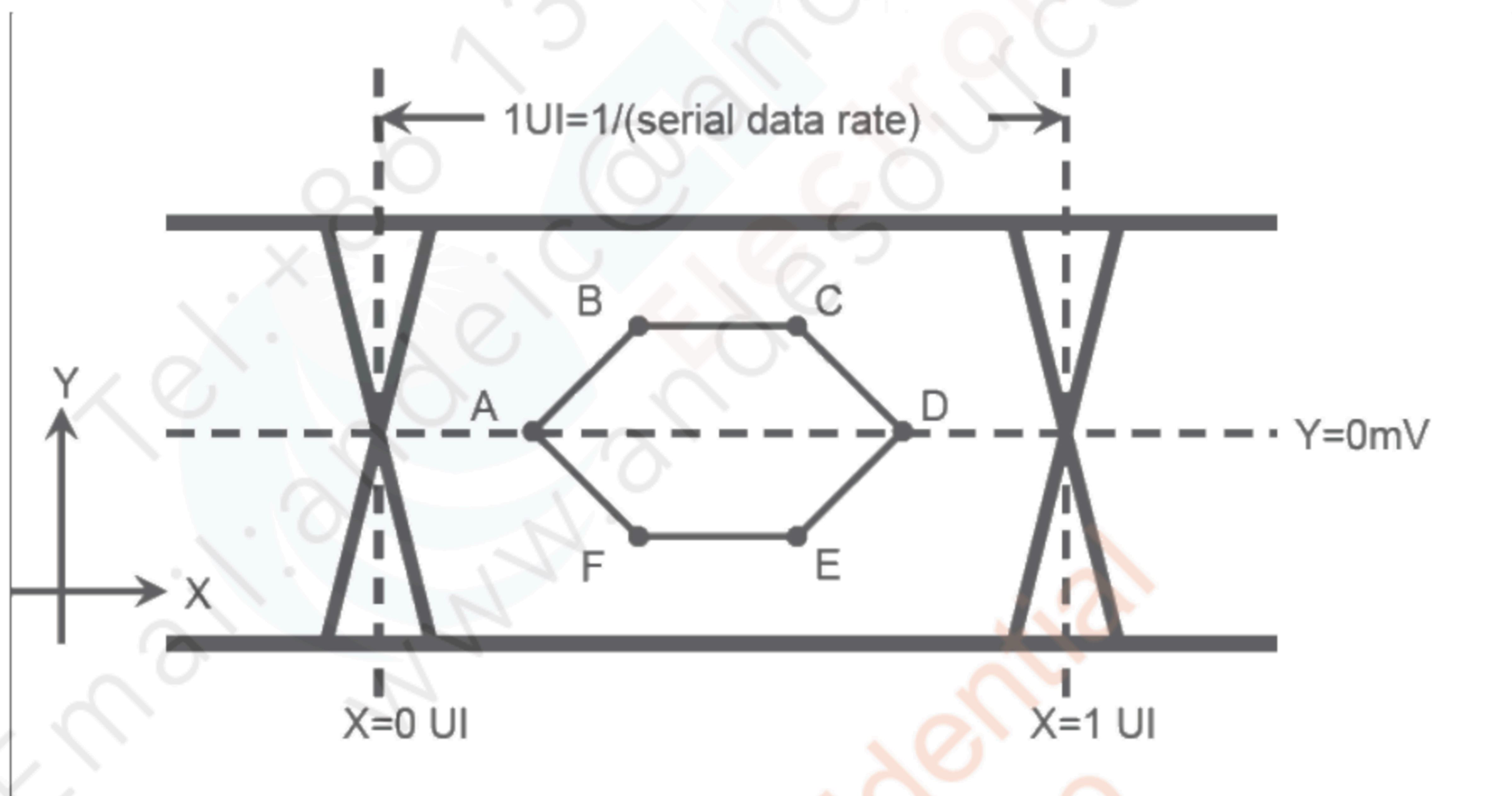
Example of Eye diagram
