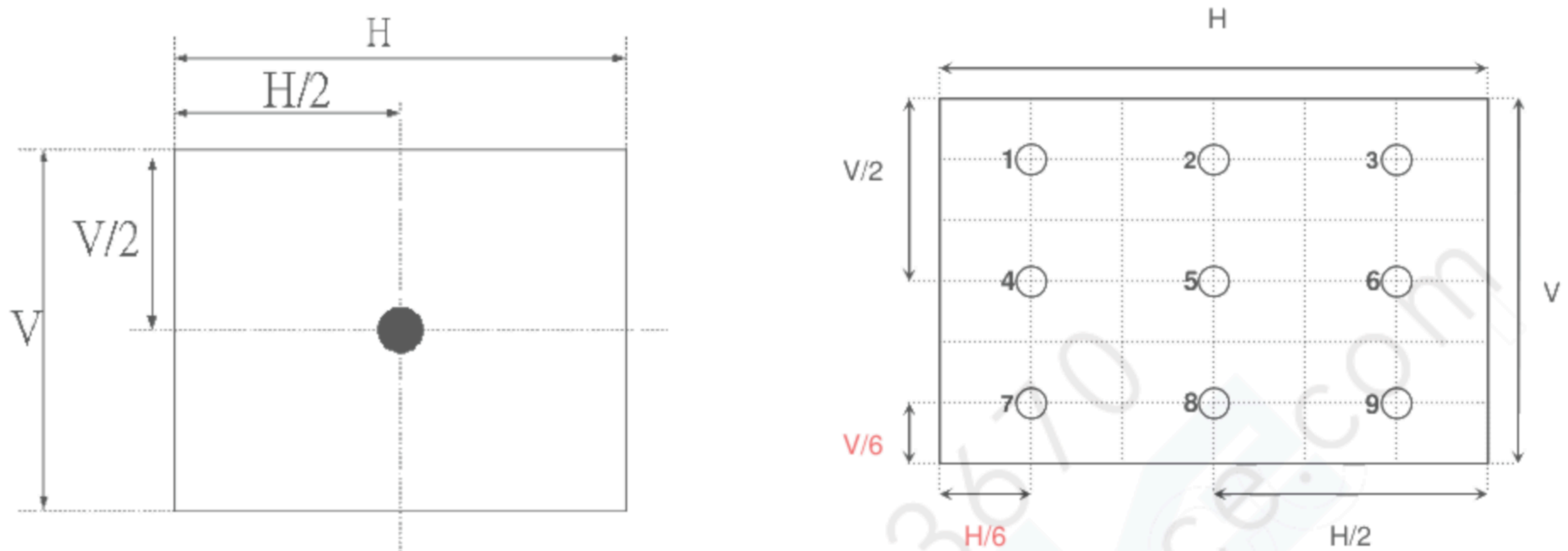
FIG. 2 Luminance
