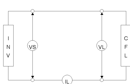
CFL Testing Circuit
