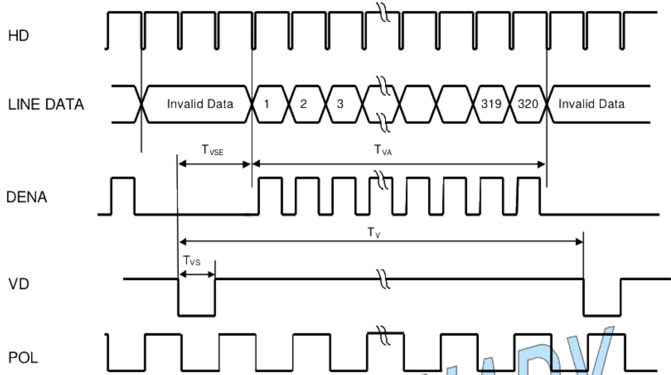
c. Vertical Timing Chart
