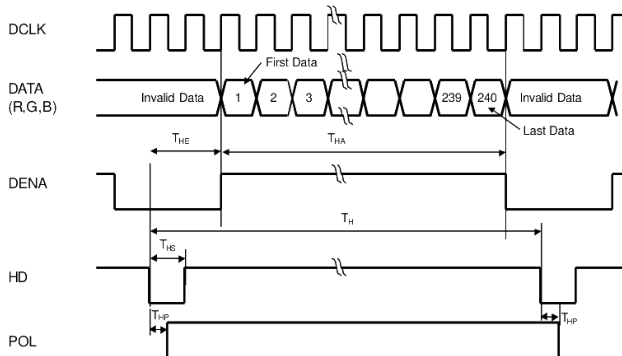
b. Horizontal Timing Chart
