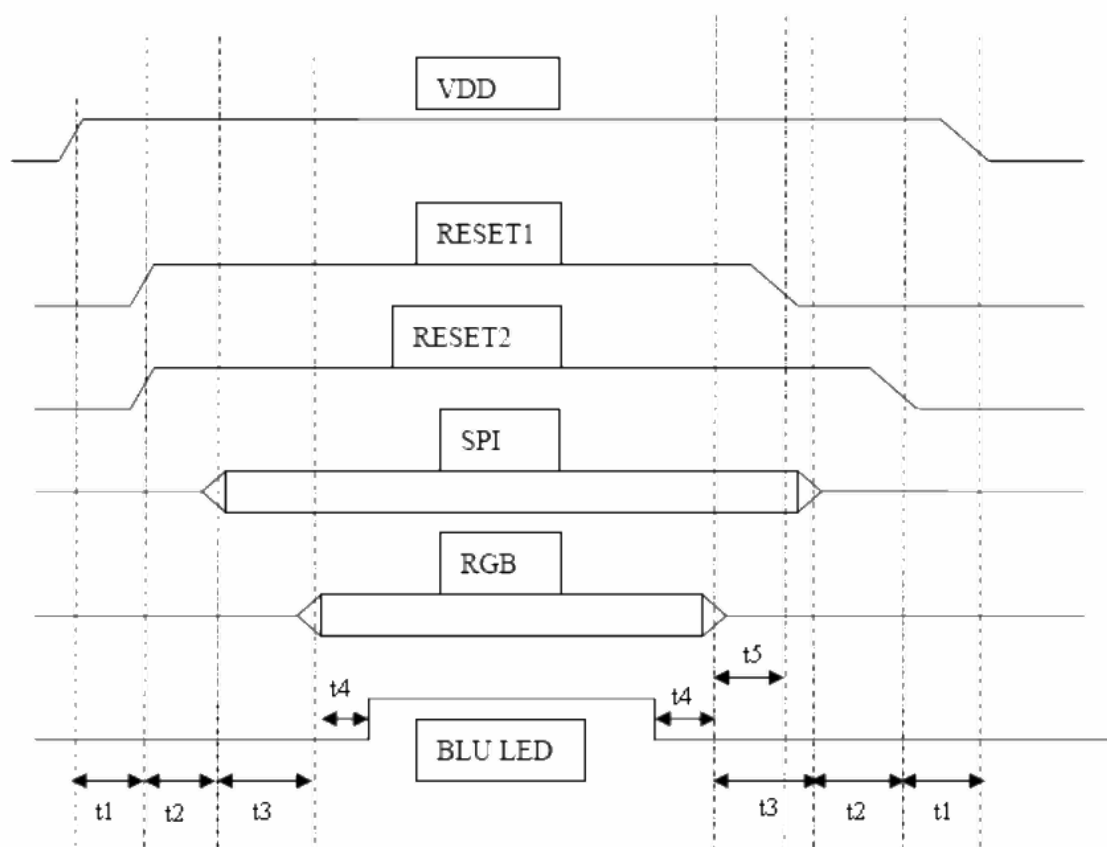
Figure 5.5 Power on/off sequence
