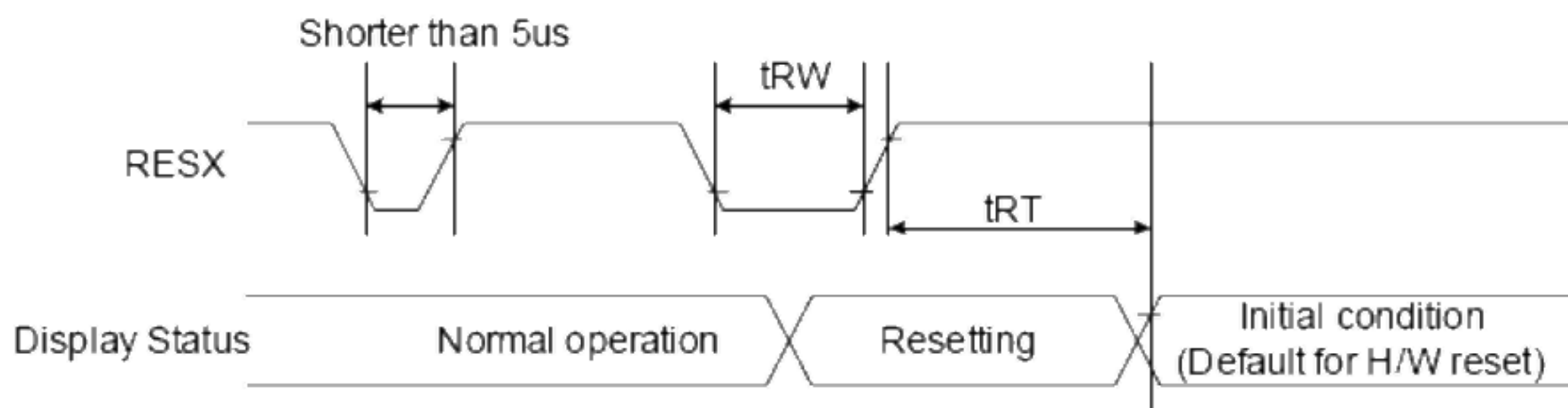
Fig.5-8 Reset timing
