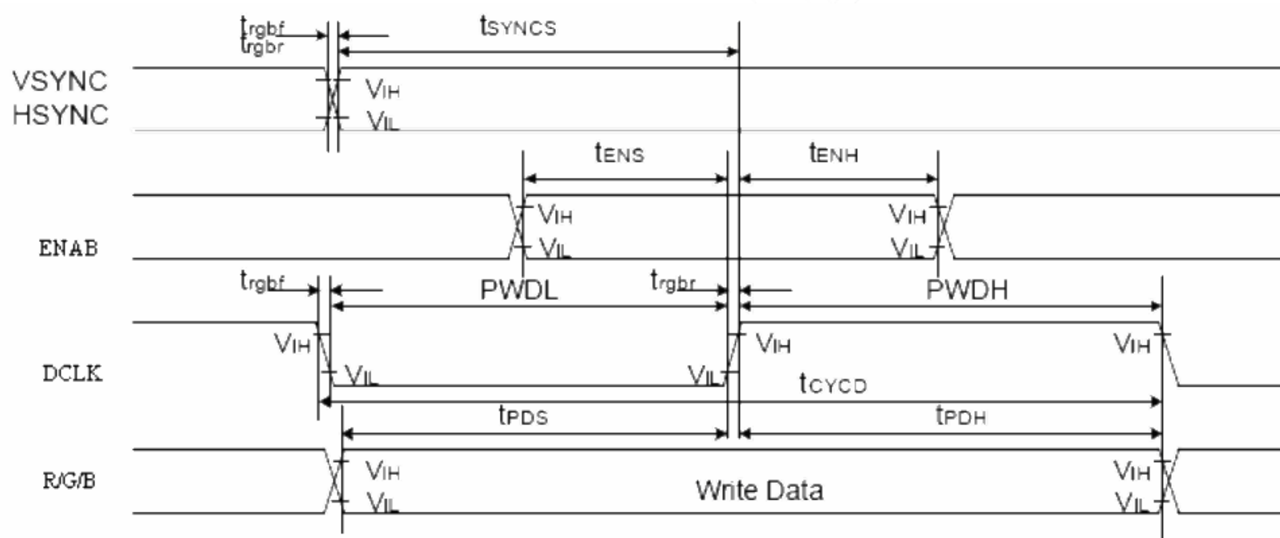
Fig.5-1 RGB Interface Timing
