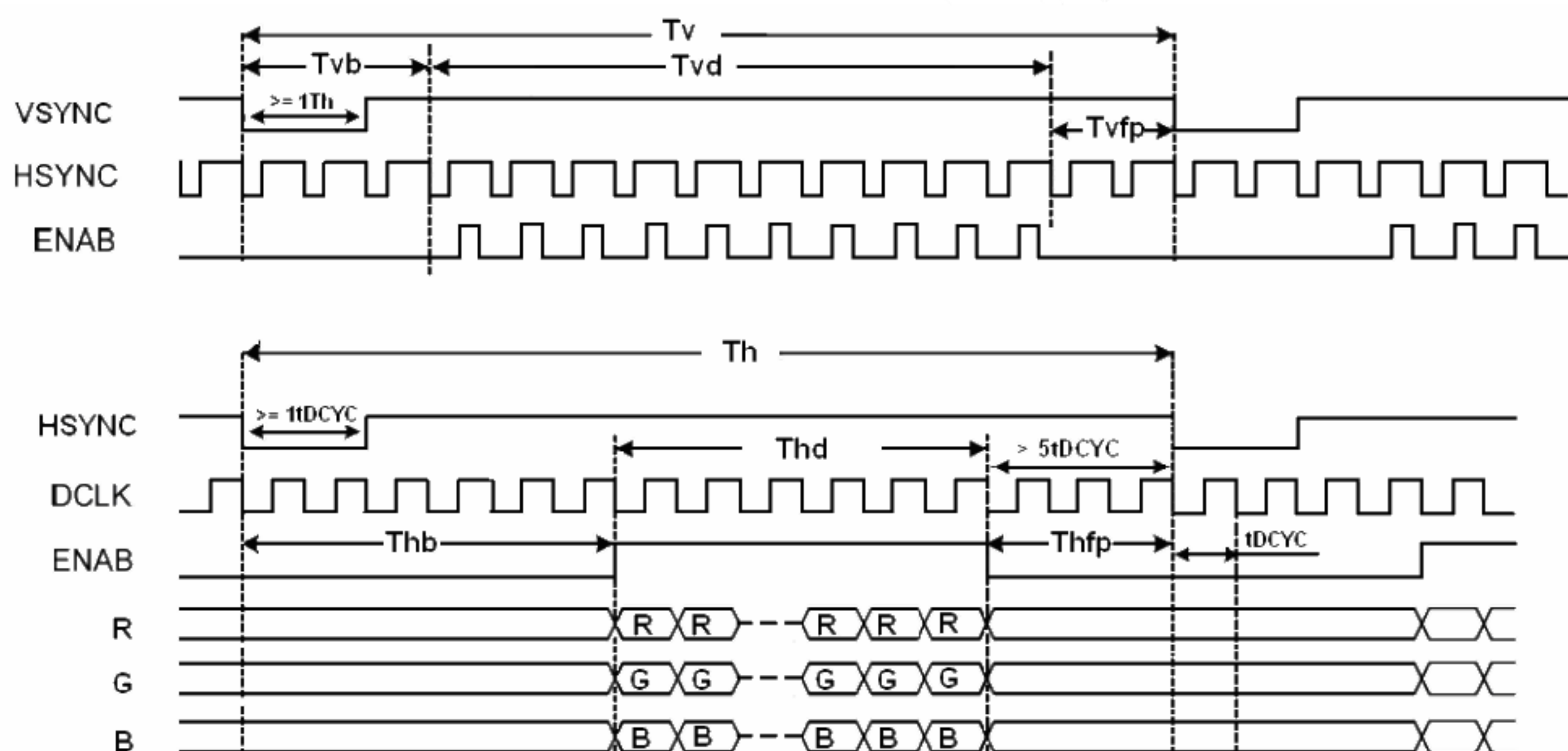
Fig.5-3 Recommend RGB Interface Timing
