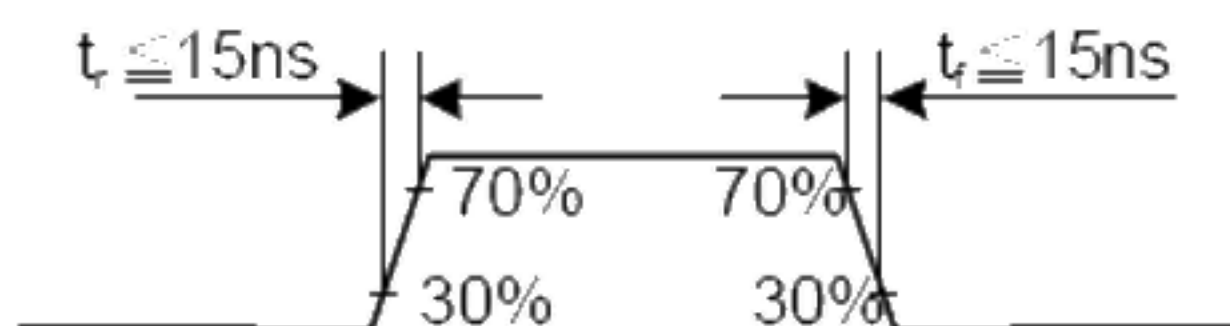
Fig.5-2 Input signal's rise and fall times
