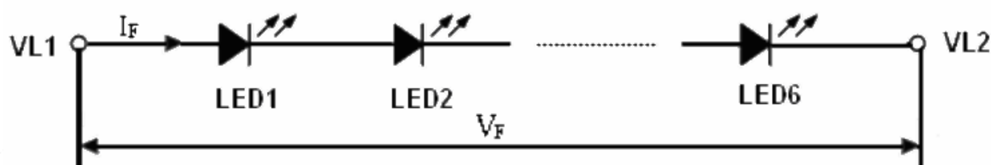
Figure 4.2 LED connection of backlight
