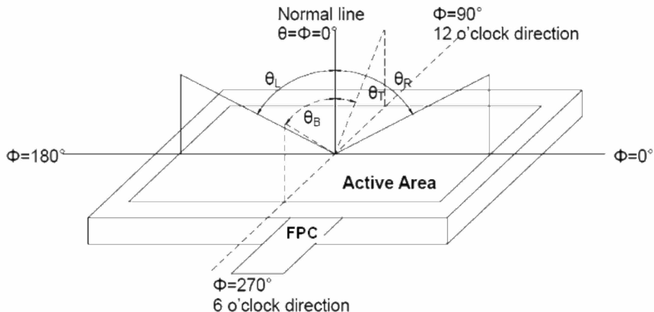
Fig. 1 Definition of viewing angle
