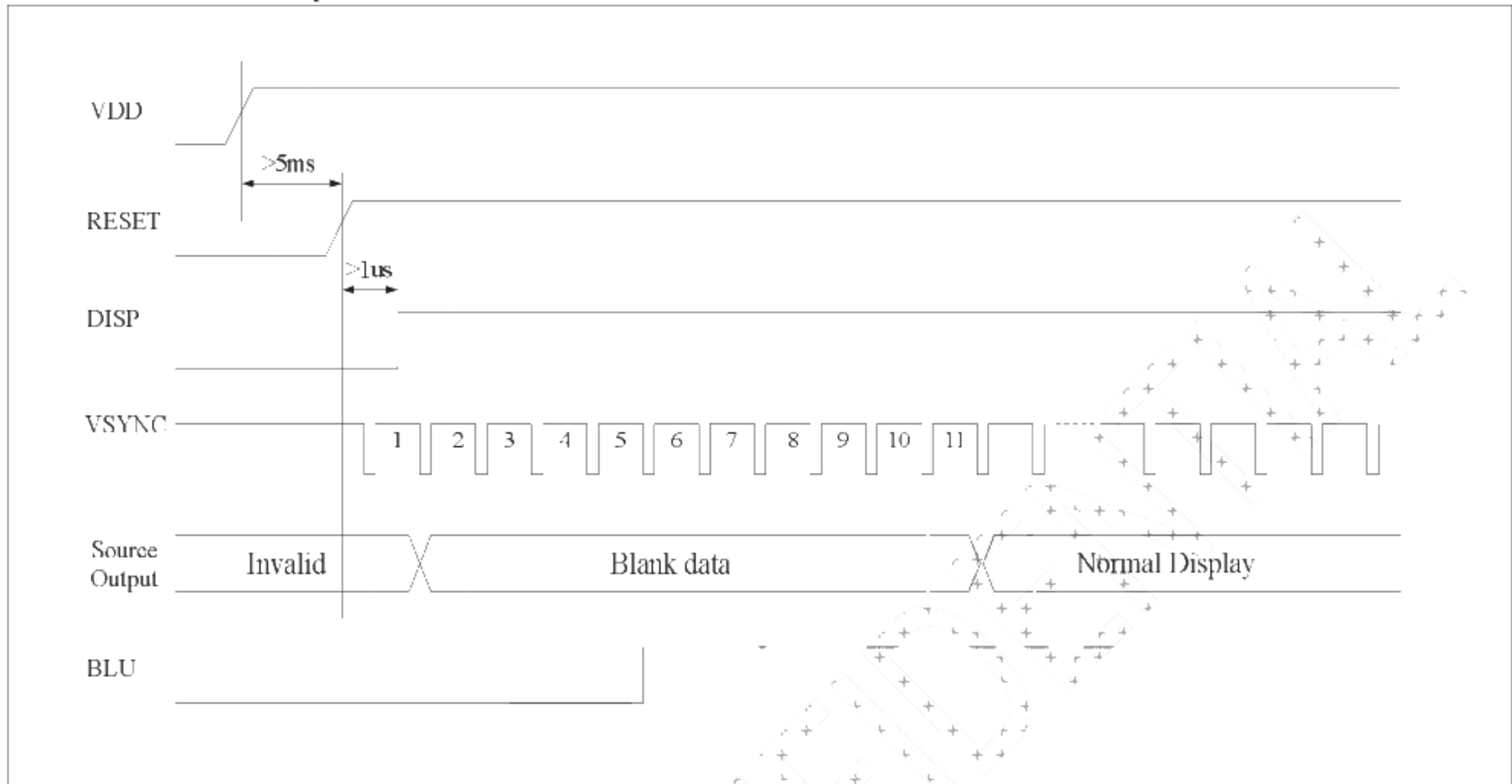
Figure 5.3.1 Power on sequence
