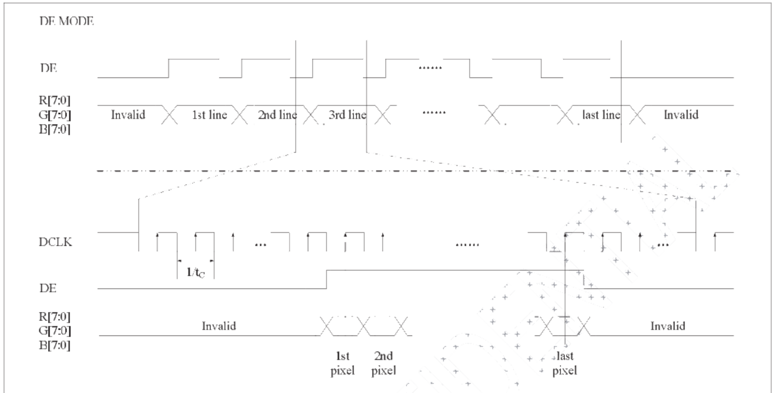
Figure 5.2.2 Data Input Timing Diagram Under DE Mode(VSYNC/HSYNC="H")
