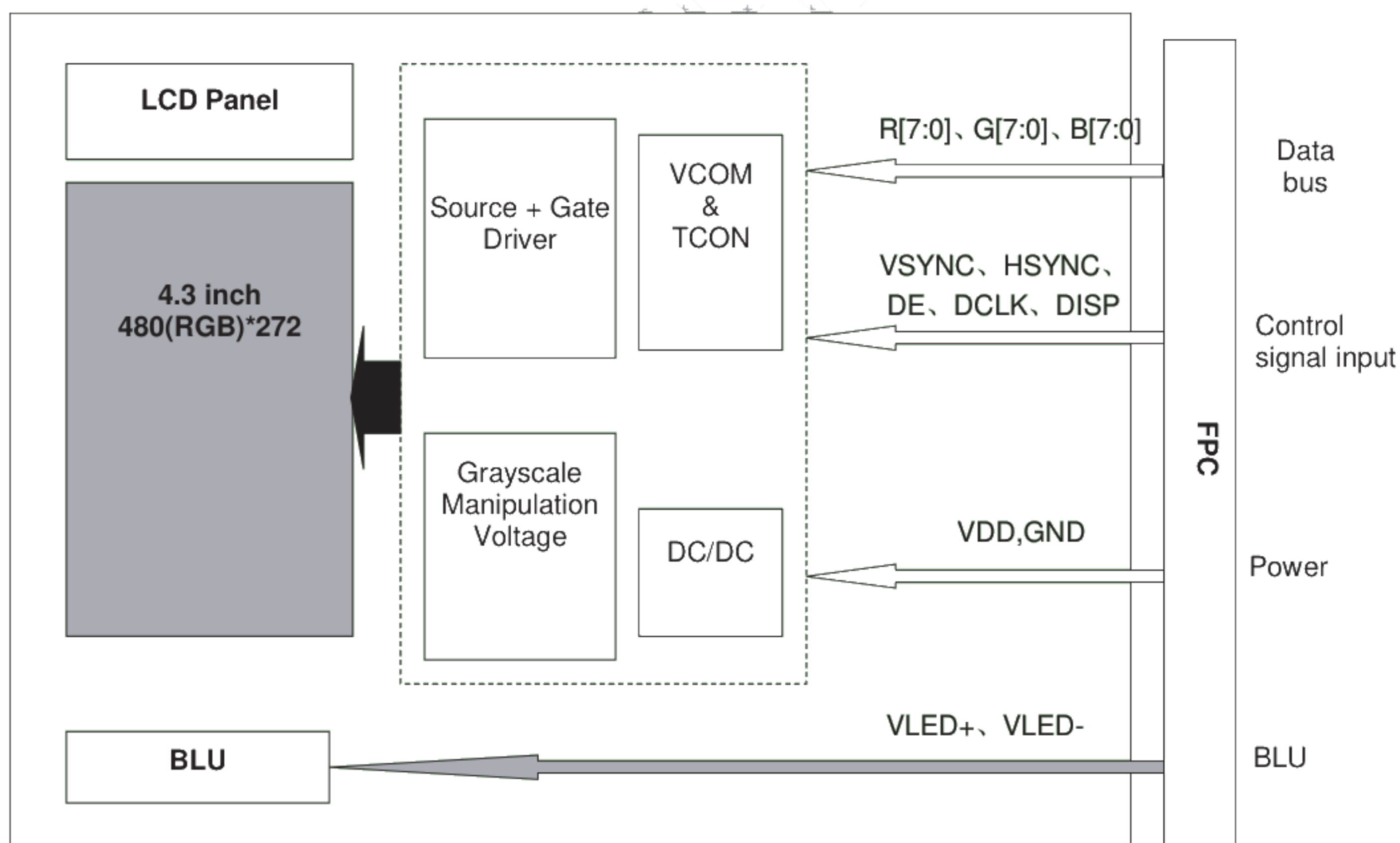
Figure 4.3 LCD Module Diagram
