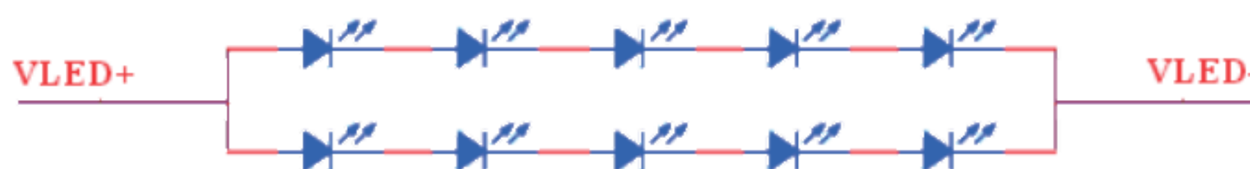
Figure 4.2 LED connection of backlight
