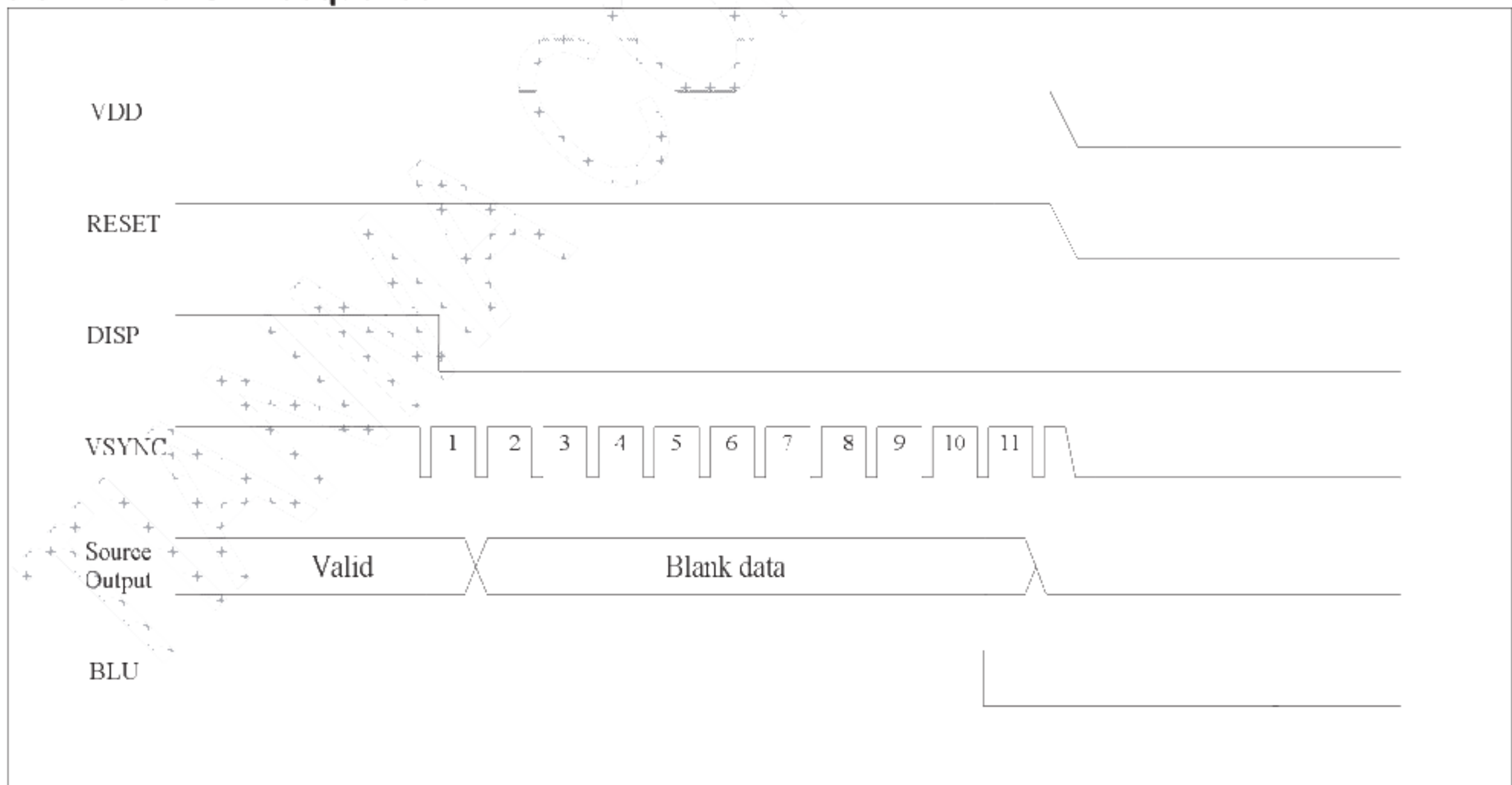
Figure 5.3.2 Power off sequence
