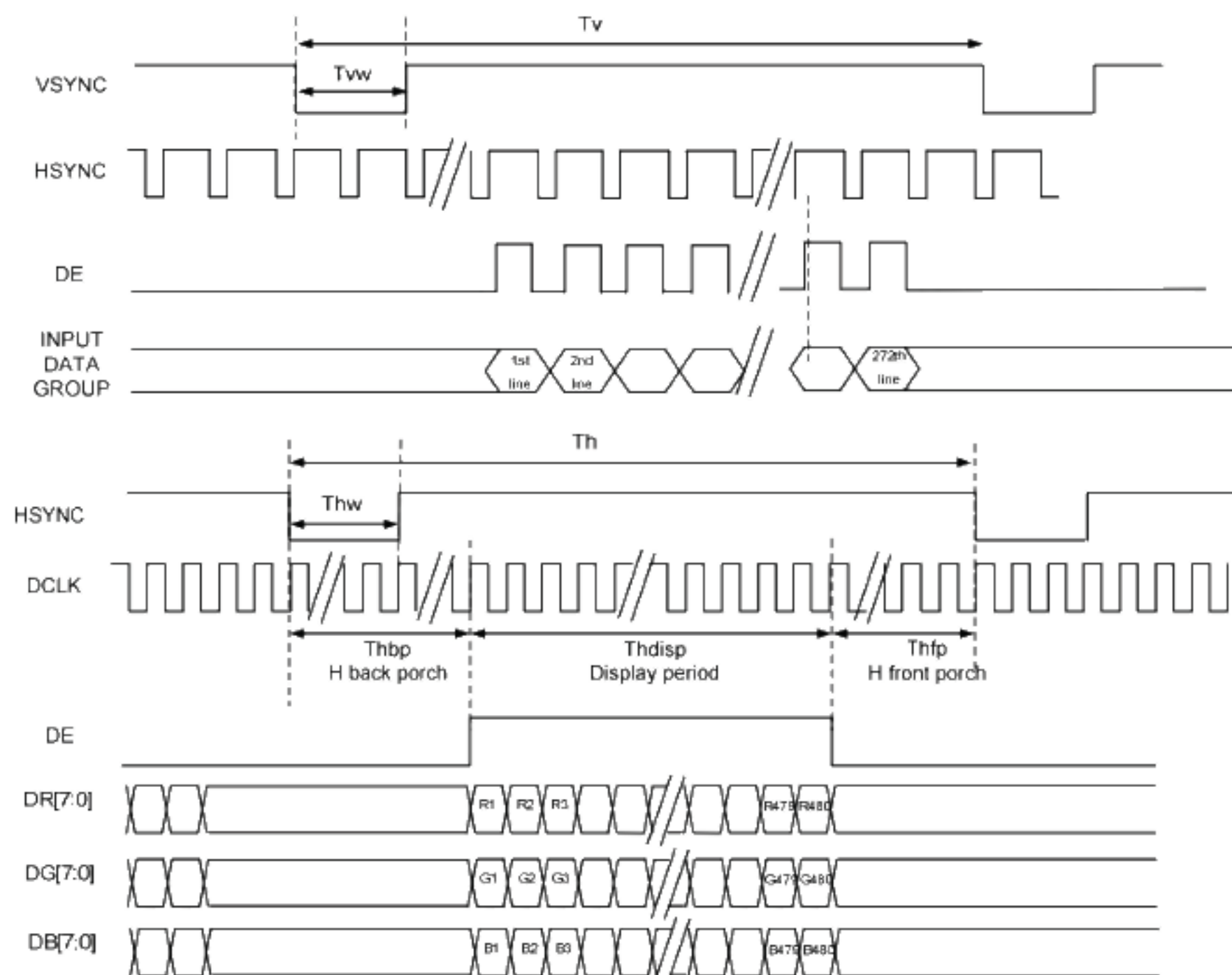
Figure 5.4.2 SYNC-DE Mode Timing Diagram
