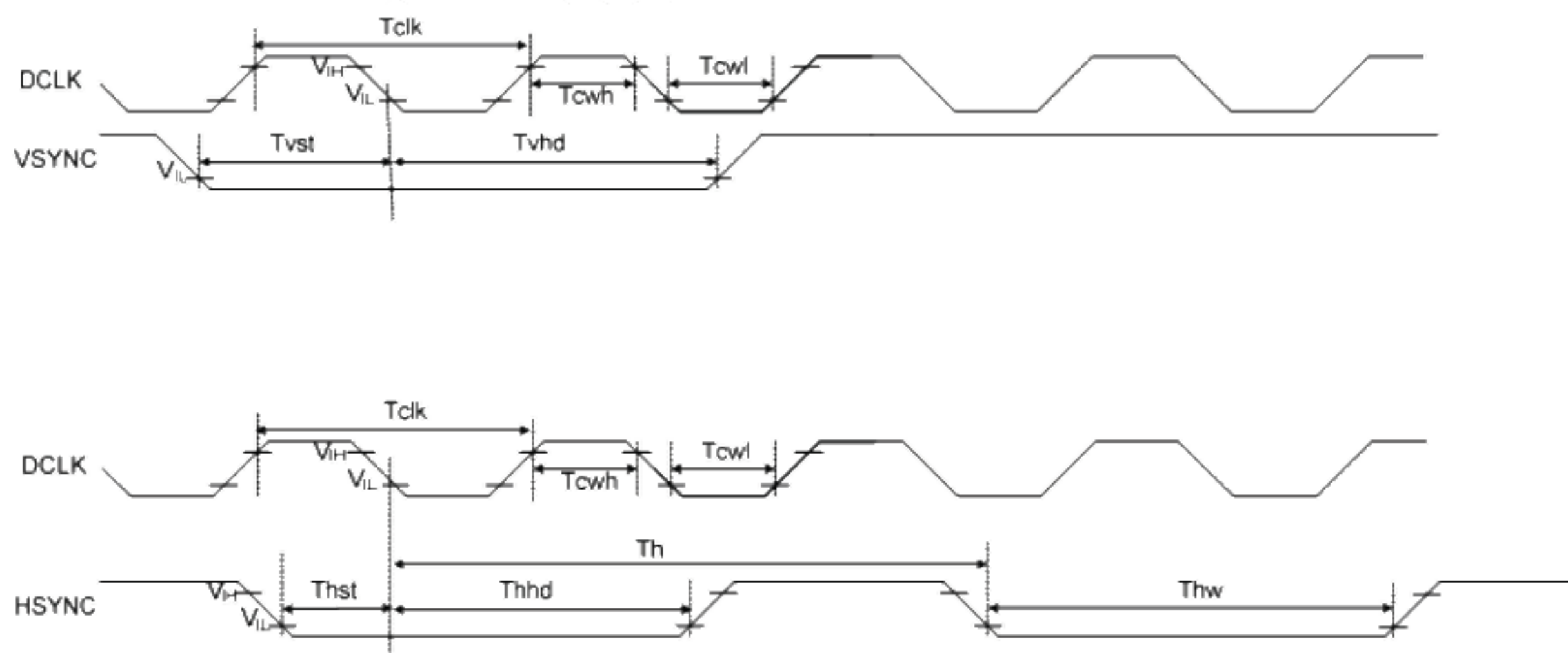
Figure 5.2.1 Clock and Data Input Timing Diagram
