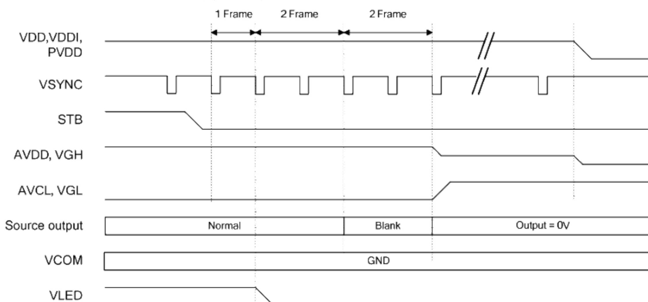
Figure 5.5.2 Power off Sequence
