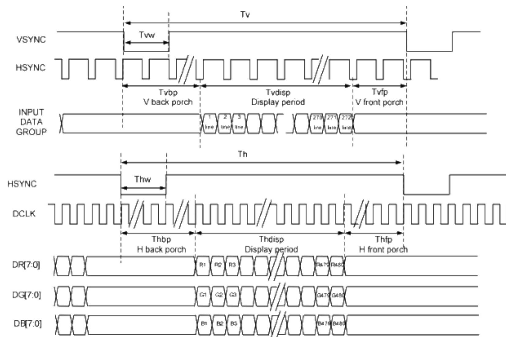
Figure 5.4.1 SYNC Mode Timing Diagram
