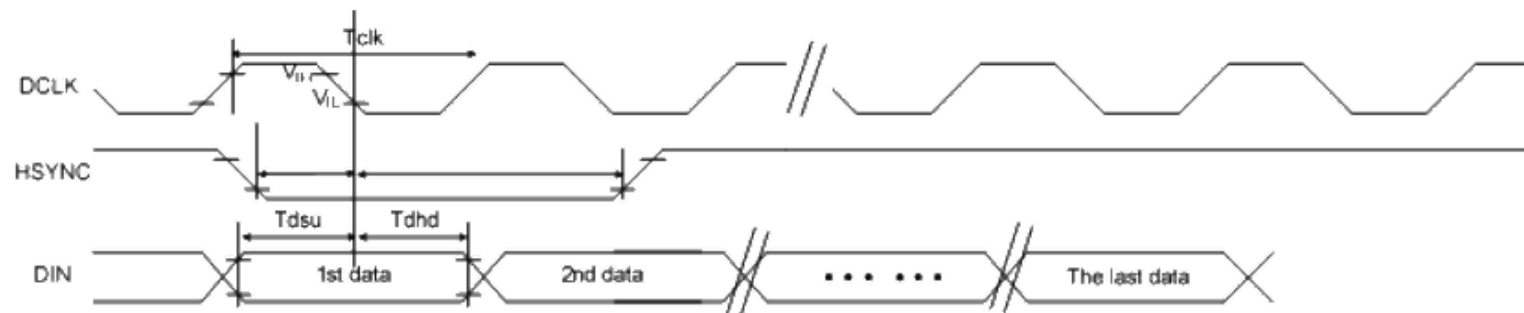
Figure 5.2.1.1 SYNC Mode
