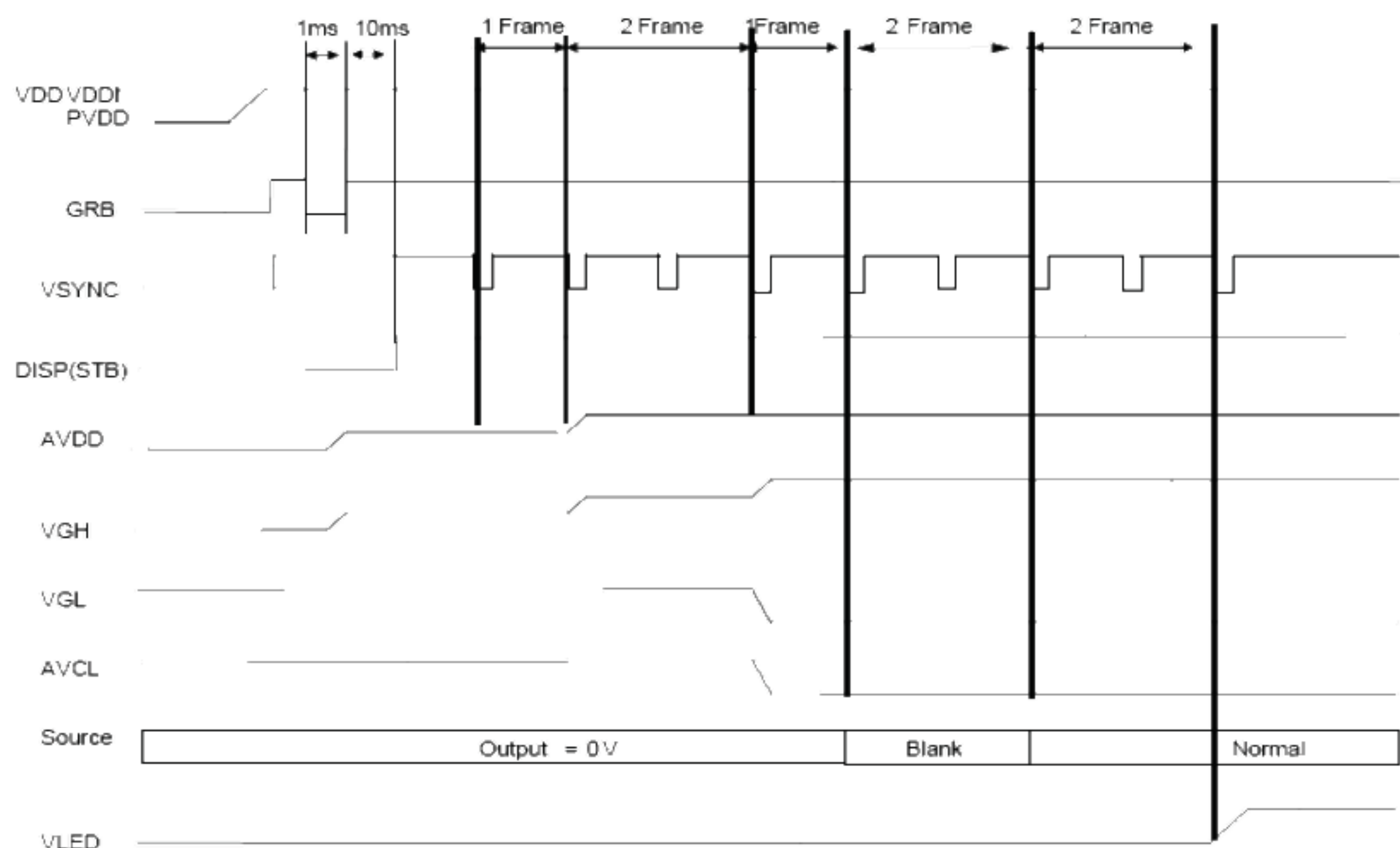
Figure 5.5.1 Power on Sequence
