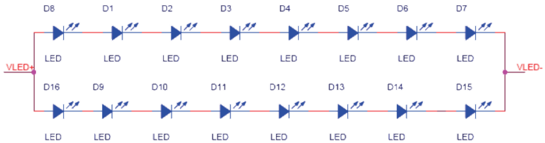
Figure 4.2.1 LED Driver Circuit
