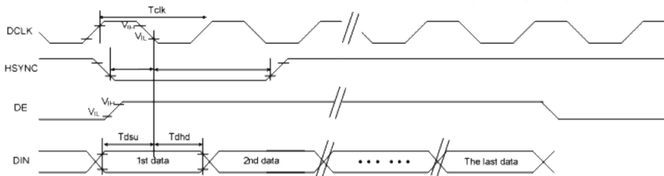
Figure 5.2.1.2 SYNC-DE Mode
