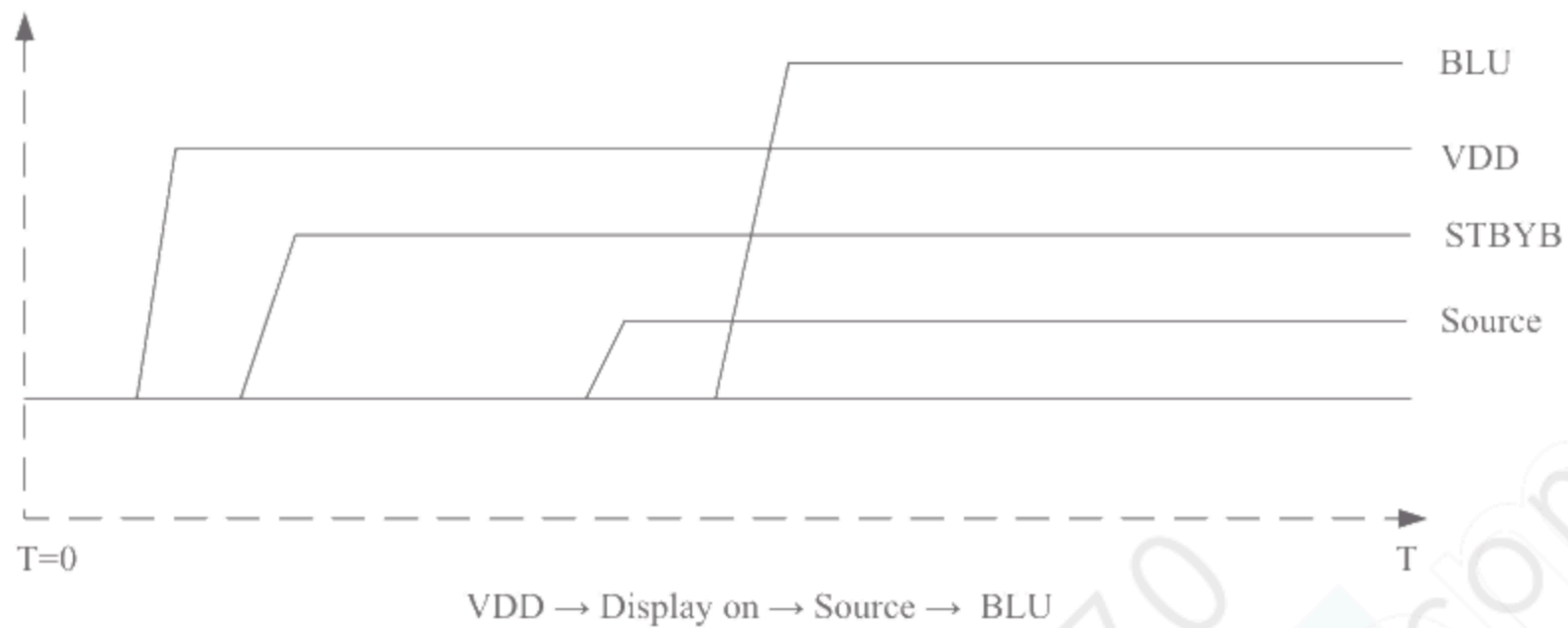
Figure 5.3.2 Power On Sequence
