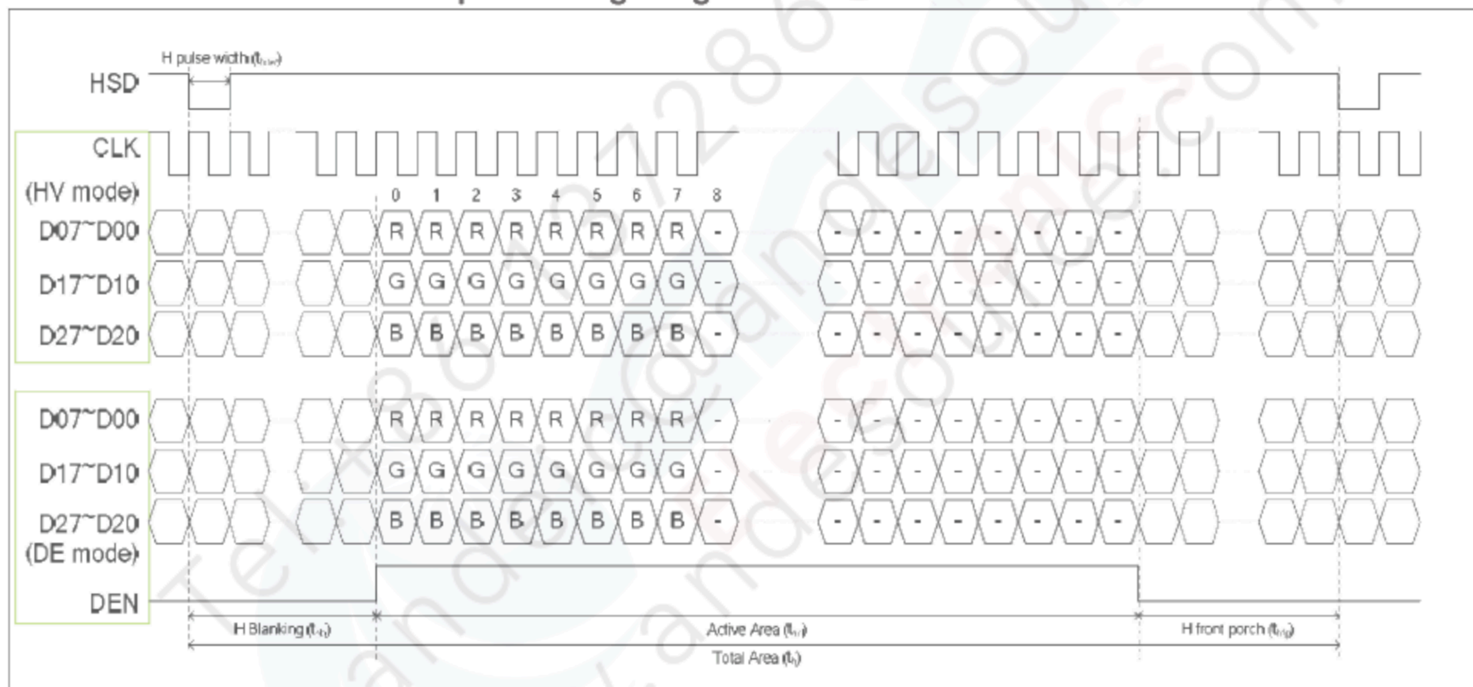
Figure 5.2 Horizontal Input Timing Diagram
