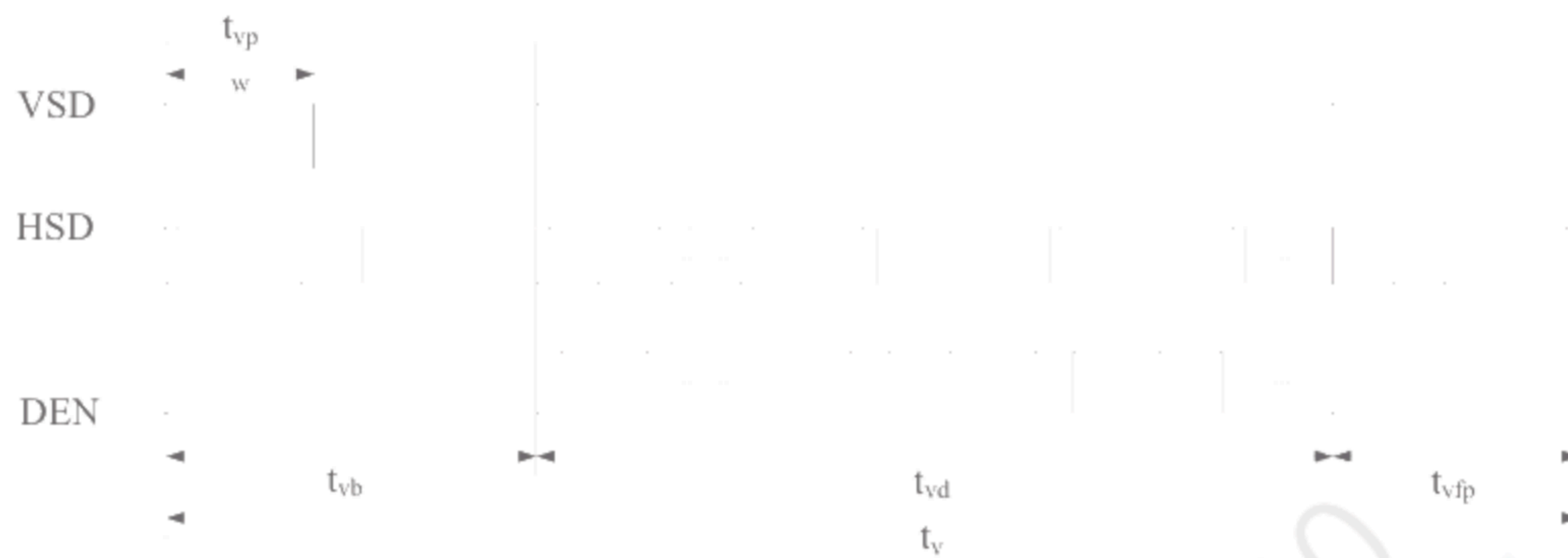
Figure 5.2.3 Vertical Input Timing Diagram
