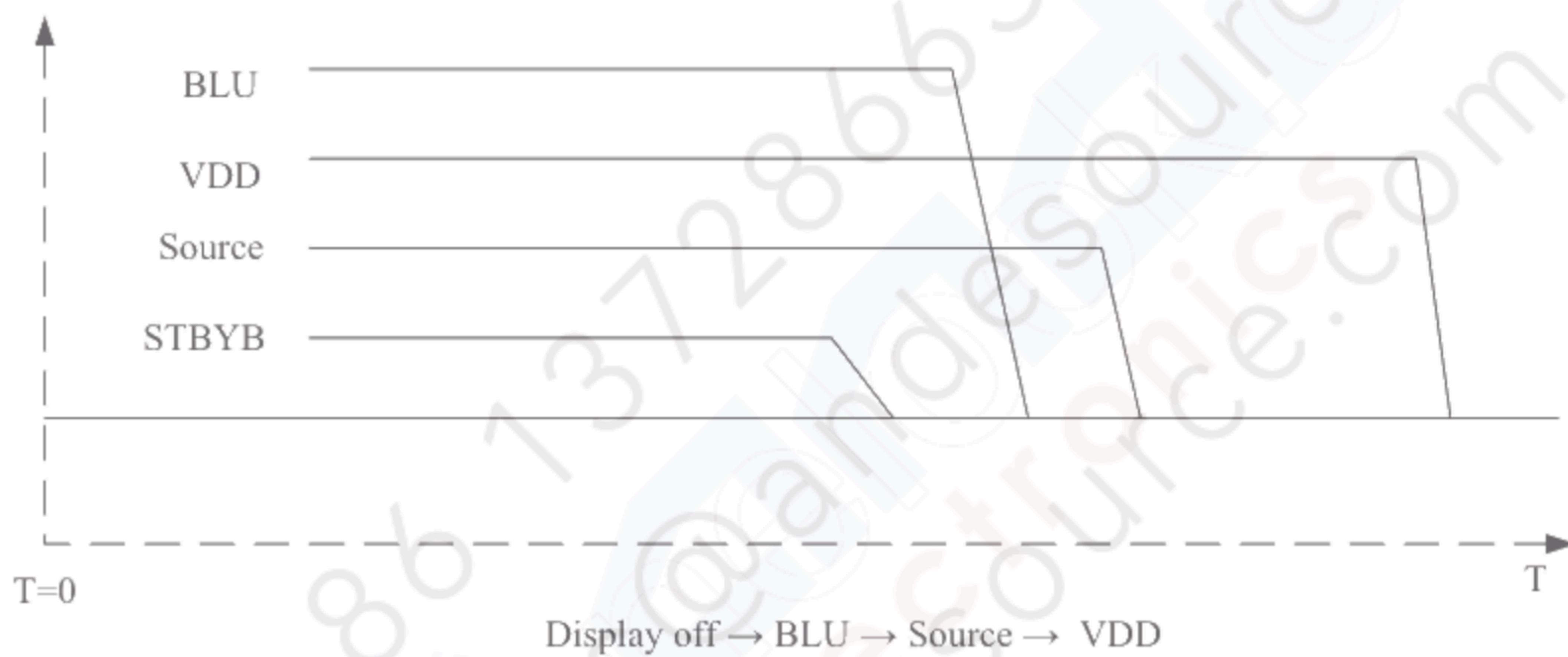
Figure 5.3.3 Power Off Sequence
